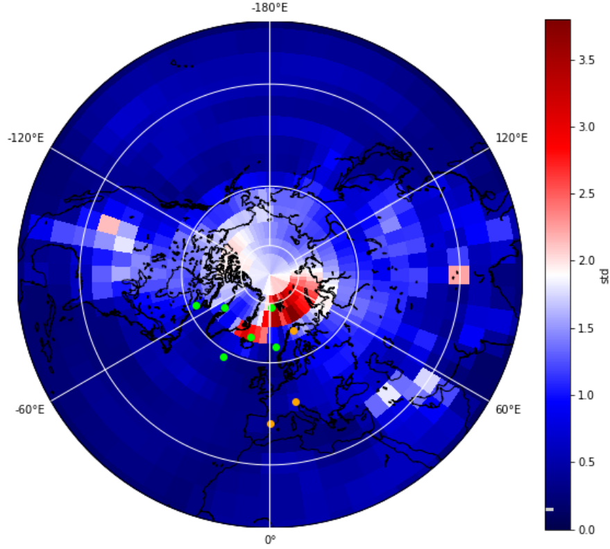
Figure 6: Illustration of the atmospheric yearly temperature standard deviation
