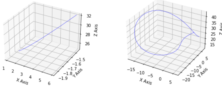
Figure 2.2: Lorenz63 trajectory visualisation 10dt and 100dt
