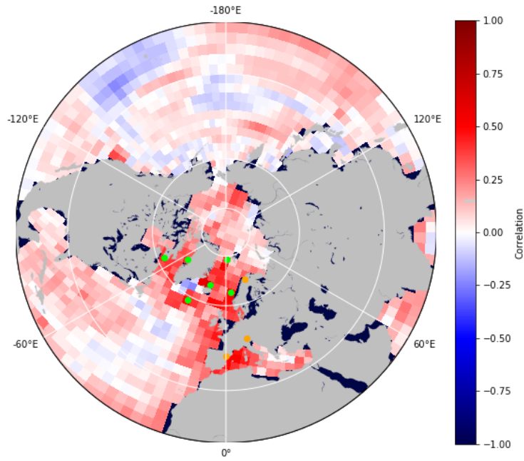
Figure 8: Illustration of yearly Correlation Coefficients on SST, base with interpolation
