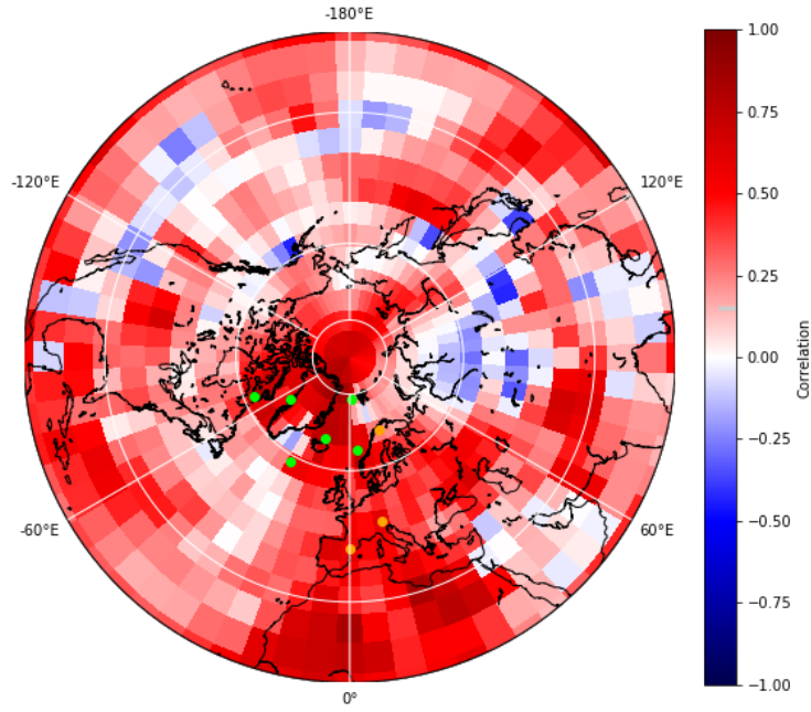
Figure 11: Illustration of decadal Correlation Coefficients on TS, base with interpolation
