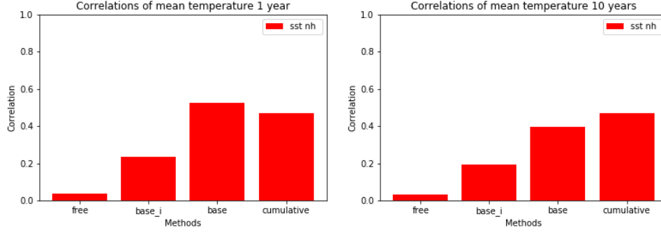
Figure 3.13: Correlation coefficients over average temperature on SST in the northern hemisphere, 1 year (left) and 10 years (right)
