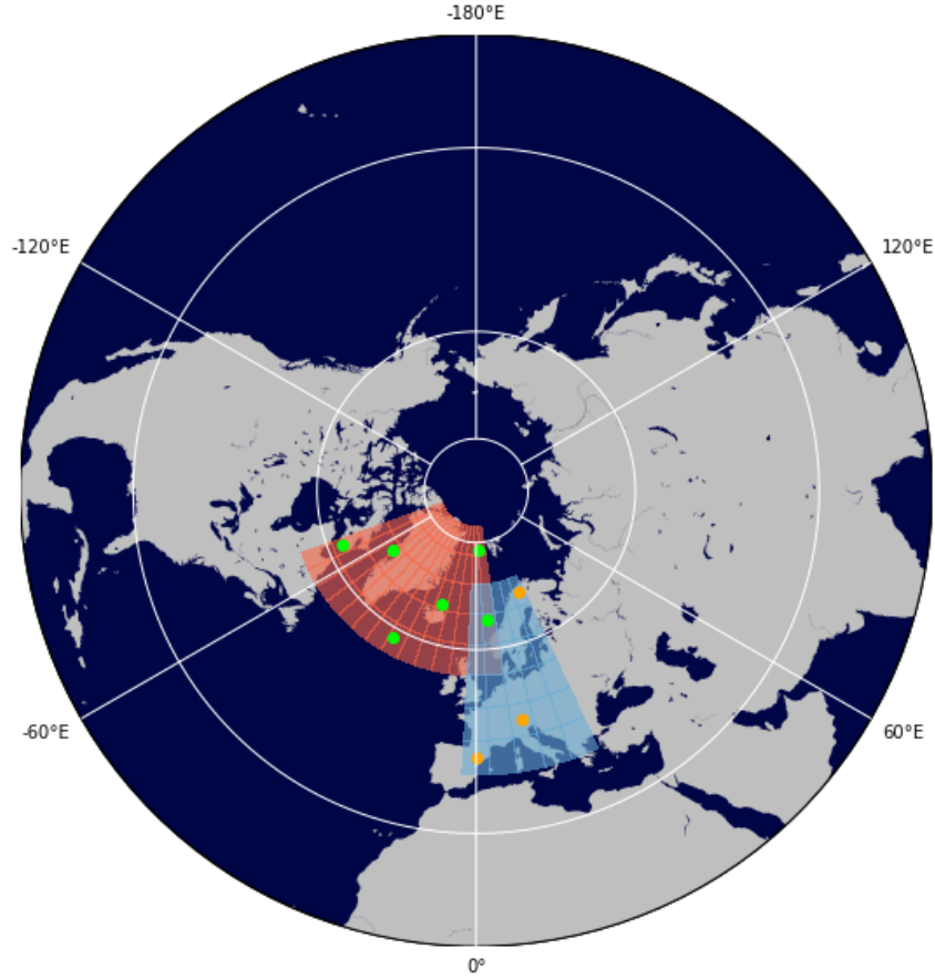
Figure 3.5: Illustration of the atmospheric zones around TS and SST proxies
