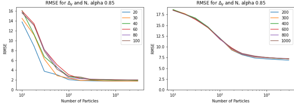
Figure 2.9: Average RMSE for Conditional Resampling based on entropy with \alpha = 0.85 , \Delta_x = 10dt (left) and \Delta_x = 100dt (right)
