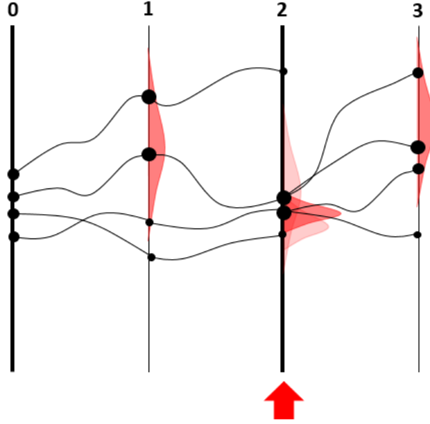
Figure 1.4: Illustration of the Cumulative Resampling Method
