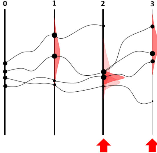
Figure 1.5: Illustration of the Conditional Resampling Method
