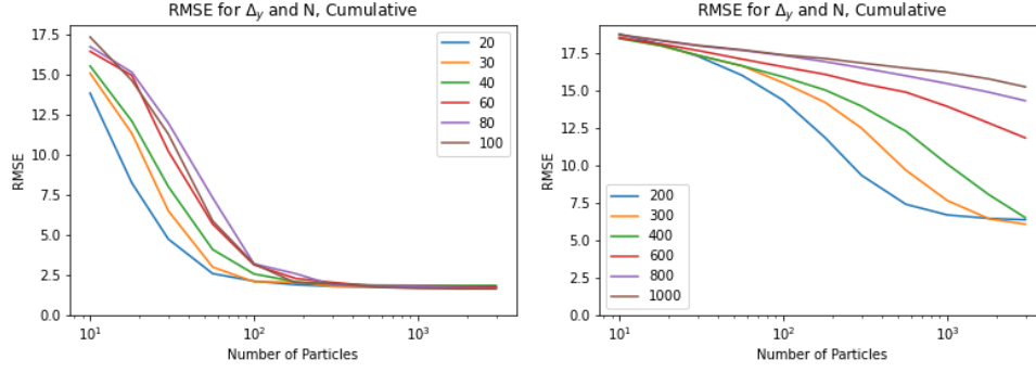
Figure 2.6: Cumulative Resampling Method \Delta_x = 10dt (left) and \Delta_x = 100dt (right)
