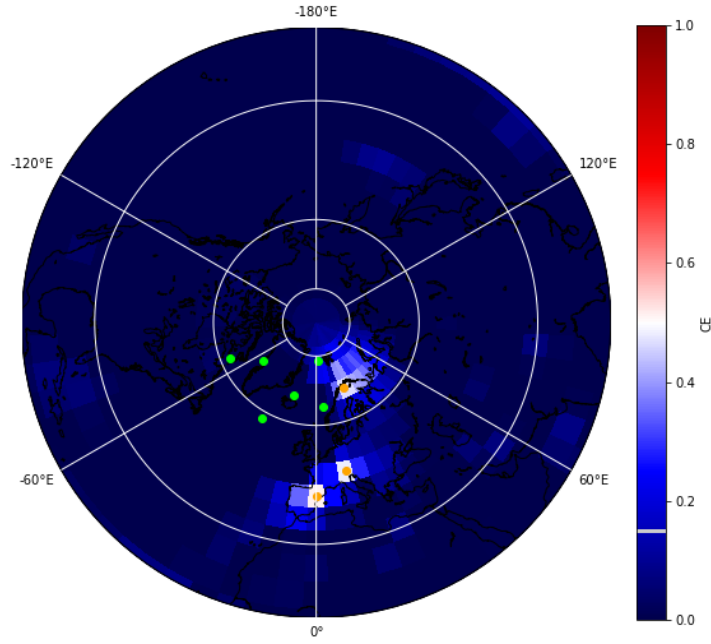
Figure 3.16: Illustration of yearly Correlation Coefficient on TS
