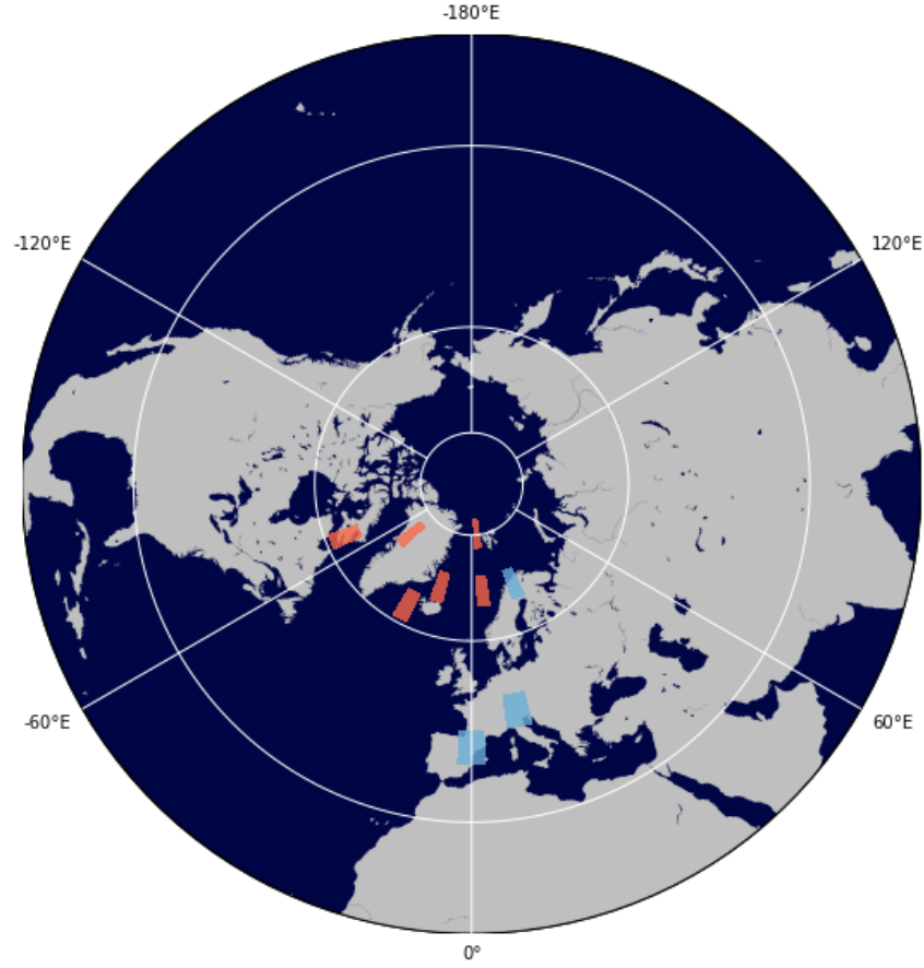
Figure 3.3: Illustration of the proxy areas in TS grid
