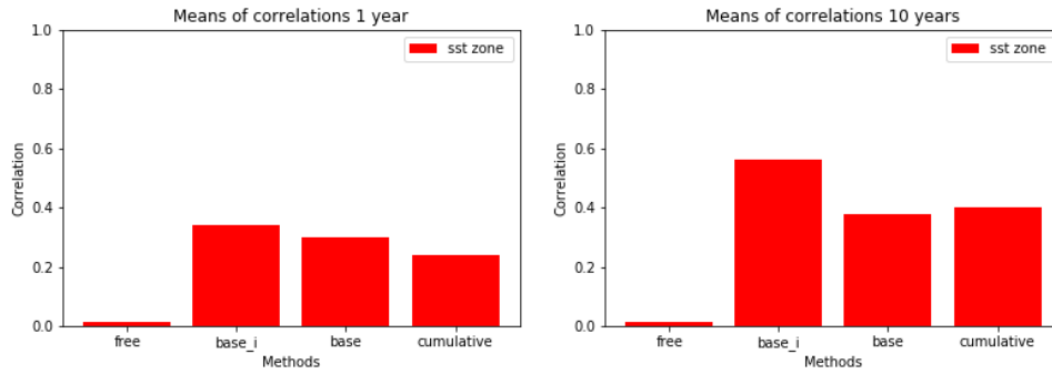
Figure 3.9: SST Correlation Coefficient Averages in the SST ocean zone, 1 year (left) and 10 years (right)
