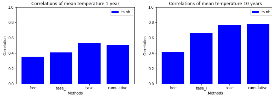
Figure 3.14: Correlation coefficients over average temperature on TS in the northern hemisphere, 1 year (left) and 10 years (right)
