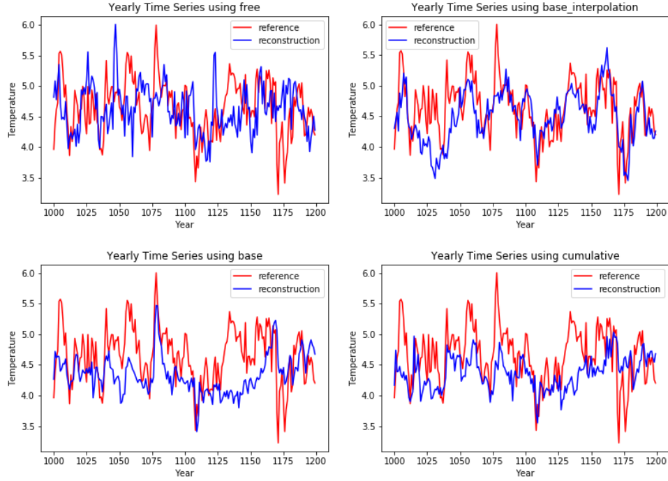
Figure 3.6: Average TS time series of reconstruction on assimilation zone for different methods
