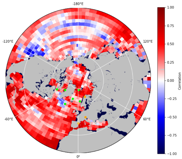
Figure 28: Illustration of decadal Correlation Coefficients on SST, cumulative
