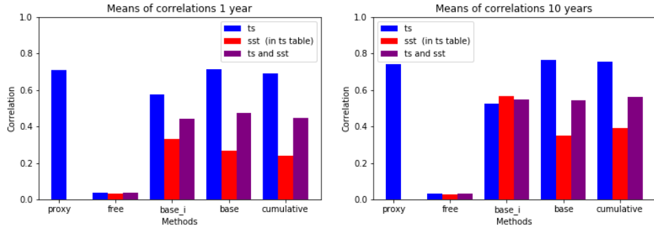
Figure 3.8: TS Correlation Coefficient Averages at SST and TS proxy locations, 1 year (left) and 10 years (right)
