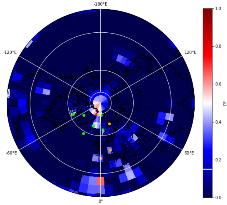
Figure 13: Illustration of decadal CE on TS, base with interpolation
