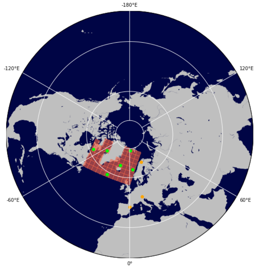
Figure 3.4: Illustration of the oceanic zone around SST proxies
