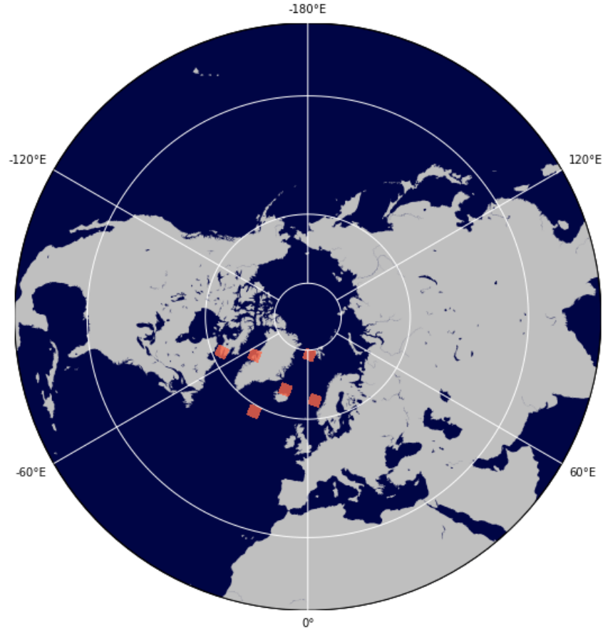
Figure 3.2: Illustration of the proxy areas in SST grid
