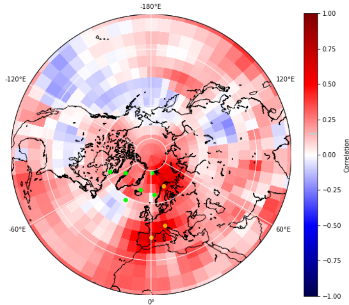
Figure 3.17: Illustration of yearly CE on TS
