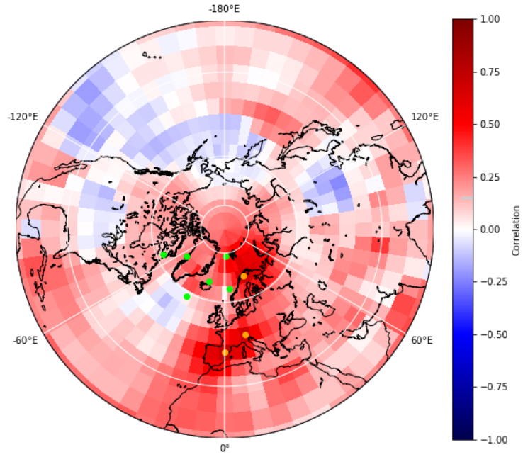
Figure 15: Illustration of yearly Correlation Coefficients on TS, base without interpolation
