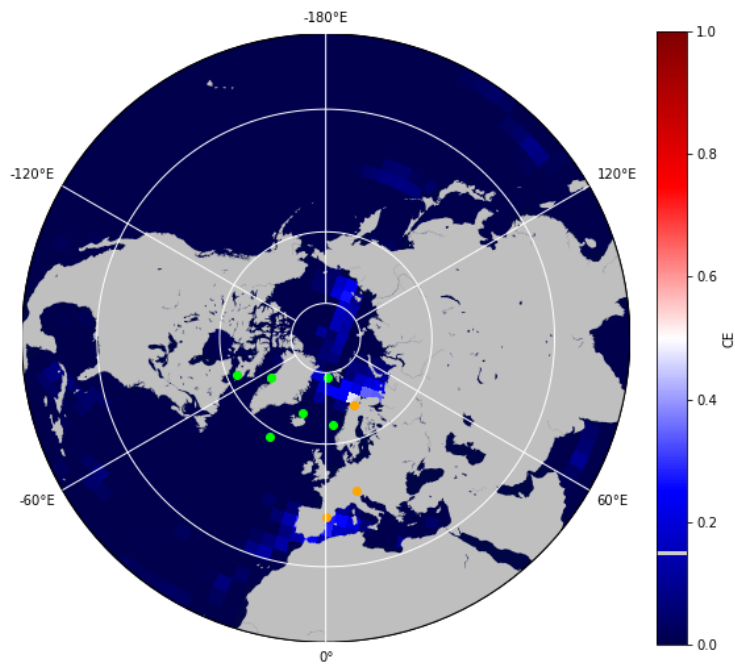
Figure 18: Illustration of yearly CE on SST, base without interpolation
