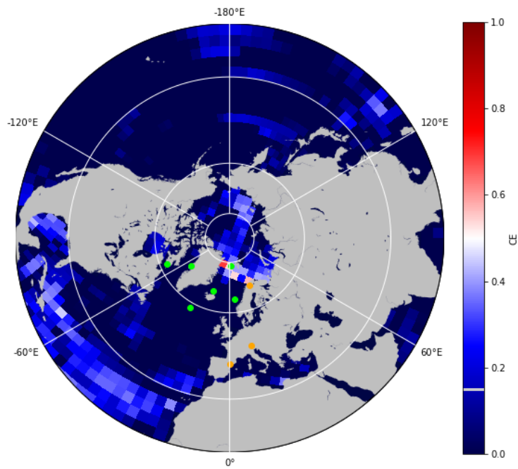
Figure 22: Illustration of decadal CE on SST, base without interpolation
