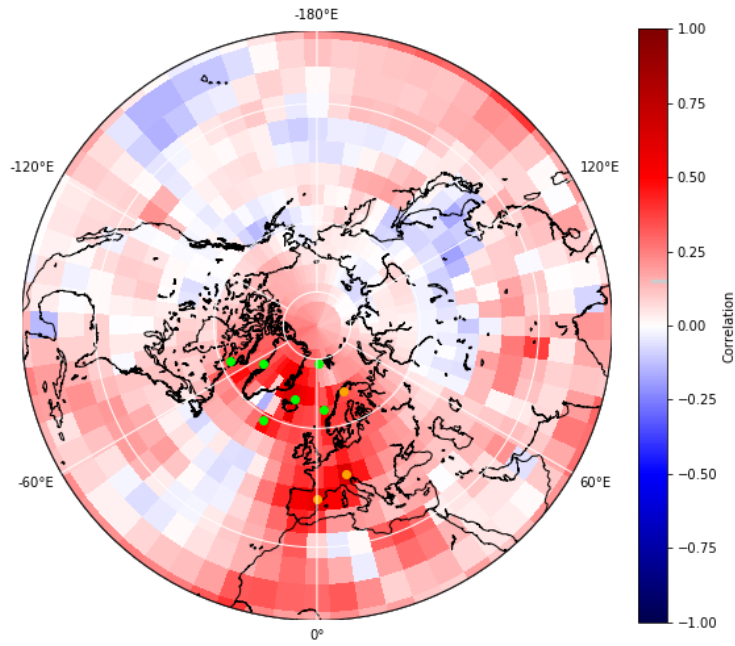
Figure 7: Illustration of yearly Correlation Coefficients on TS, base with interpolation
