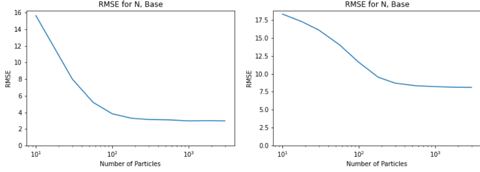
Figure 2.3: Base Method without interpolation \Delta_x = 10dt (left) and \Delta_x = 100dt (right)
