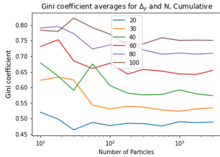
Figure 3: Average Gini, \Delta_x = 10dt
