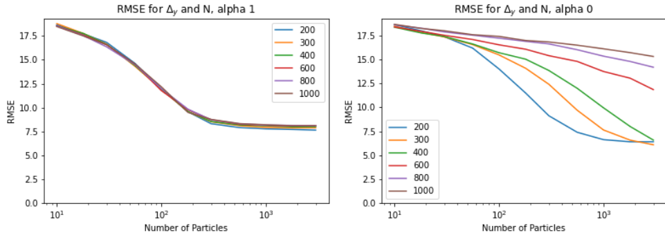
Figure 2.8: Average RMSE in Conditional Resampling for different entropy thresholds for \Delta_x = 100dt , \alpha = 1 (left) and \alpha = 0 (right)
