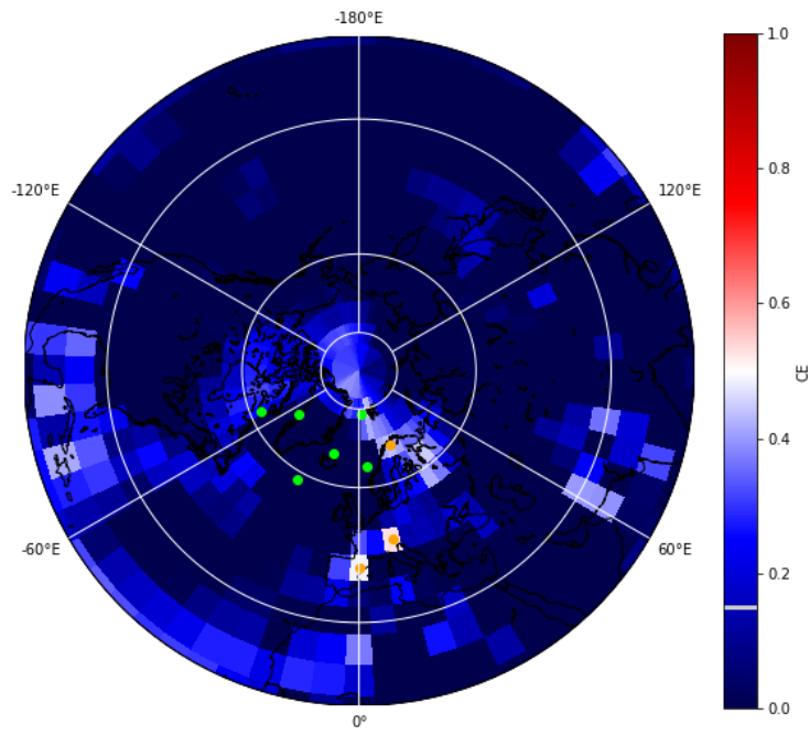
Figure 29: Illustration of decadal CE on TS, cumulative
