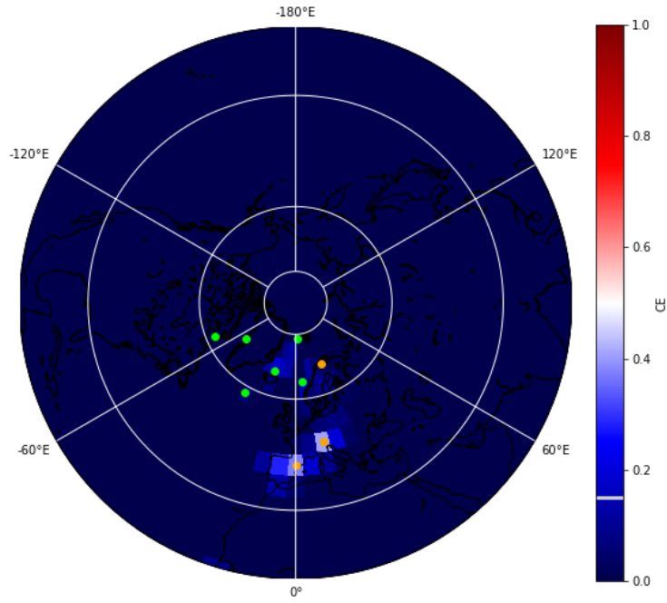
Figure 9: Illustration of yearly CE on TS, base with interpolation
