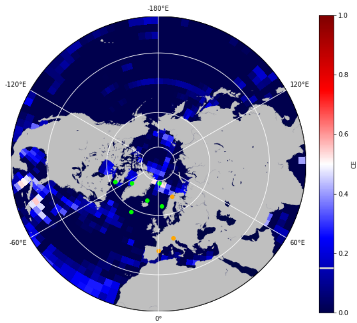
Figure 30: Illustration of decadal CE on SST, cumulative
