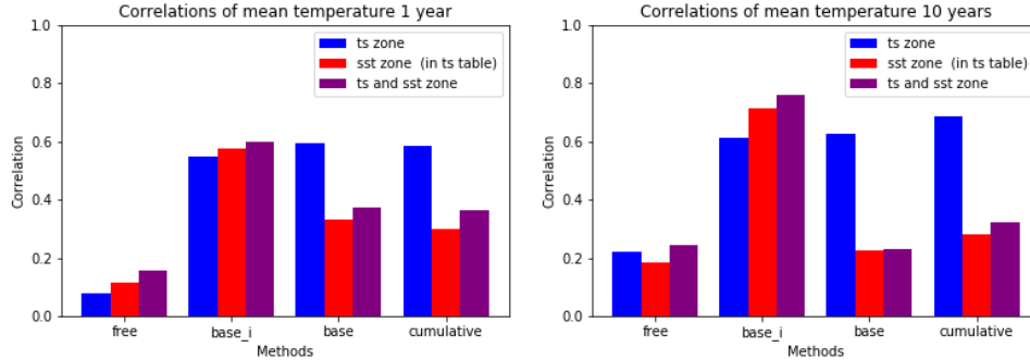
Figure 3.12: Correlation Coefficients over average TS on TS and SST proxy zones, 1 year (left) and 10 years (right)
