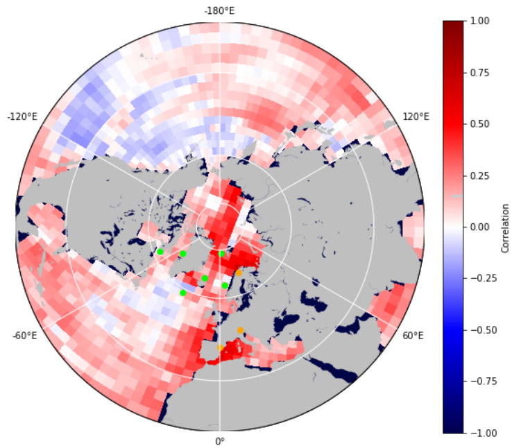
Figure 16: Illustration of yearly Correlation Coefficients on SST, base without interpolation
