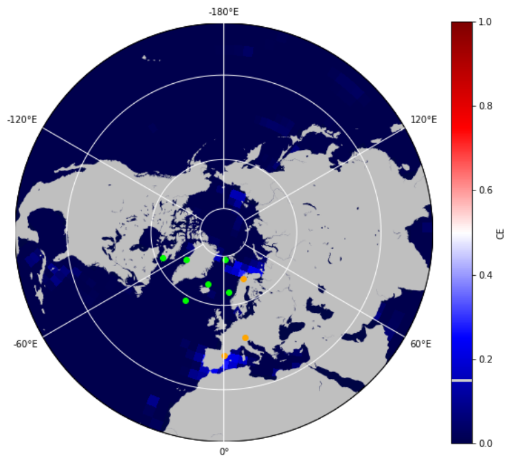
Figure 26: Illustration of yearly CE on SST, cumulative
