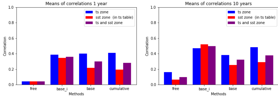
Figure 3.10: TS Correlation Coefficient Averages in the SST and TS proxy zones, 1 year(left) and 10 years (right)
