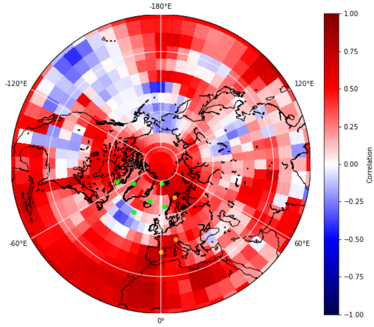
Figure 19: Illustration of decadal Correlation Coefficients on TS, base without interpolation
