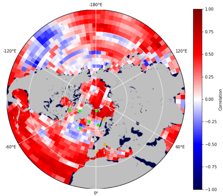
Figure 20: Illustration of decadal Correlation Coefficients on SST, base without interpolation
