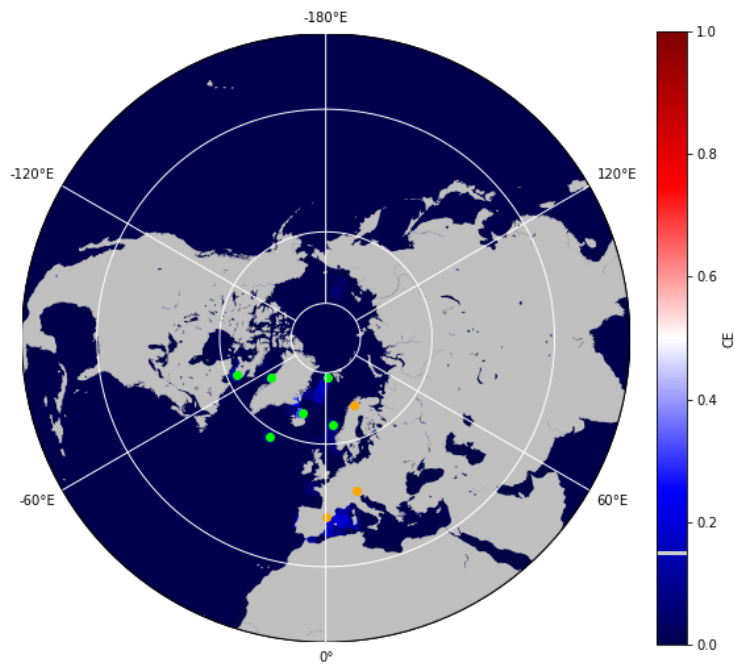
Figure 10: Illustration of yearly CE on SST, base with interpolation
