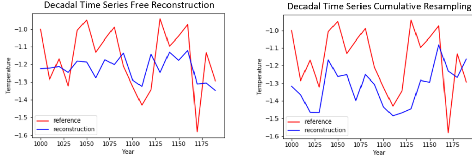
Figure 3.15: TS decadal time series over the zone enclosing all proxies, Free Reconstructions averages (left), Cumulative Resampling Method (right)
