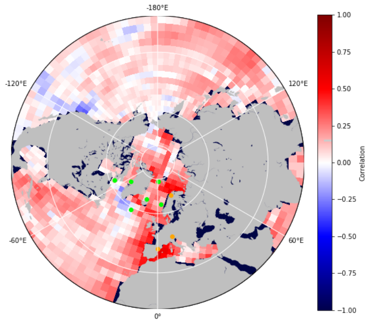
Figure 24: Illustration of yearly Correlation Coefficients on SST, cumulative
