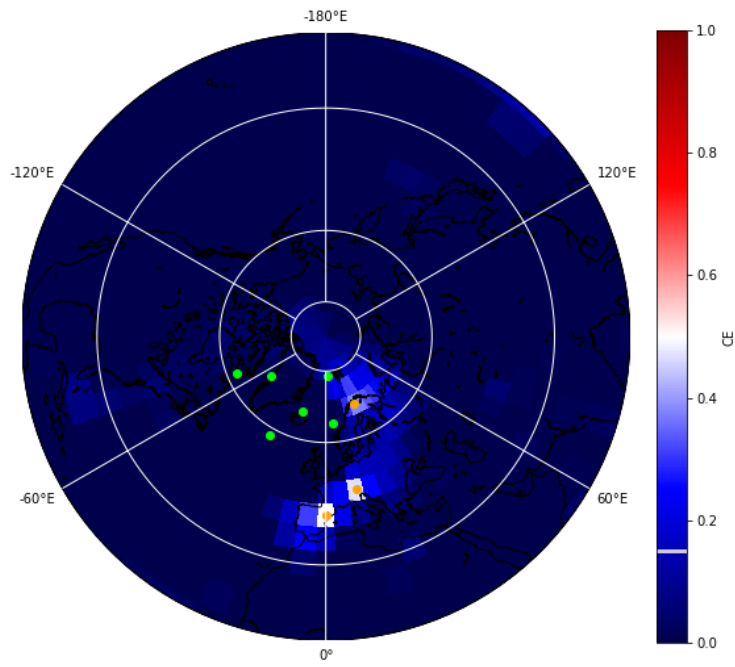
Figure 25: Illustration of yearly CE on TS, cumulative
