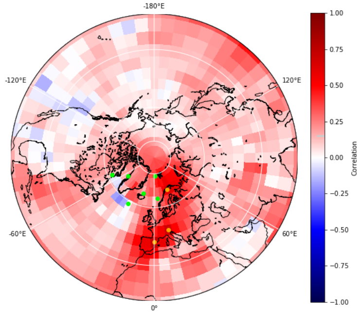
Figure 23: Illustration of yearly Correlation Coefficients on TS, cumulative
