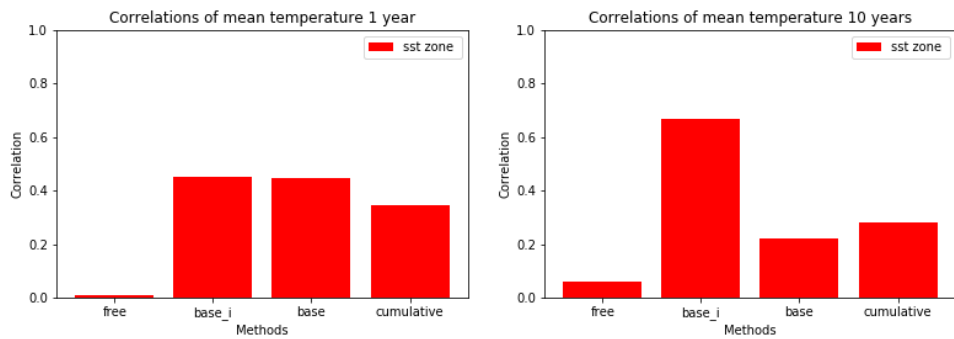
Figure 3.11: Correlation Coefficients over average SST on SST proxy zone, 1 year (left) and 10 years (right)
