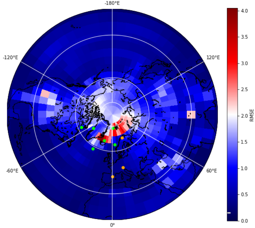
Figure 5: Illustration of the atmospheric RMSE on temperatures in the northern hemisphere
