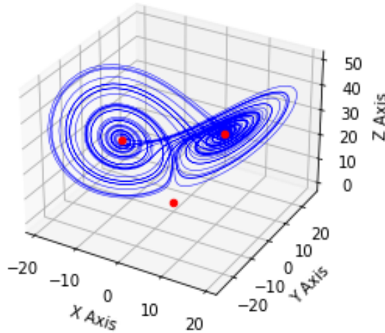
Figure 2.1: Numerical Integration of Lorenz63 with equilibria
