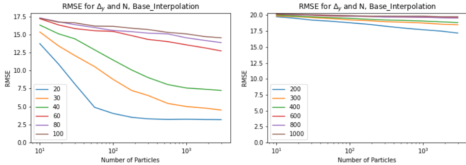
Figure 2.4: Base Method with interpolation \Delta_x = 10dt (left) and \Delta_x = 100dt (right)
