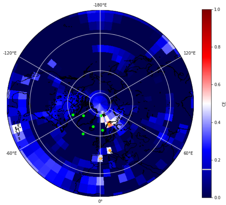
Figure 21: Illustration of decadal CE on TS, base without interpolation
