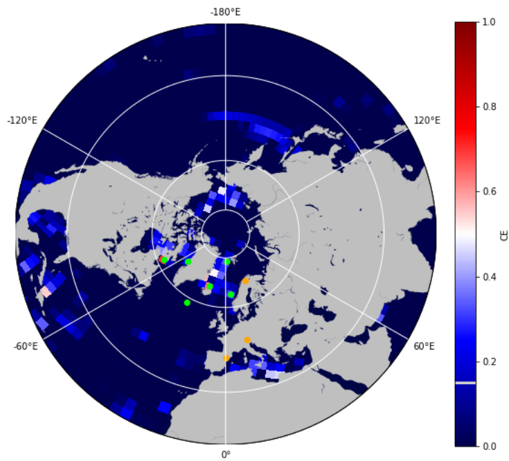
Figure 14: Illustration of decadal CE on SST, base with interpolation
