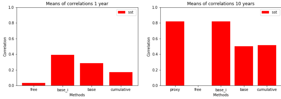
Figure 3.7: SST Correlation Coefficient Averages at SST proxy locations, 1 year (left) and 10 years (right)
