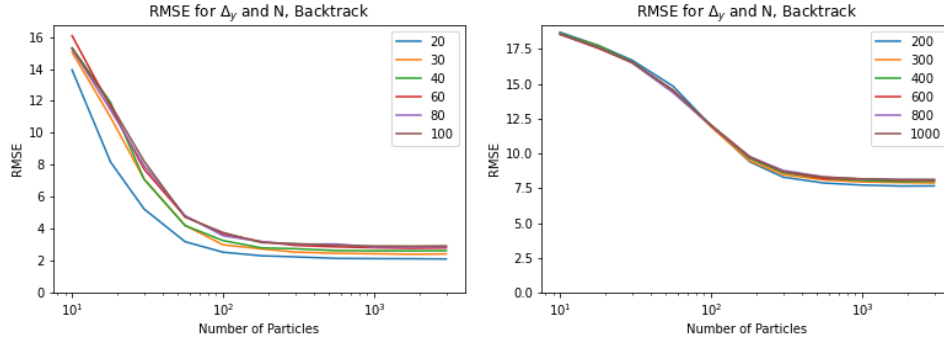
Figure 2.5: Particle Backtracking \Delta_x = 10dt (left) and \Delta_x = 100dt (right)
