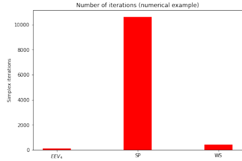
Figure 4.3: Number of simplex iterations for each solution (numerical example). Computing SP is significantly more computationally demanding than EEV_4 and WS .
