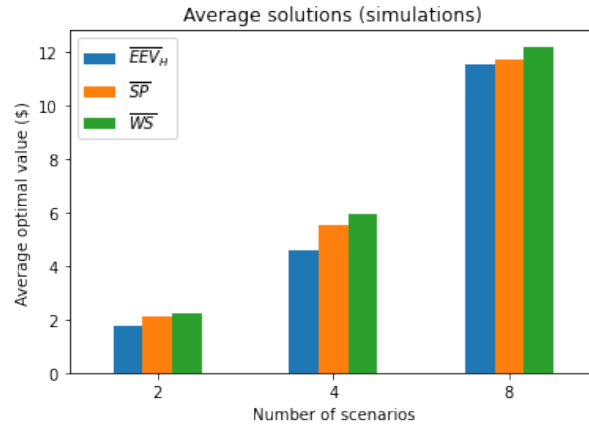
Figure 4.7: Average solutions (simulations). For all the numbers of scenarios, the inequality \overline{EEV}_H \leq \overline{SP} \leq \overline{WS} is satisfied.
