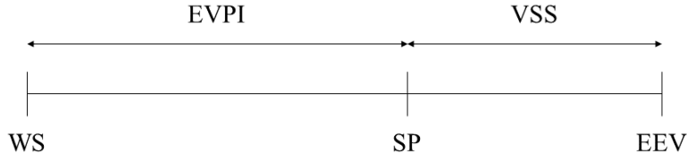
Figure 2.2: Relations between WS , SP , and EEV .
