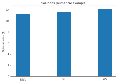
Figure 4.2: Optimal value of each solution (numerical example). As stated in Propositions 2.2.1 and 2.2.2, EEV_4 \leq SP \leq WS .
