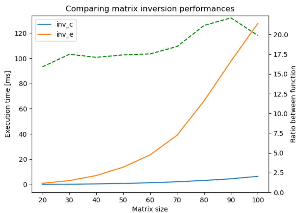
Figure 4.6: Comparison of matrix inversion
