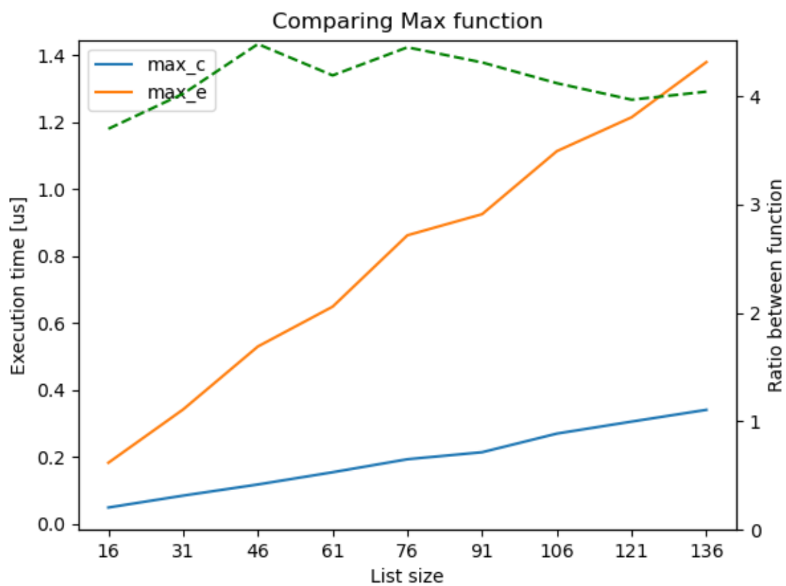
Figure 3.1: Finding maximum value within a N sized list
