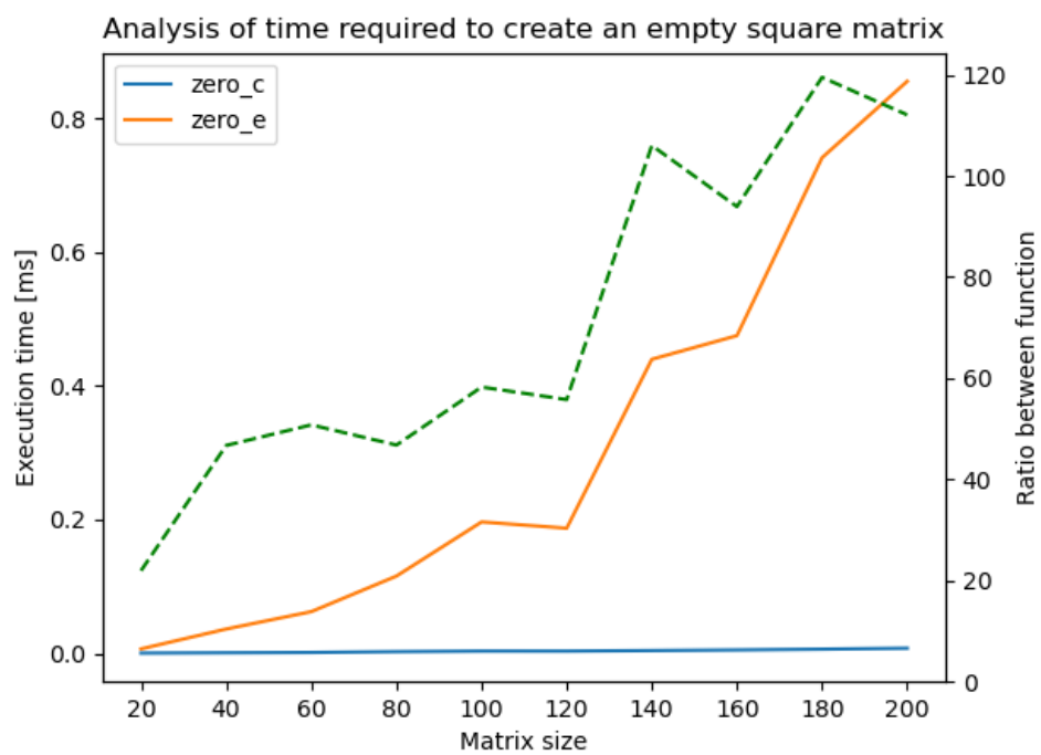
Figure 4.1: Creation of N \times N empty matrices
