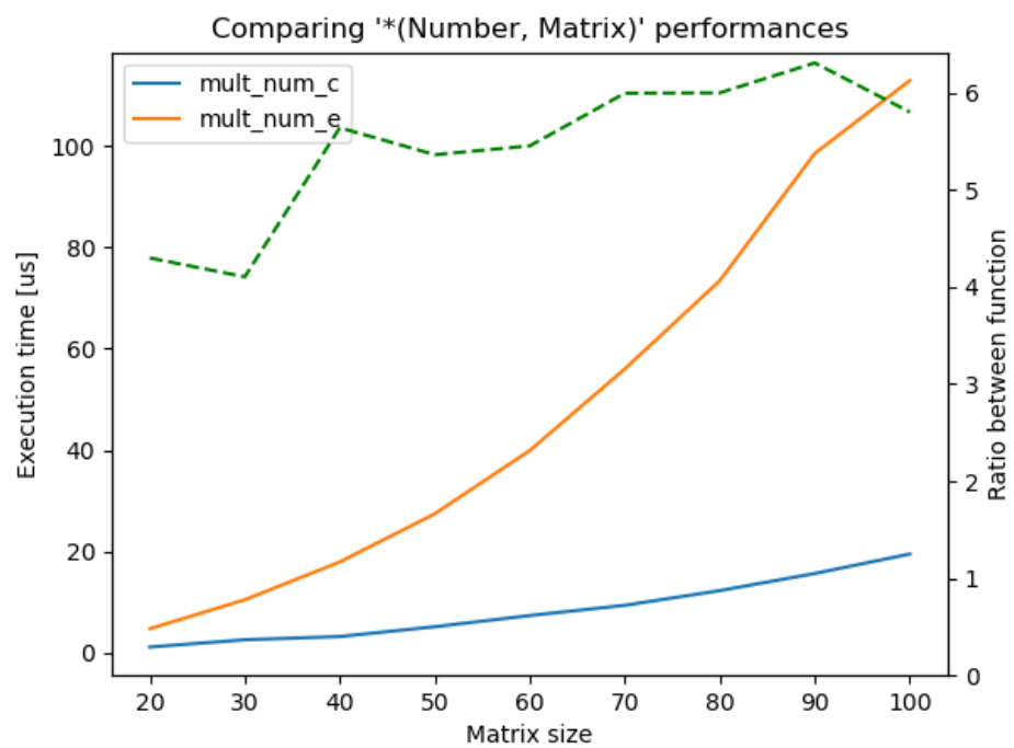
Figure 4.4: Comparison of number-matrix multiplication
