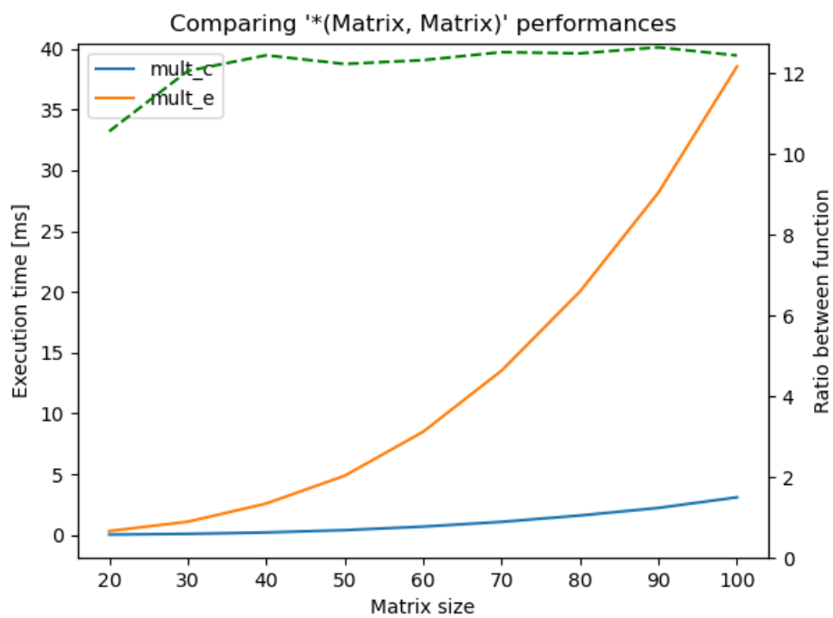
Figure 4.5: Comparison of matrix-matrix multiplication
