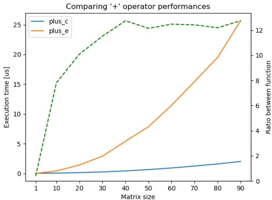
Figure 4.3: Comparison of addition
