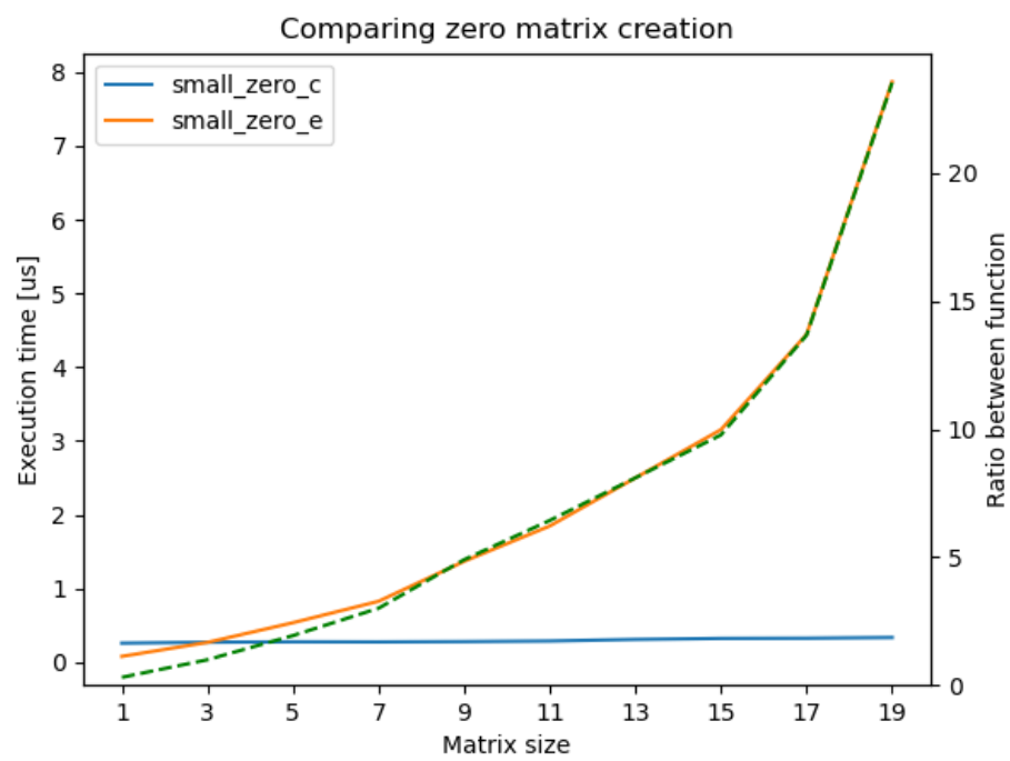
Figure 4.2: Creation of a small NxN empty matrices
