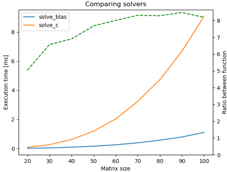
Figure 4.7: Comparison of linear system resolution
