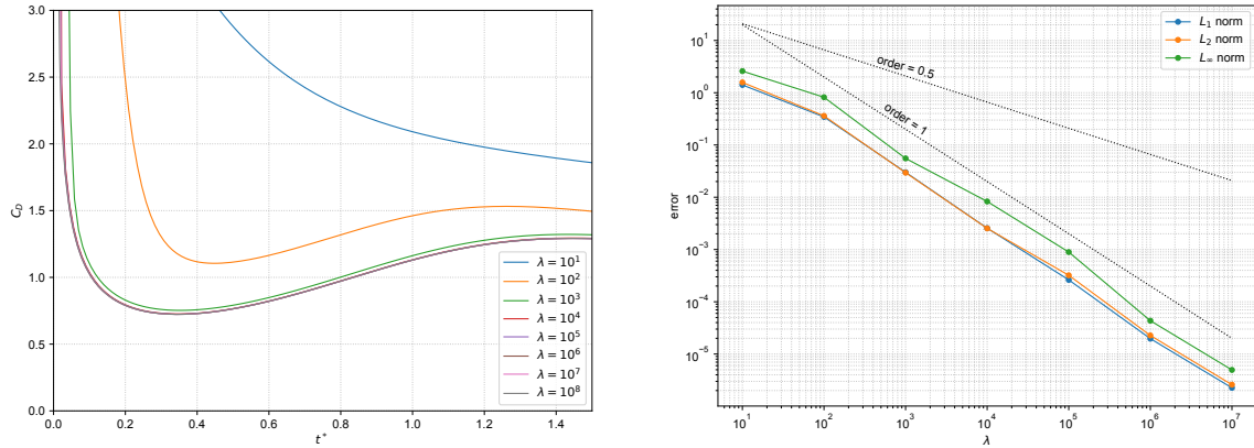
Figure 2.6: \lambda convergence study of the implicit direct method for an impulsively started flow past a cylinder at Re = 550 . Left: drag coefficient C_D evolution. Right: Convergence analysis of \lambda . The reference case is set to \lambda = 10^9 .
