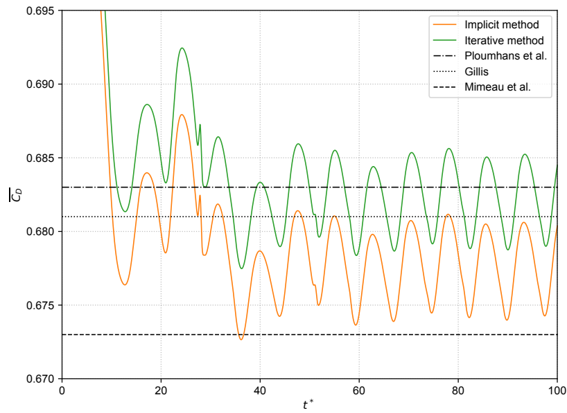
Figure 2.13: Flow past a sphere at Re = 300 . Long term drag coefficient C_D using the iterative and the implicit method and comparison with \overline{C_D} from the literature.
