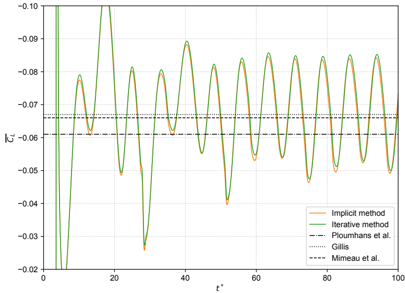
Figure 2.14: Flow past a sphere at Re = 300 . Long term lift coefficient C_L using the iterative and the implicit method and comparison with \overline{C_L} from the literature.
