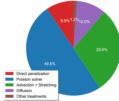
Figure 2.20: Percentage of the different stages implied in the resolution of the 3D penalized Navier-Stokes equations, in one simulation time step for the execution on 1 core, for the direct penalization methods.
