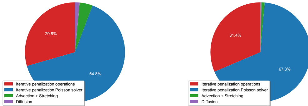
Figure 2.21: Percentage of the different stages implied in the resolution of the 3D penalized Navier-Stokes equations, in one simulation time step for the execution on 1 core, for the iterative penalization method. Left: \epsilon = 0.1 . Right: \epsilon = 0.05 .
