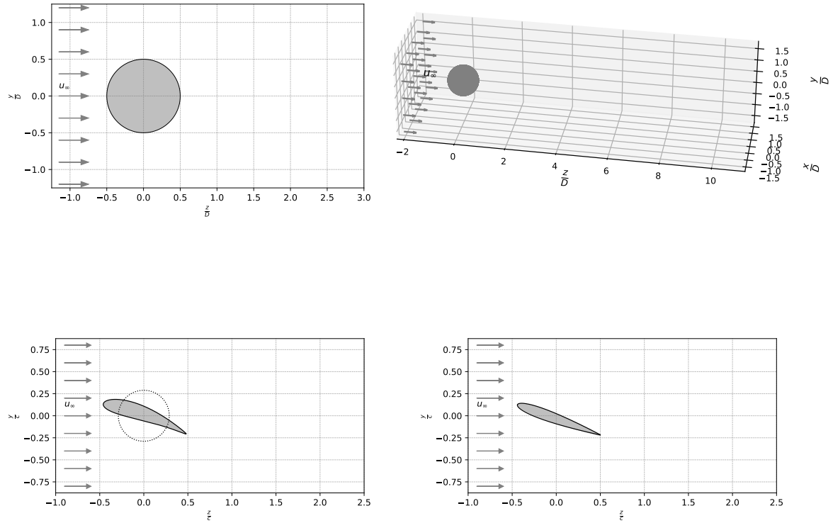
Figure 2.1: Computational domains and their corresponding mask functions \chi . Upper left: circular cylinder case (slice). Upper right: sphere case. Lower left: Joukowski airfoil section and its corresponding inverse Joukowski transform. Lower right: NACA0012 airfoil section. Both airfoils here have an angle of attack (AoA) \alpha = 20^\circ . The uniform upstream velocity is also represented.
