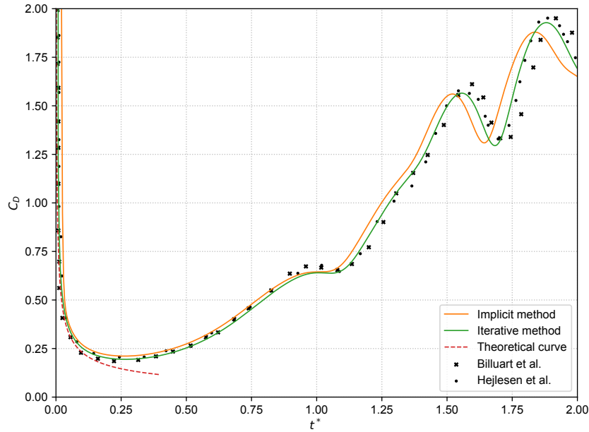
Figure 2.9: Impulsively started cylinder at Re = 9500 . Long time comparison with Hejlesen et al. [7] and Billuart et al. [35]. The first time step is \Delta t^* = 10^{-6} .
