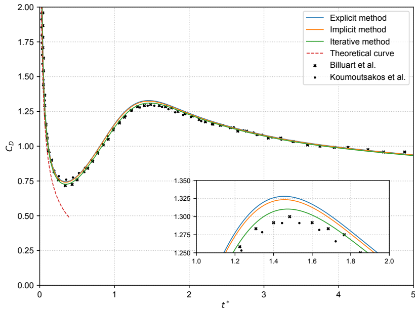
Figure 2.2: Impulsively started cylinder at Re = 550 . Short time comparison with the theoretical curve of Barlev et al. [34]. The first time step is \Delta t^* = 10^{-6} .
