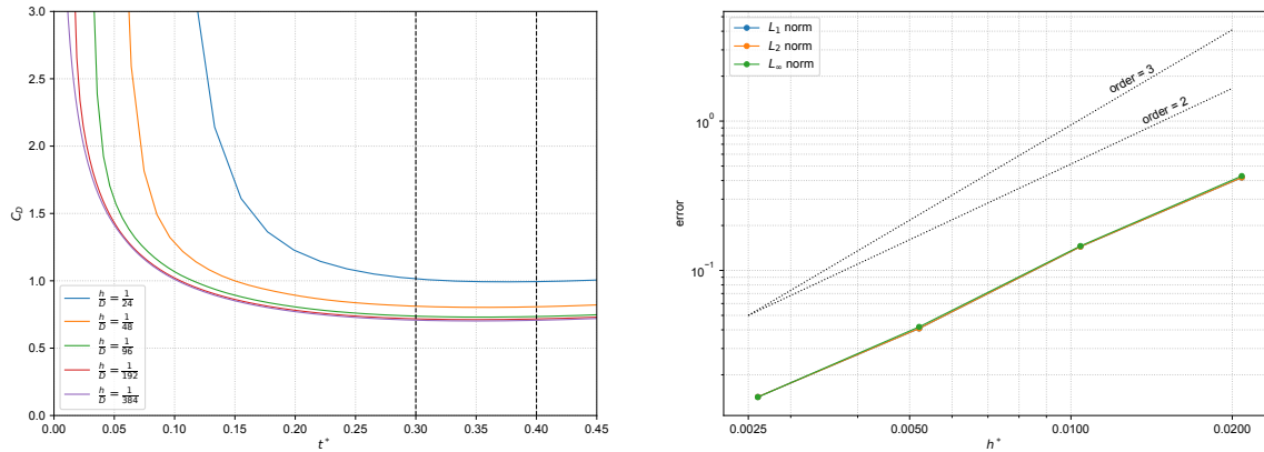
Figure 2.7: Grid-convergence study on the drag coefficient for flow past a circular cylinder at Re = 550 for the iterative method. Left: drag coefficient C_D evolution. The section on which the analysis is done is between the black dashed lines. Right: grid convergence analysis of the problem. The reference mesh is h^* = \frac{1}{384} .
