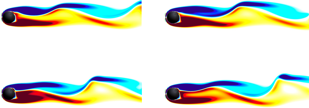
Figure 2.15: Flow past a sphere at Re = 300 . Vorticity \omega_x^* in the YZ plane for every quarter period of a shedding cycle, with the iterative method and \epsilon = 0.1 . The color plot is saturated for |\omega_x^*| \geq 6 .
