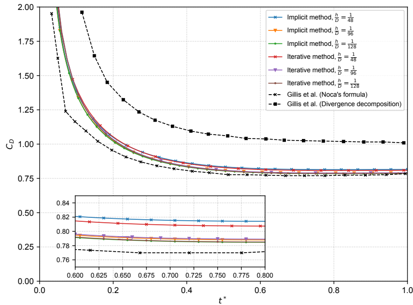
Figure 2.12: Impulsively started sphere at Re = 300 . Comparison of the drag coefficients with Gillis [6]. The two reference solutions use h^* = \frac{1}{128} .
