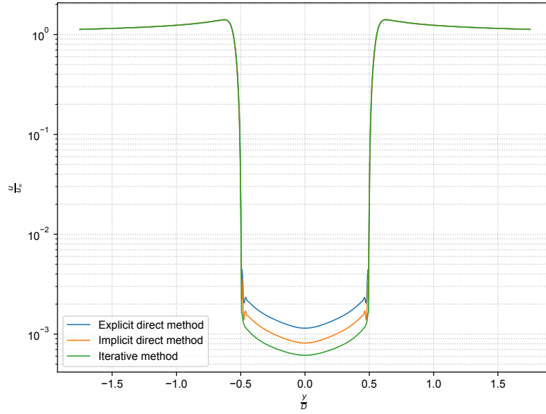
Figure 2.5: Mean velocity magnitude profiles u^* at t^* \simeq 3 in a section across the center of the cylinder at \frac{x}{D} = 0 . The object is located between \frac{y}{D} = -0.5 and \frac{y}{D} = 0.5 .
