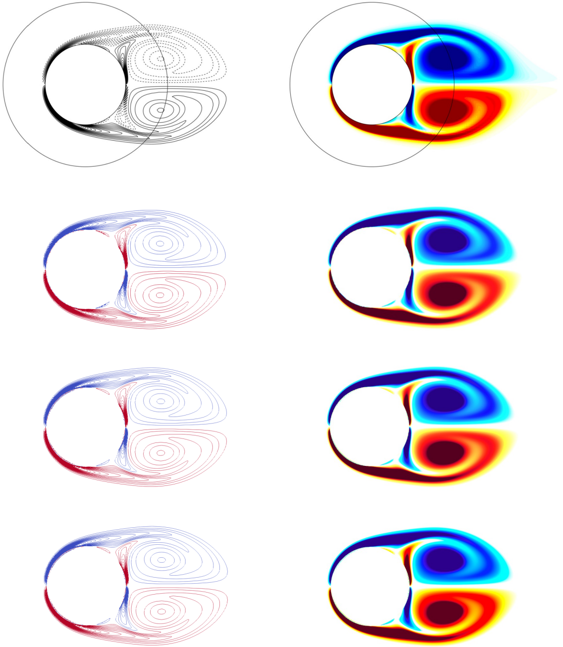
Figure 2.4: Impulsively-started cylinder at \text{Re} = 550 : contours of dimensionless vorticity at t^* \simeq 4 . Contour levels are by steps of 1.5. The color plot is saturated for |\omega_x^*| > 6 . First row: Billuart et al. [35] at t^* \simeq 4 . The circle represents the boundary between his Near-Wall (NW) region and his Vortex Particle-Mesh (VPM) region. Second row: Explicit approach with \lambda\Delta t = 1 . Third row: Implicit approach with \lambda = 10^8 . Fourth row: Iterative approach with \alpha = 1.9 and \epsilon = 0.05 .
