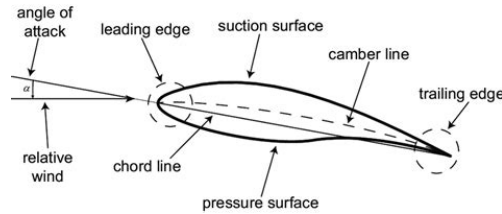
Figure A.1: Airfoil terminology, from [42]
