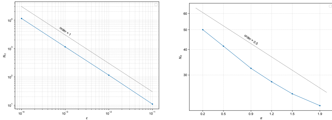
Figure 2.11: Impulsively started cylinder at Re = 9500 , iterative method sensitivity analysis. Left : Number of iterations as a function of the stopping criterion \epsilon , for \alpha = 1.9 . Right = Number of iterations as a function of \alpha , for \epsilon = 0.05 .
