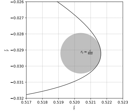
Figure A.2: Radius of curvature of the Regularized Joukowski airfoil
