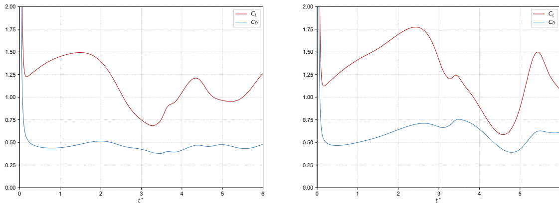
Figure 2.18: Flow past the airfoils at Re = 1000 and \alpha = 20^\circ : evaluation of the forces. Left: regularized Joukowski airfoil with r_t \approx \frac{1}{400} . Right: NACA0012 airfoil.
