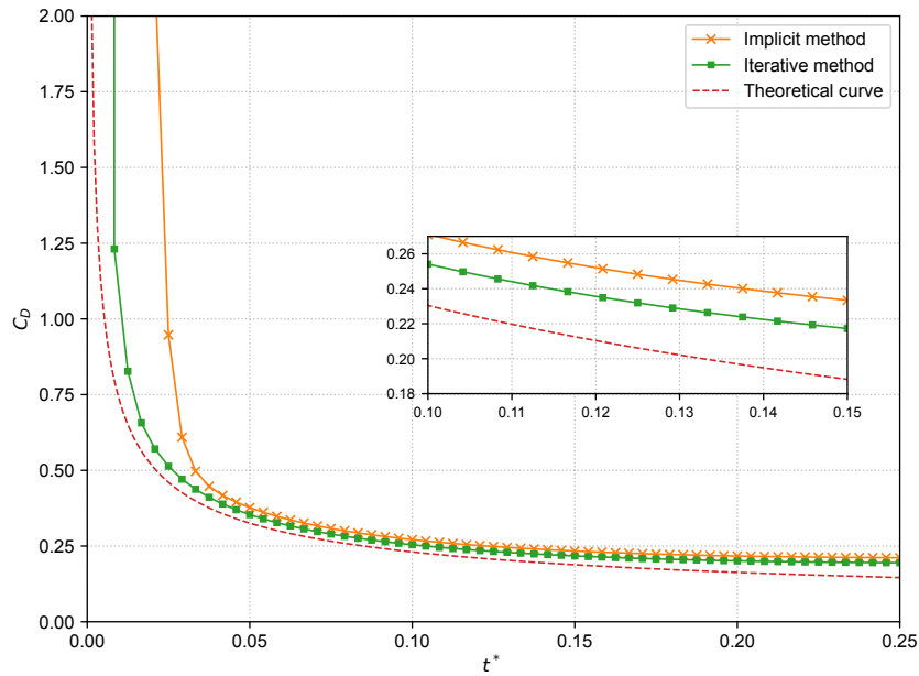
Figure 2.8: Impulsively started cylinder at Re = 9500 . Short time comparison with the theoretical curve of Barlev et al. [34]. The first time step is \Delta t^* = 10^{-6} .
