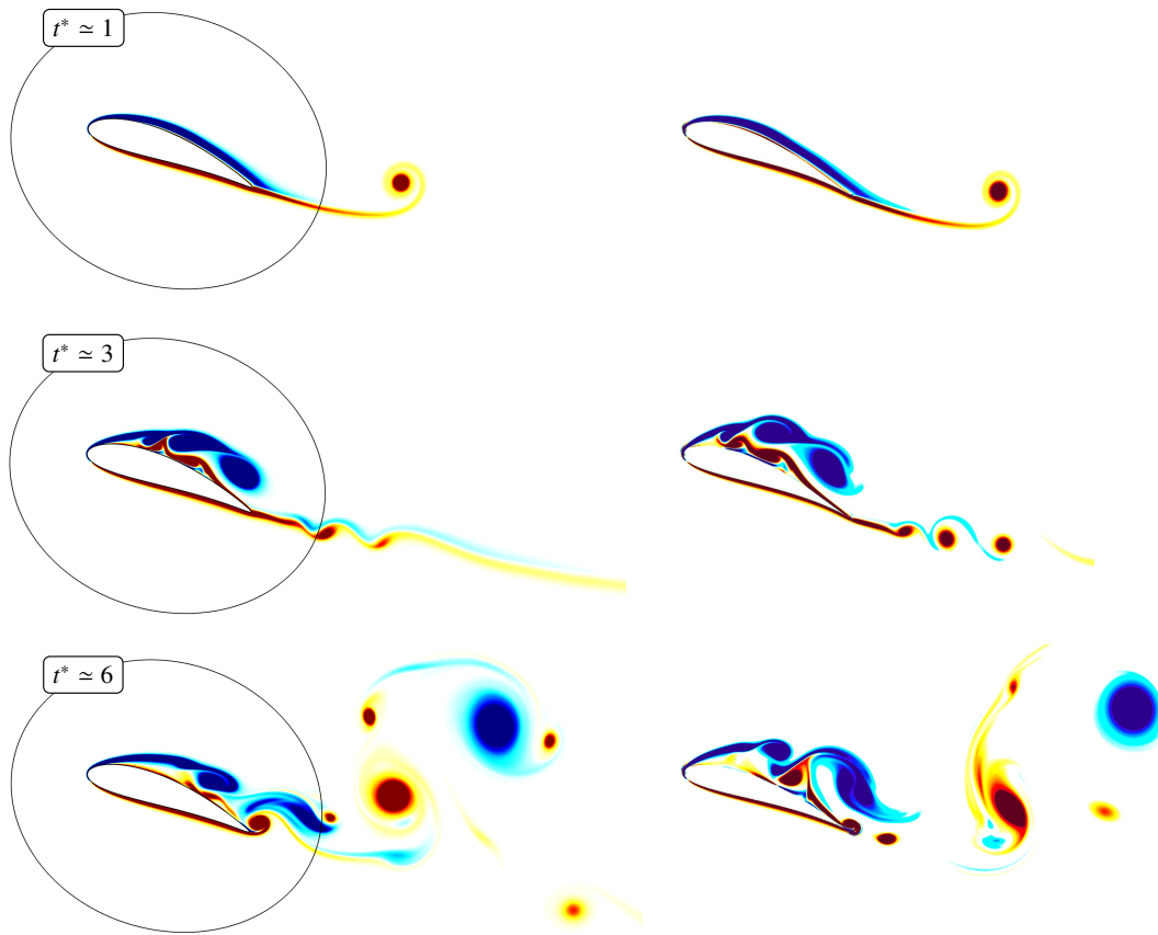
Figure 2.19: Dimensionless vorticity field for airfoils at Re = 5000 and \alpha = 20^\circ . Left column : regularized Jukowski airfoil. Right column : NACA0012 airfoil. First row : t^* \simeq 1 . Second Row : t^* \simeq 3 . Third row : t^* \simeq 6 . The plot is saturated for |\omega_x^*| > 15 . The two airfoils are scaled with the same chord length. The iterative method is used with \epsilon = 0.05 and \alpha = 1.9 .
