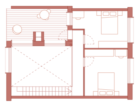
R+1
