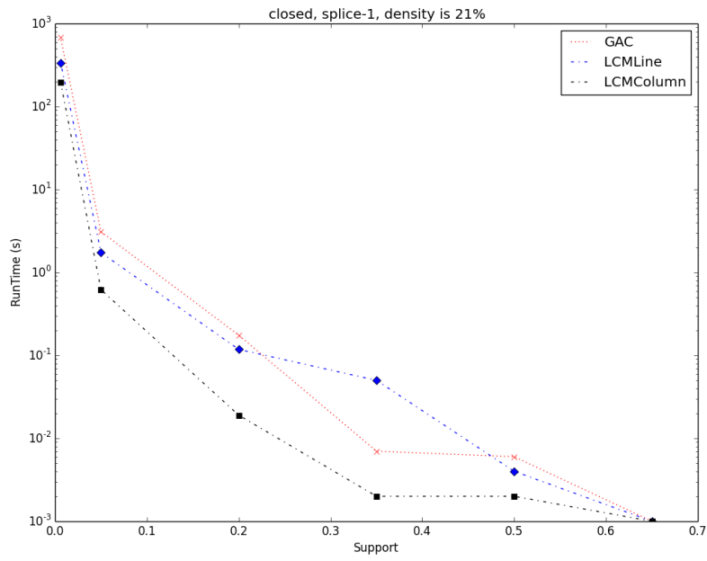
Figure A.8: comparisons for the CFIMP on the splice-1 dataset
