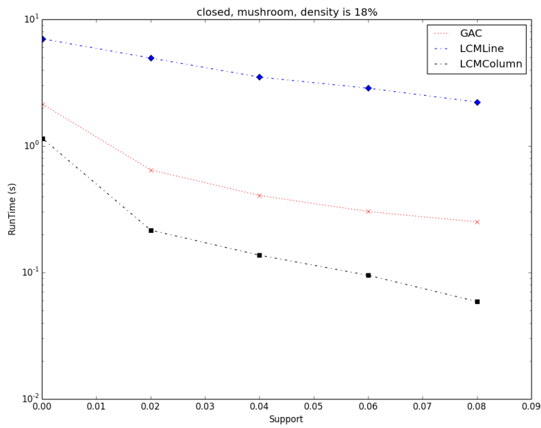
Figure A.9: comparisons for the CFIMP on the mushroom dataset
