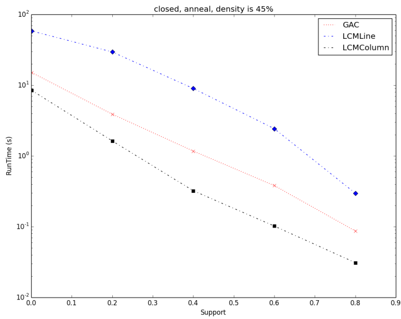
Figure A.7: comparisons for the CFIMP on the anneal dataset
