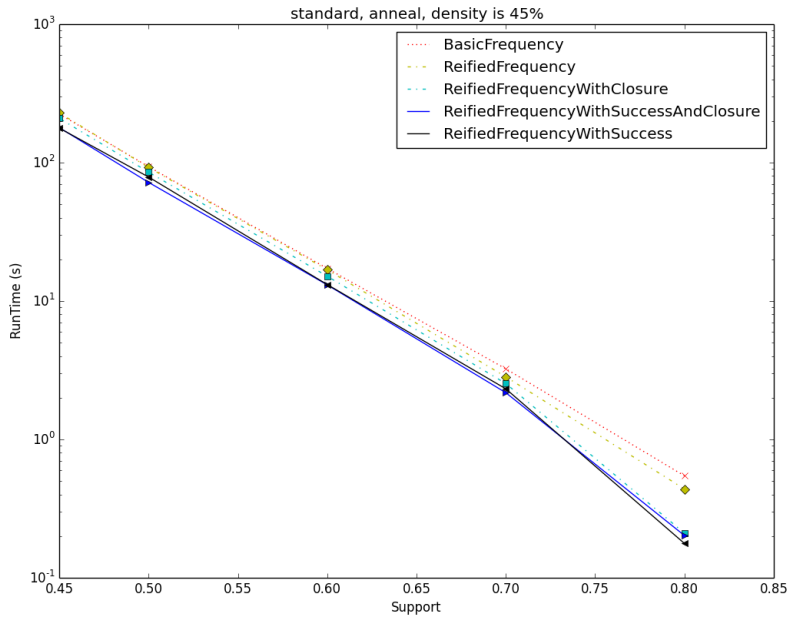
Figure A.2: comparisons for the FIMP on the anneal dataset
