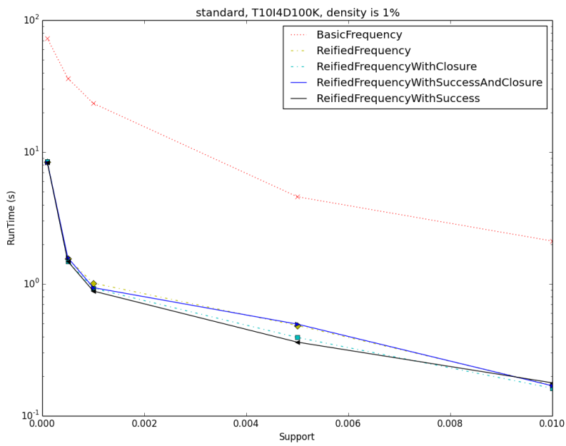
Figure A.5: comparisons for the FIMP on the T1014D100K dataset
