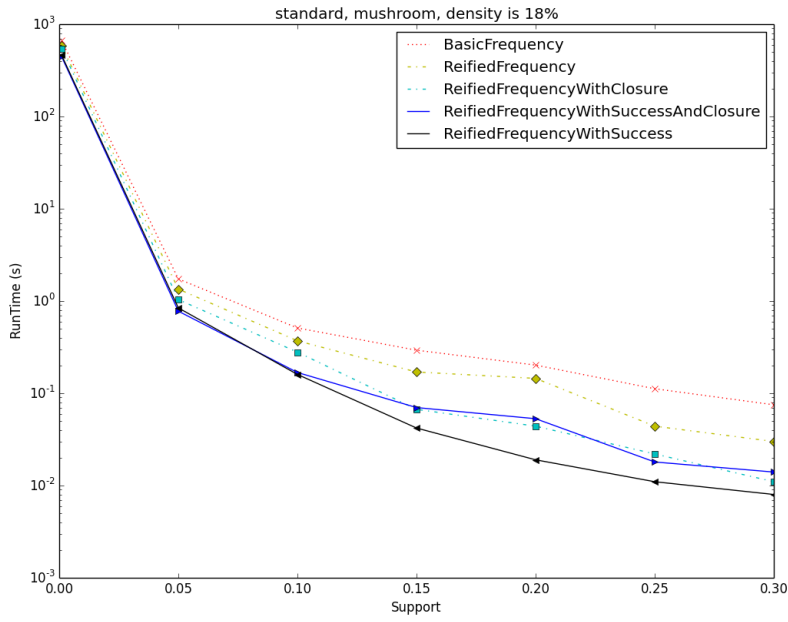
Figure A.4: comparisons for the FIMP on the mushroom dataset
