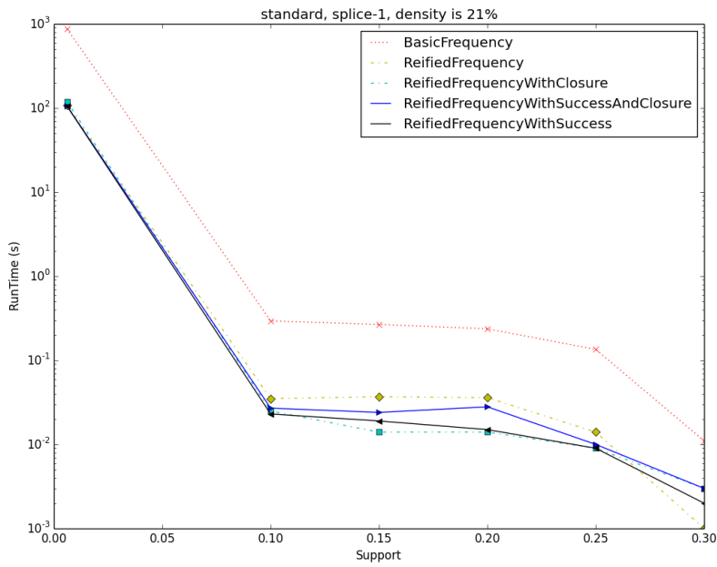
Figure A.3: comparisons for the FIMP on the splice-1 dataset
