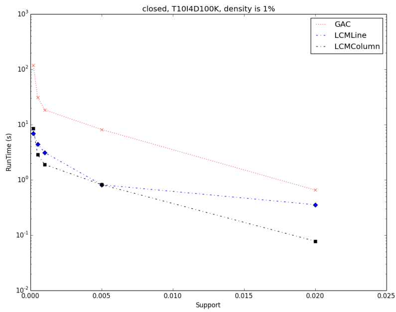
Figure A.10: comparisons for the CFIMP on the T10I4D100K dataset
