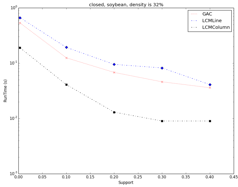
Figure A.6: comparisons for the CFIMP on the soybean dataset
