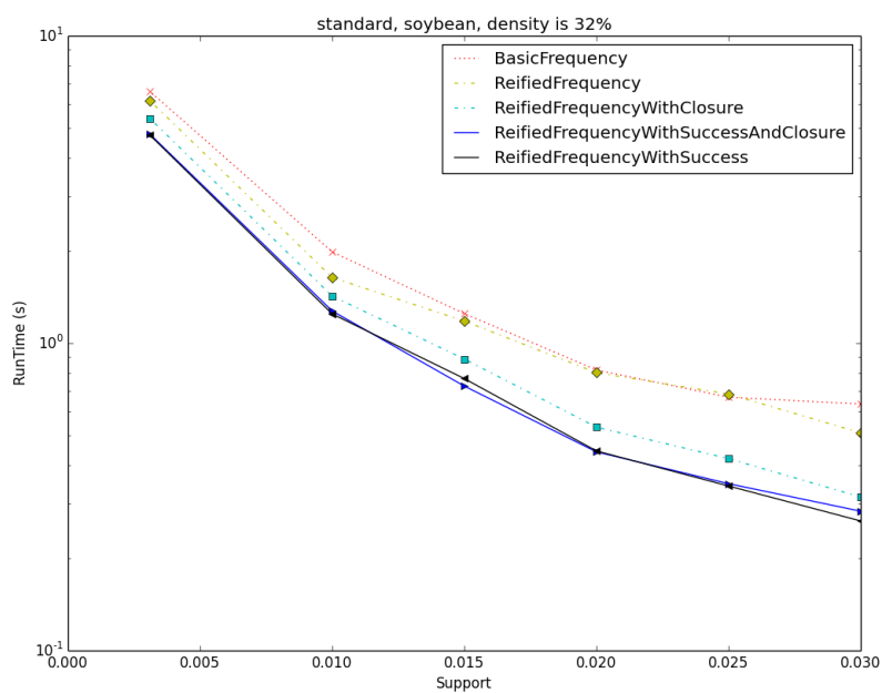
Figure A.1: comparisons for the FIMP on the soybean dataset
