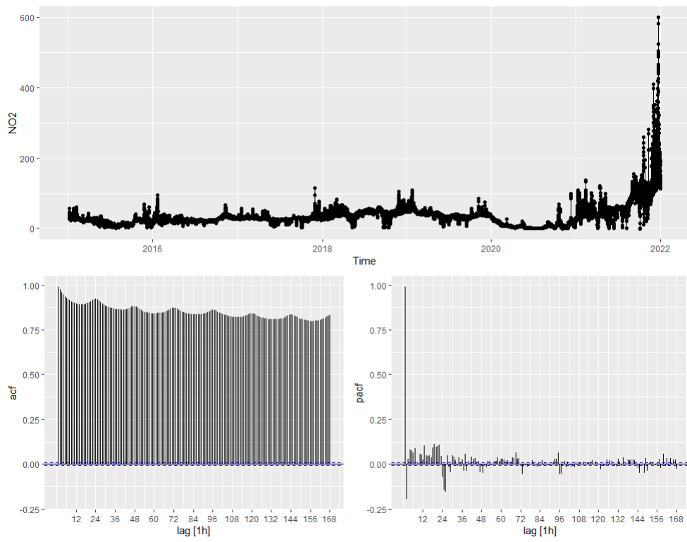
Figure 40: pACF Southern Norway
