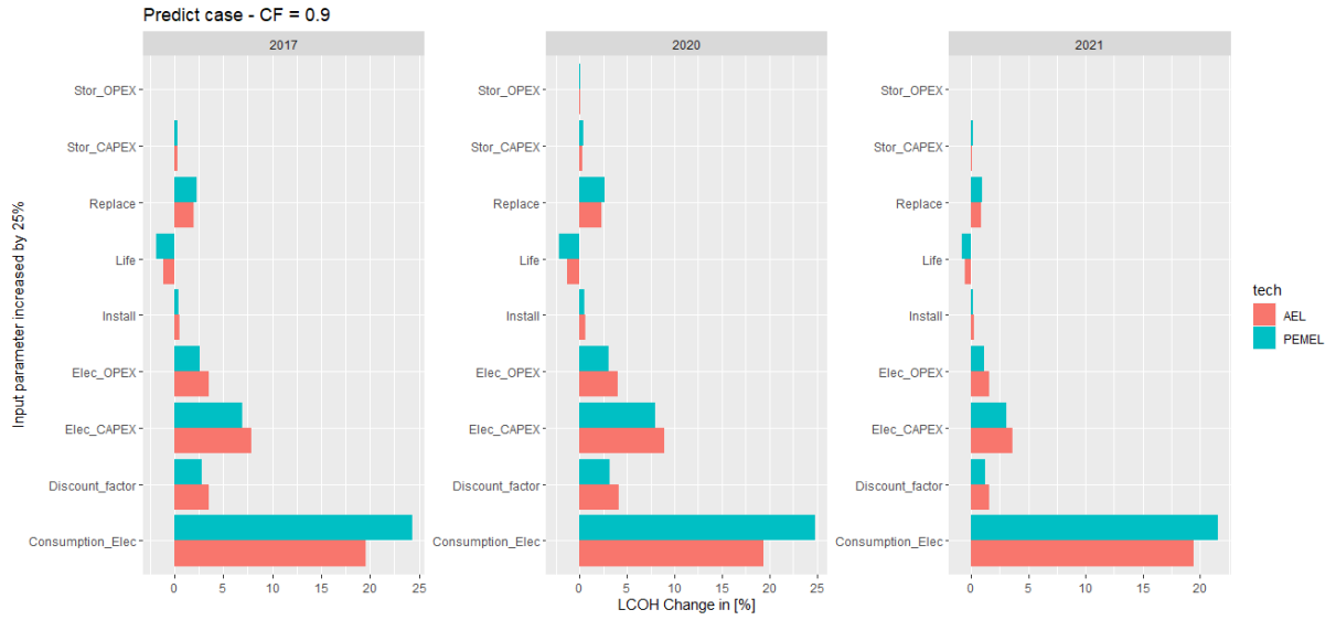
Figure 24: Sensitivity for DK1 using Forecasted prices at a Capacity Factor of 0.9
