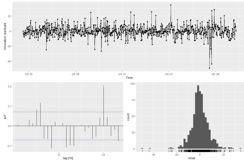
Figure 12: BE residuals
