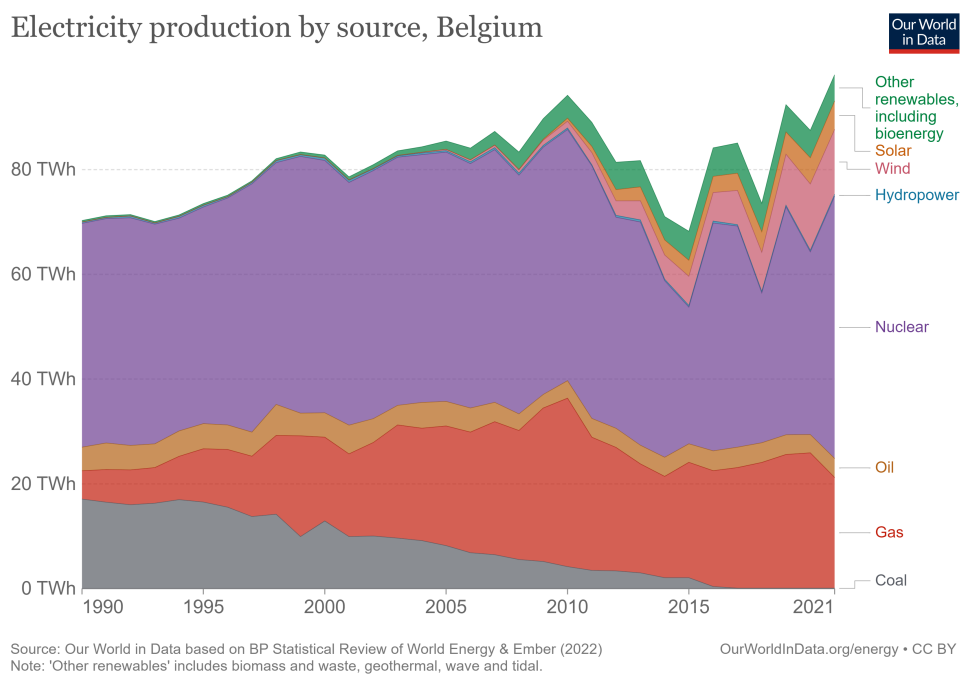
Figure 33: Belgium electricity generation mix [58]
