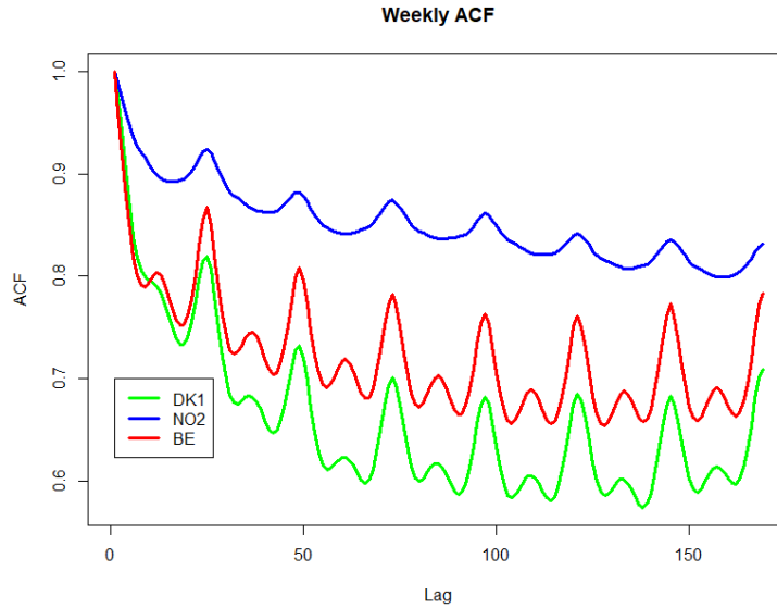
Figure 11: Weekly ACF
