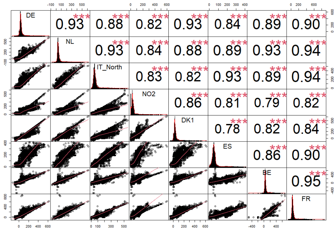
Figure 26: Chart Correlation
