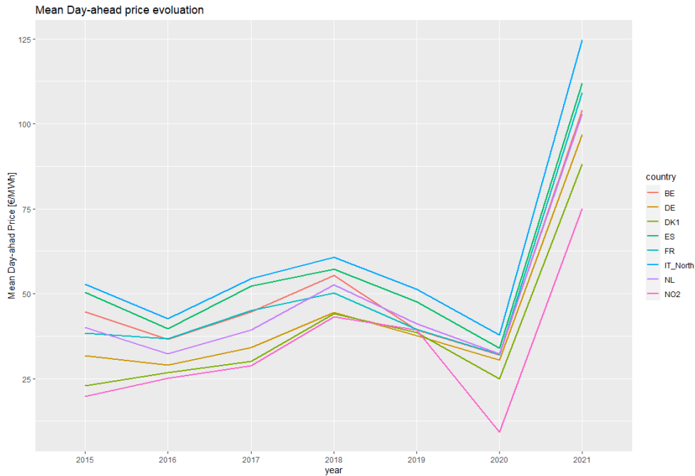
Figure 3: Mean day-ahead price evolution
