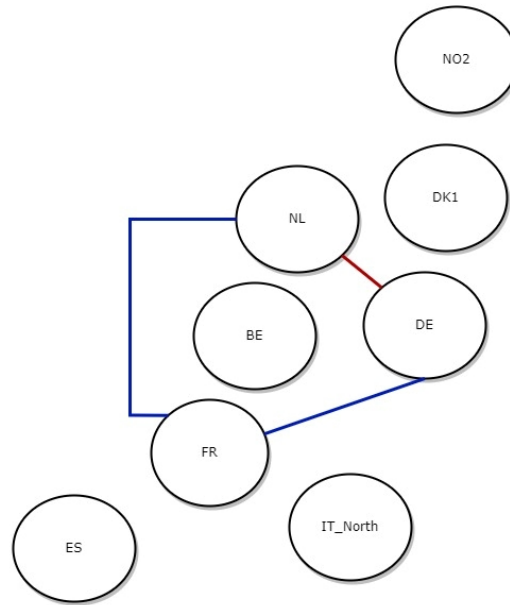
Figure 28: Daily variability diagram
