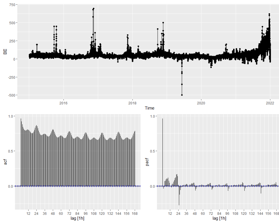
Figure 39: pACF Belgium
