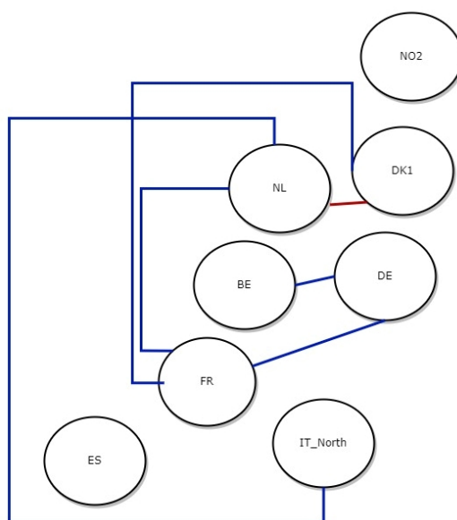
Figure 29: Weekly variability diagram
