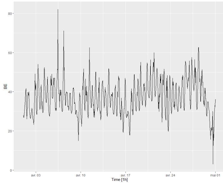
Figure 10: Belgian day-ahead power prices in April 2017 [€/MWh]
