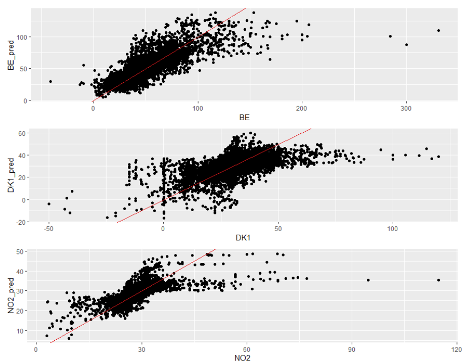
Figure 44: Year 2017
