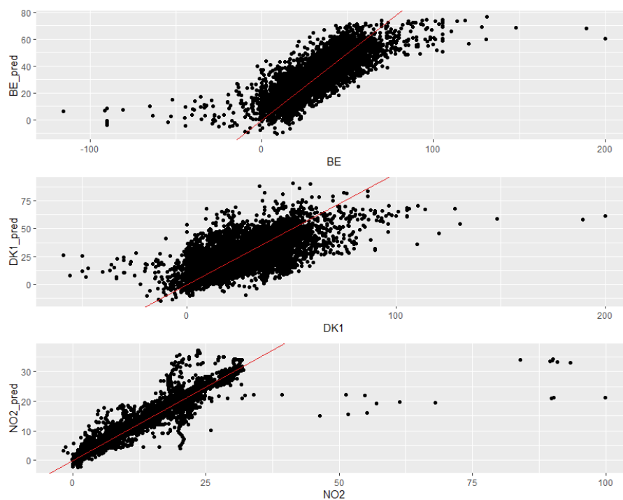
Figure 45: Year 2020
