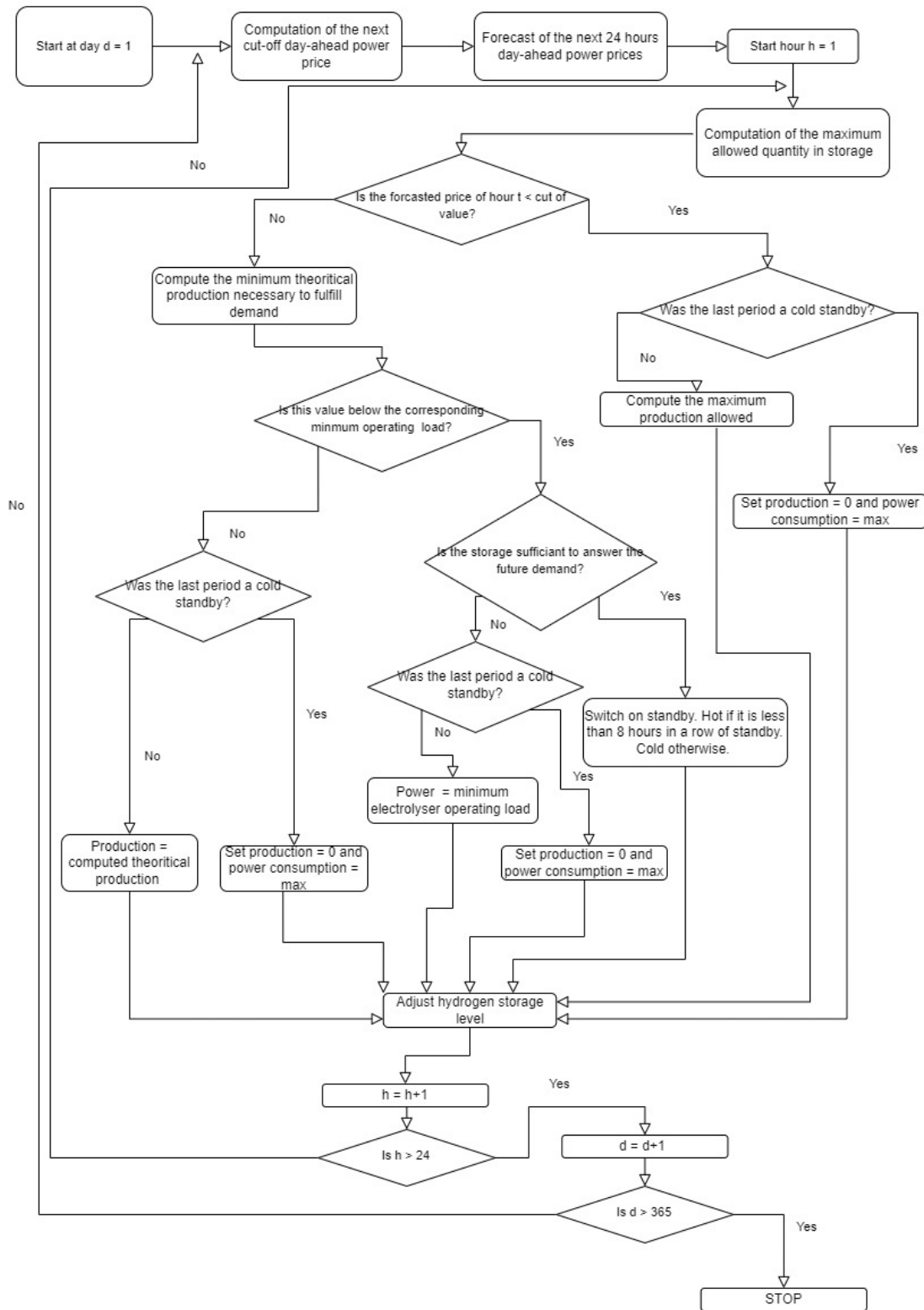
Figure 17: AEL Bidding Strategy diagram
