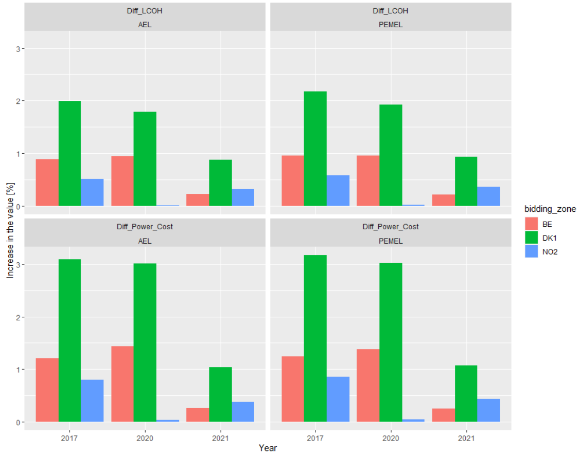
Figure 23: Increase in the Levelized Cost of Hydrogen and in the Power Cost [%] caused by forecasts
