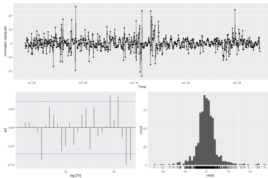
Figure 43: Residuals Western Denmark
