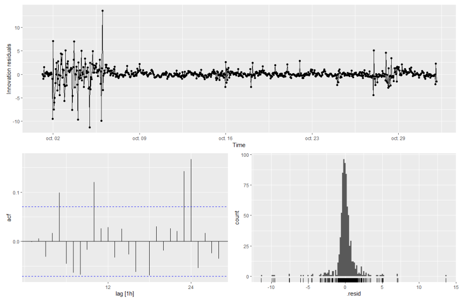
Figure 42: Residuals Southern Norway
