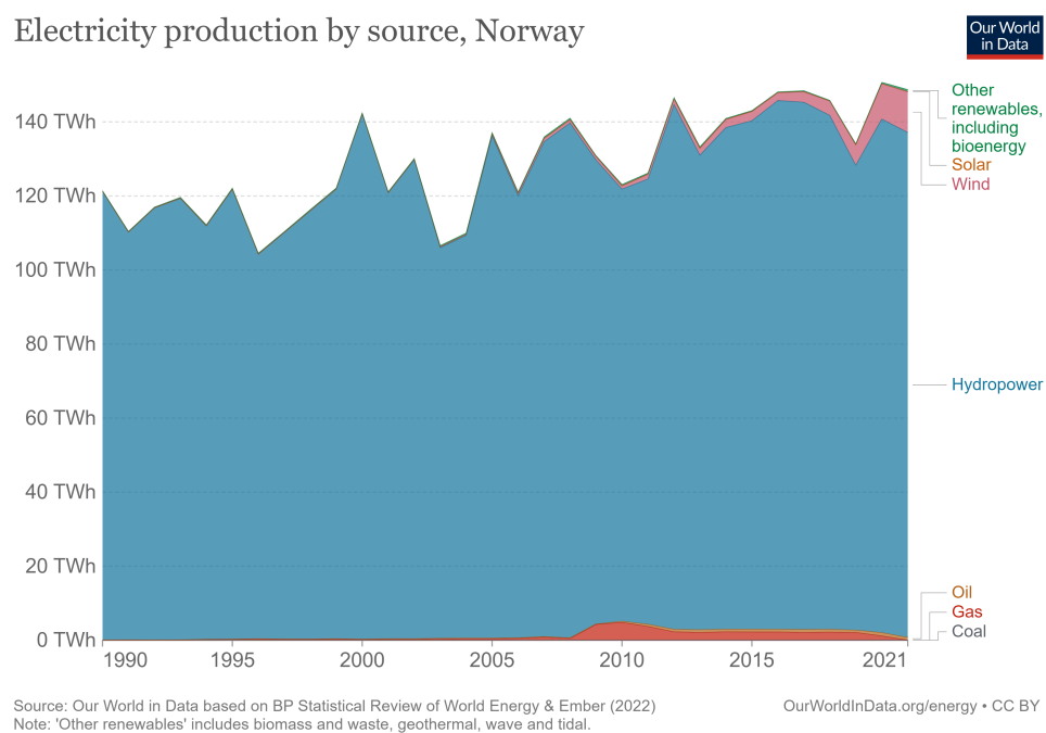
Figure 31: Norway electricity generation mix [58]
