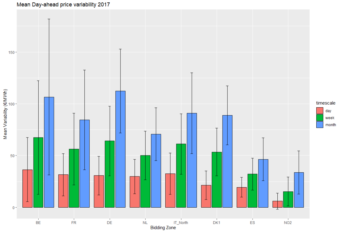
Figure 6: Daily, weekly and monthly mean variability
