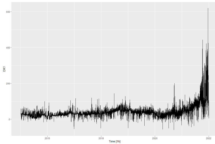
Figure 35: DK1 day-ahead power prices [€/MWh]
