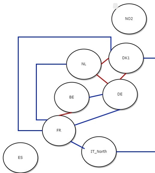
Figure 30: Monthly variability diagram
