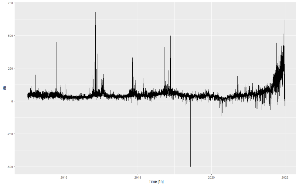
Figure 9: Belgian day-ahead power prices [€/MWh]
