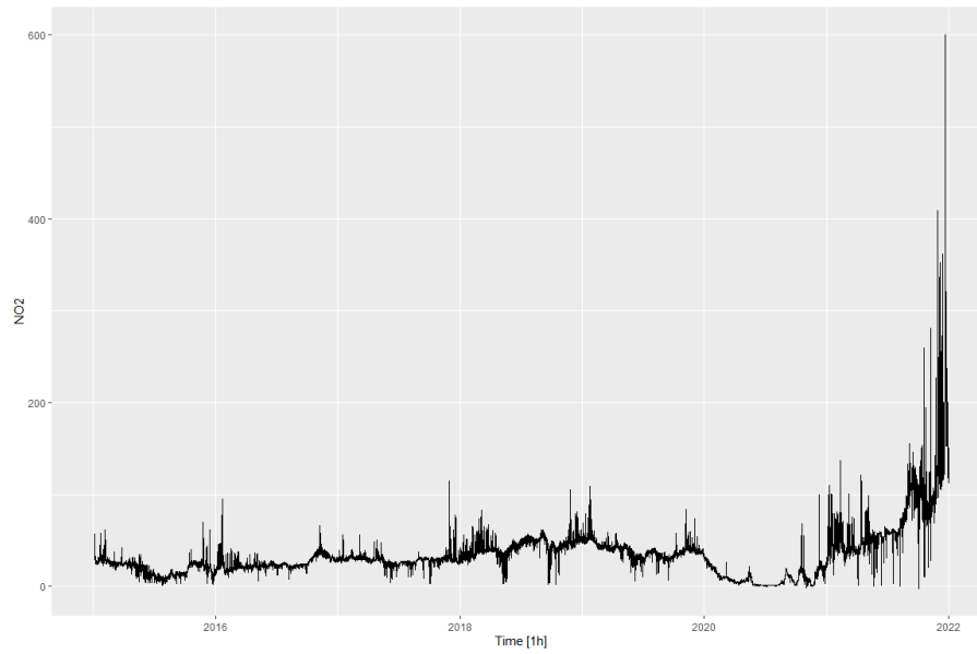
Figure 34: NO2 day-ahead power prices [€/MWh]
