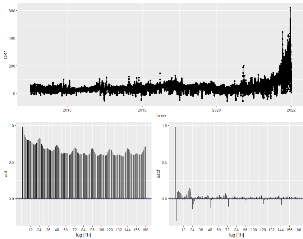
Figure 41: pACF Western Denmark
