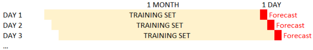
Figure 14: Simulation process
