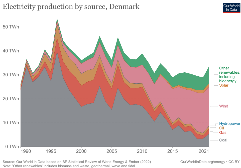
Figure 32: Denmark electricity generation mix [58]
