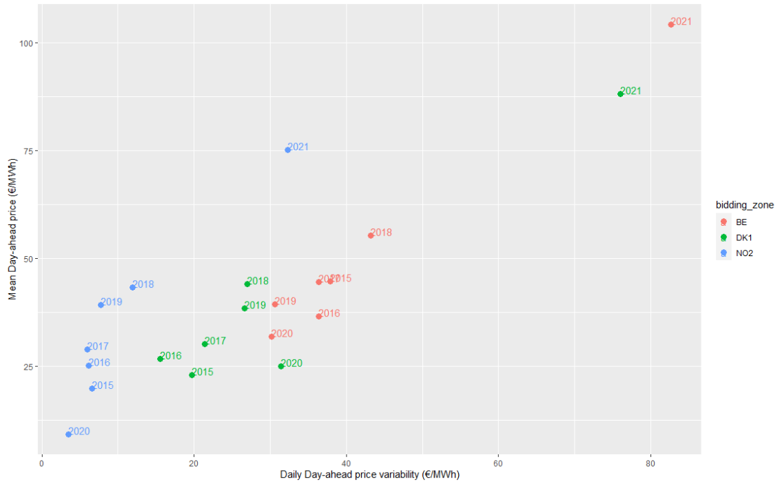
Figure 8: Mean day-ahead price and daily day-ahead price volatility
