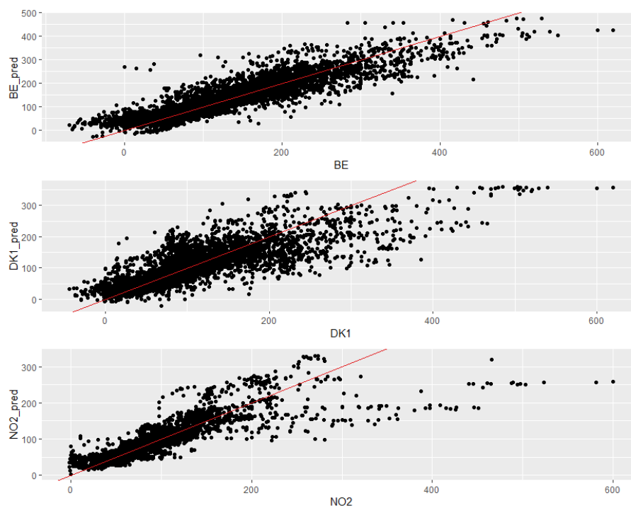
Figure 46: Year 2021
