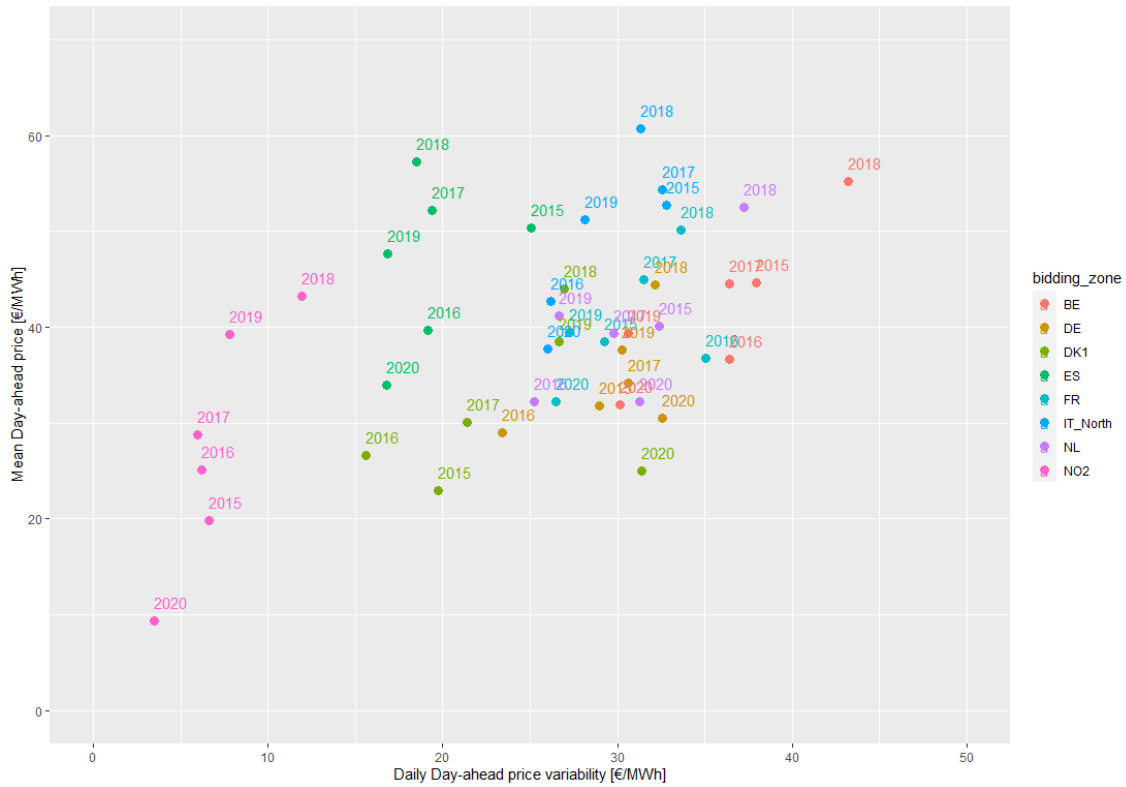
Figure 7: Mean day-ahead price and daily day-ahead price volatility
