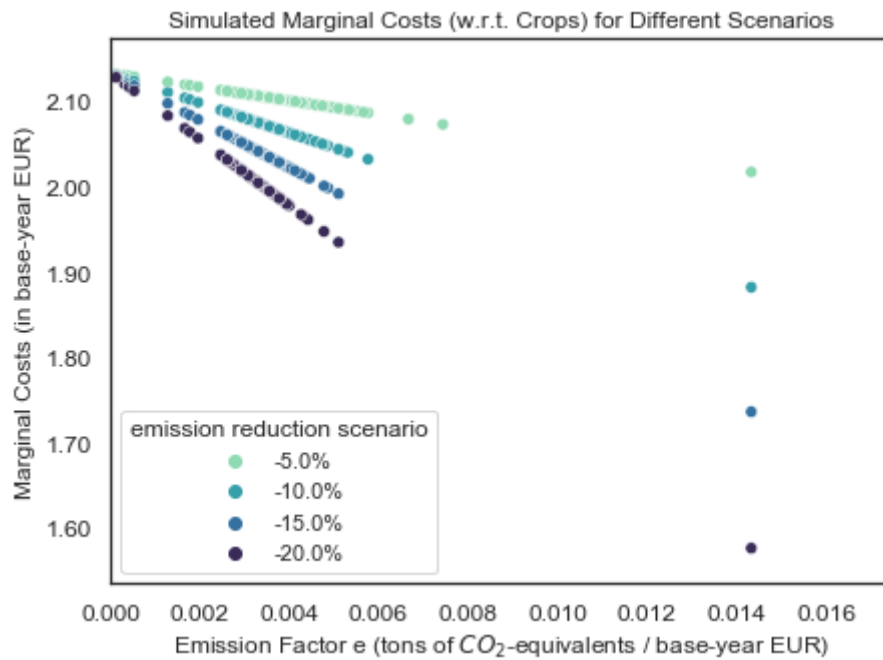
Figure A.20: Simulated marginal costs w.r.t. crop outputs for dairy farms, for four different emission reductions scenarios. Source: own visualization and simulation.
