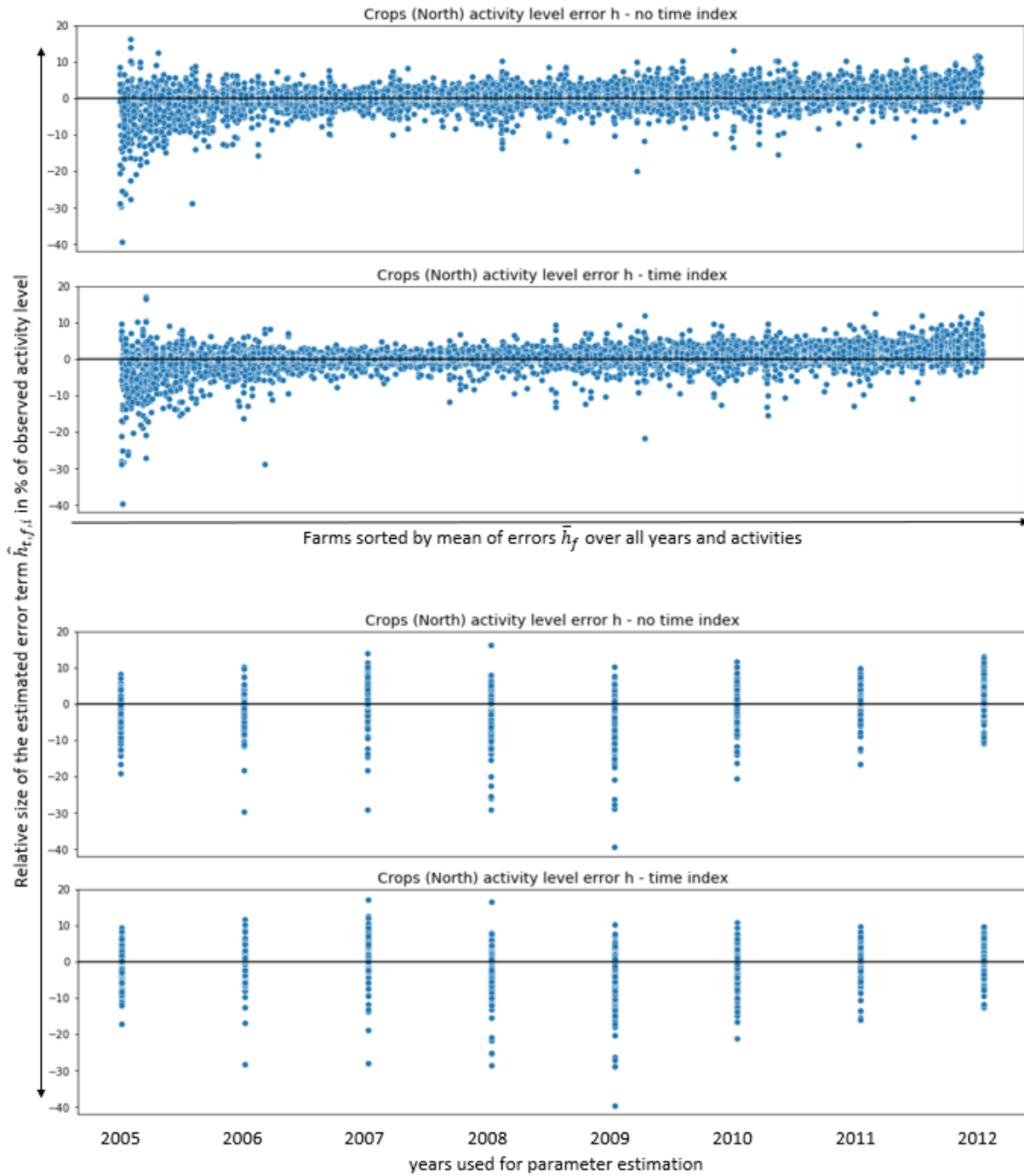
Figure A.8: Distribution of estimated activity level related error term \hat{h} for crop farms in northern Central France. Relative size of error term, measured in % of observed value. Activity level and fixed-input level dependent cost function with q_{\min ii} = 0.2 . Source: own simulation and visualization.
