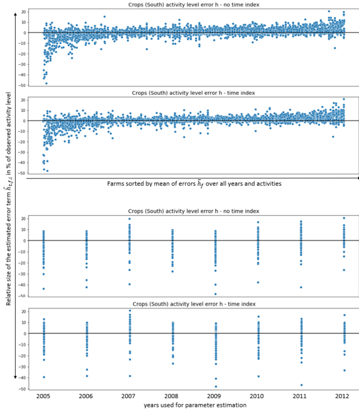
Figure A.5: Distribution of estimated activity level related error term \hat{h} for crop farms in southern Central France. Relative size of error term, measured in % of observed value. Activity level and fixed-input level dependent cost function with q_{\min_{ii}} = 0.2 . Source: own simulation and visualization.
