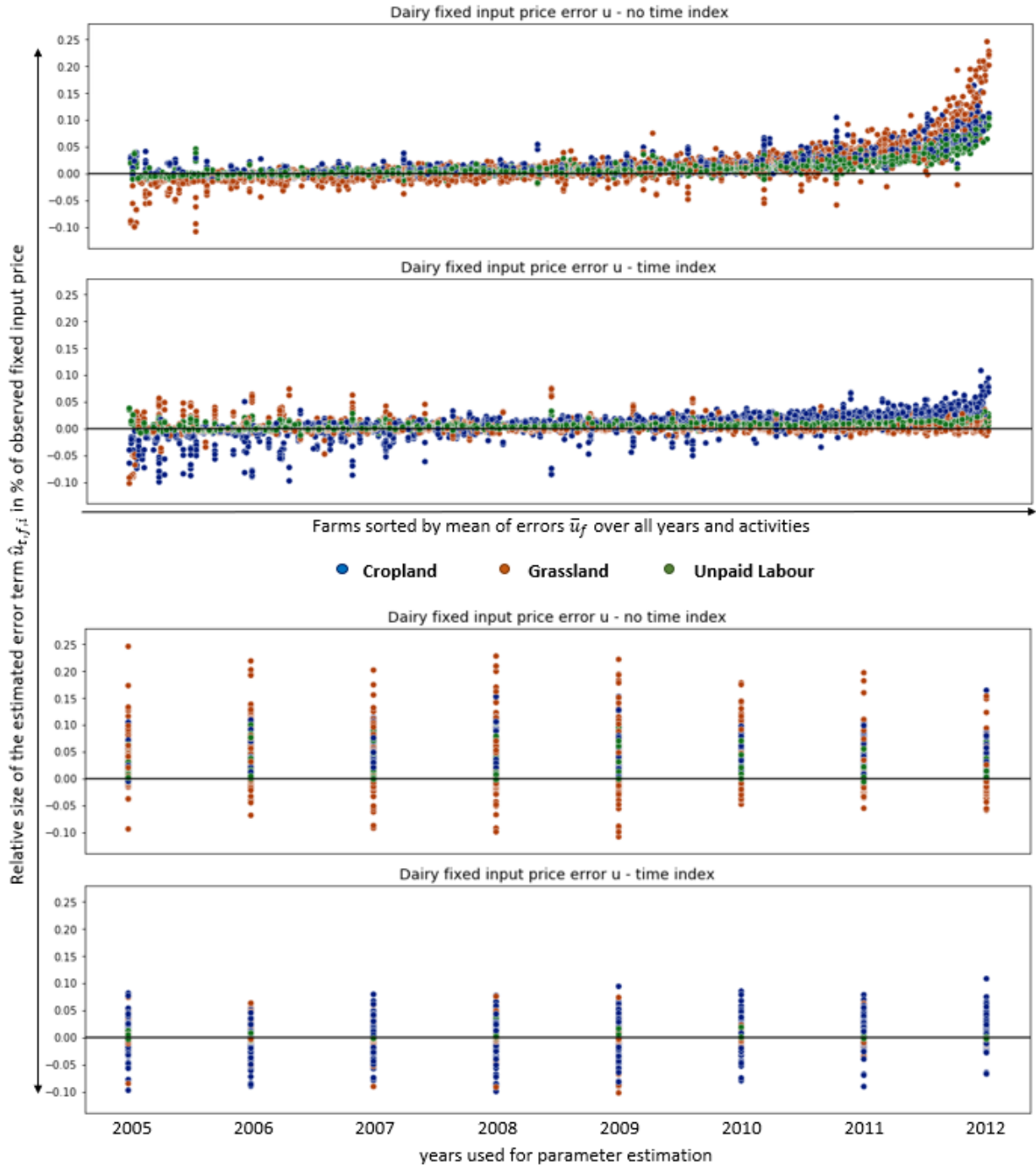
Figure A.12: Distribution of estimated fixed-input price related error term \hat{u} for dairy farms in West France. Relative size of error term, measured in % of observed value. Activity level and fixed-input level dependent cost function with q_{\min i} = 0.2 . Source: own simulation and visualization.
