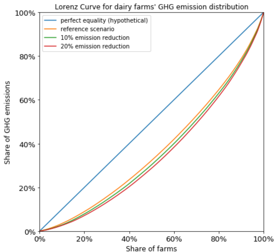
Figure 13: Lorenz curve indicating that emissions become more unevenly distributed if an emission cap is imposed. Source: own simulation and visualization.
