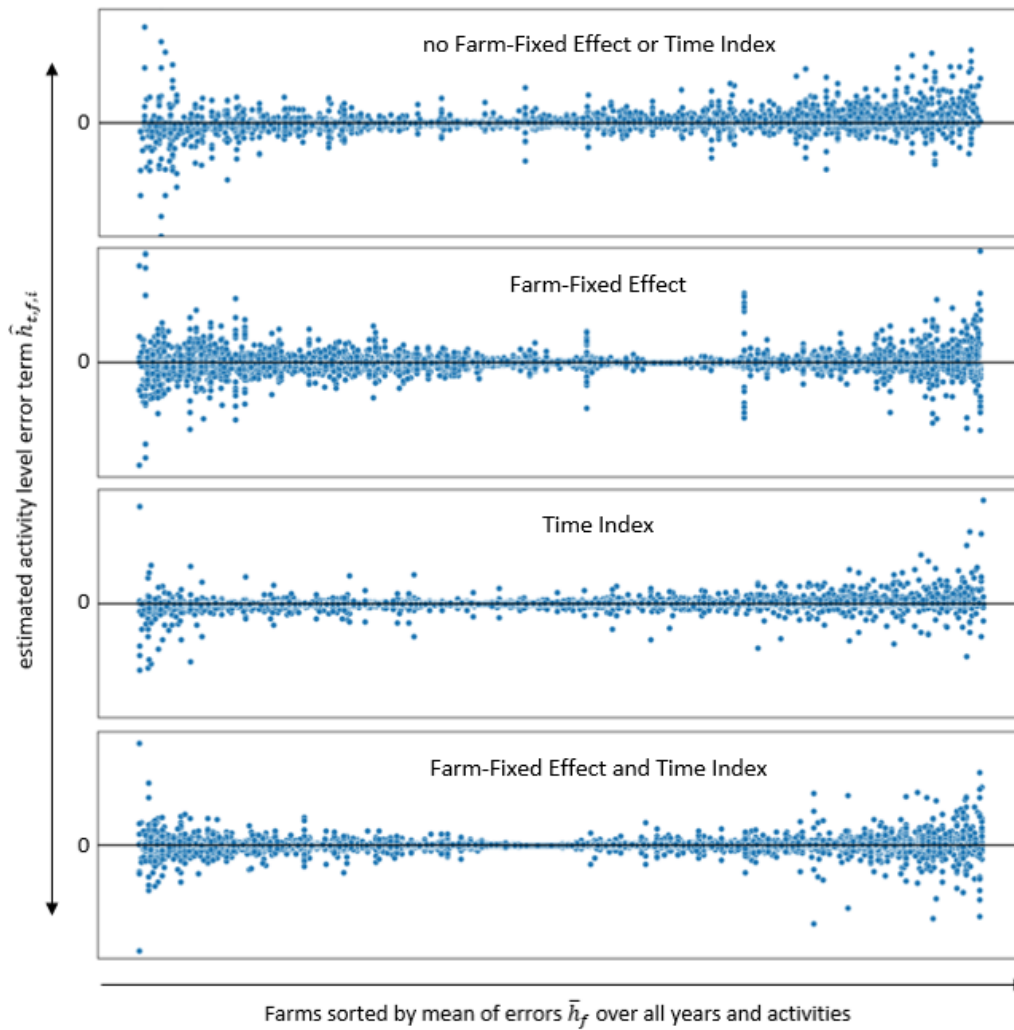
Figure 6: Estimated activity-level error terms \hat{h}_{t,f,i} per farm. Estimation for crop farms in southern Central France for different specifications of the activity-level cost function. Source: own visualization.
