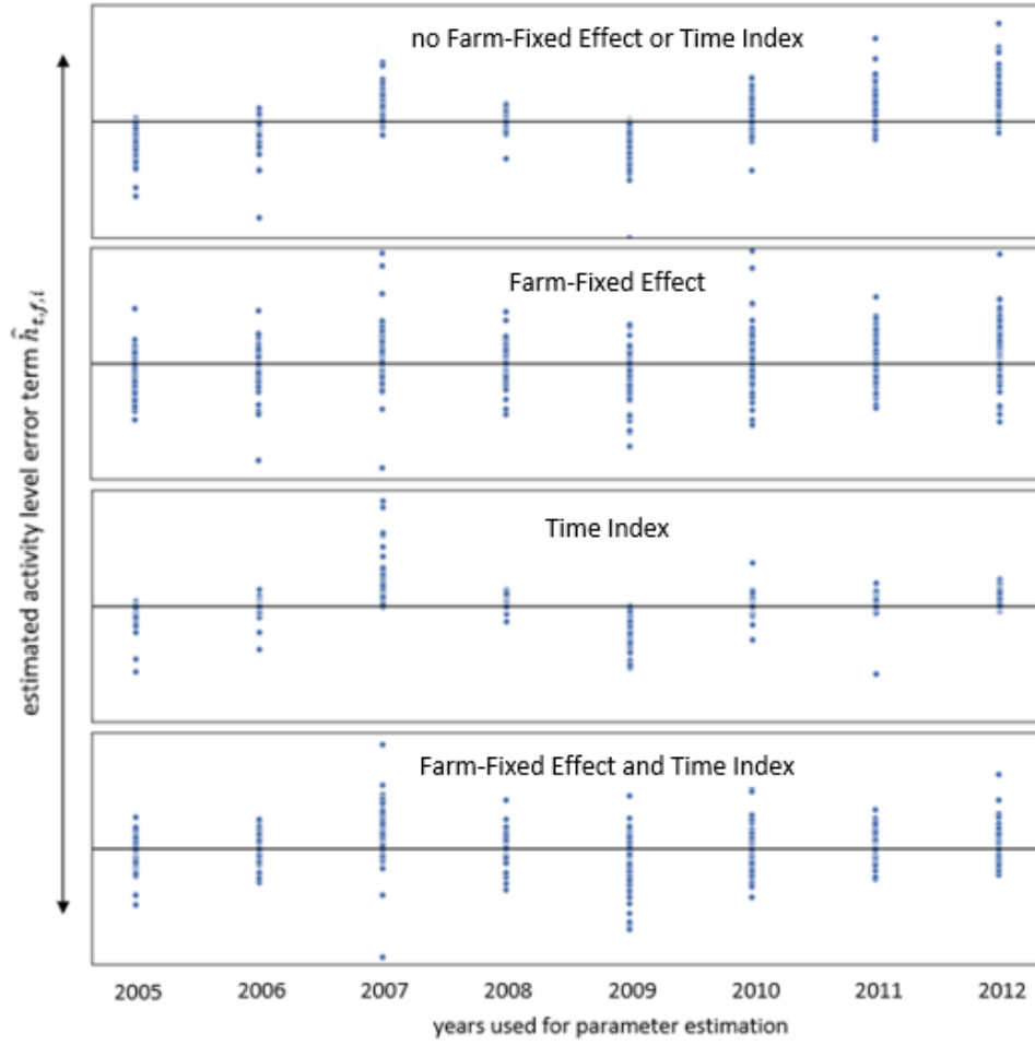
Figure 7: Estimated activity-level error terms \hat{h}_{t,f,i} per year. Estimation for crop farms in southern Central France for different specifications of the activity-level cost function. Source: own visualization.
