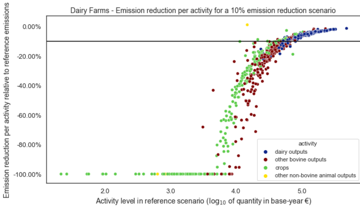
Figure A.22: impact of activity level in reference scenario on the emission reduction for a 10% emission cap. Source: own visualization and simulation.
