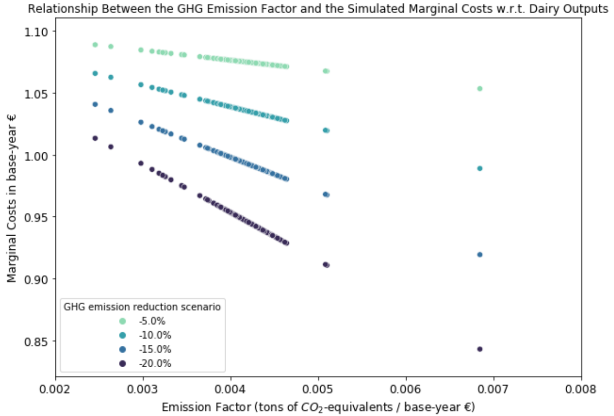
Figure 10: Simulated marginal costs with respect to dairy outputs for each of the dairy farms from West France, represented by the respective GHG emission factor e_{t,f,dairy} . Four different emission reduction scenarios are displayed. Source: own simulation and visualization.
