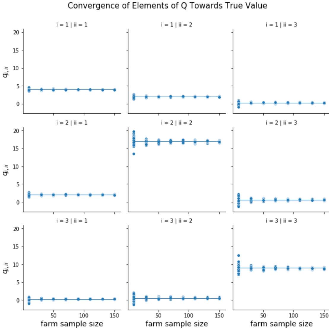
Figure 4: Convergence of estimates for the elements of matrix Q towards their true values with increasing sample sizes. Note that matrix Q is a quadratic, positive (semi-) definite matrix and therefore its elements q_{i,ii} = q_{ii,i} . Each dot represents an estimate \hat{q}_{r,i,ii} . The blue horizontal line indicates the true value of the element q_{i,ii} . Source: own calculations and visualizations.
