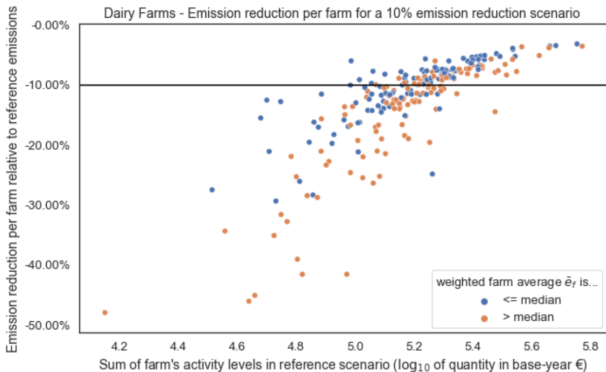
Figure A.23: Dairy farm's emission reduction for an emission cap of 10% compared to the reference scenario. Farms that lie above the black line are net emission right buyers, whereas the farms below the line are net sellers of emission rights. Source: own visualization and simulation.
