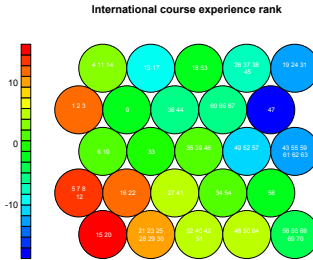
Figure 4.34: SOM coloured with International students (11).
