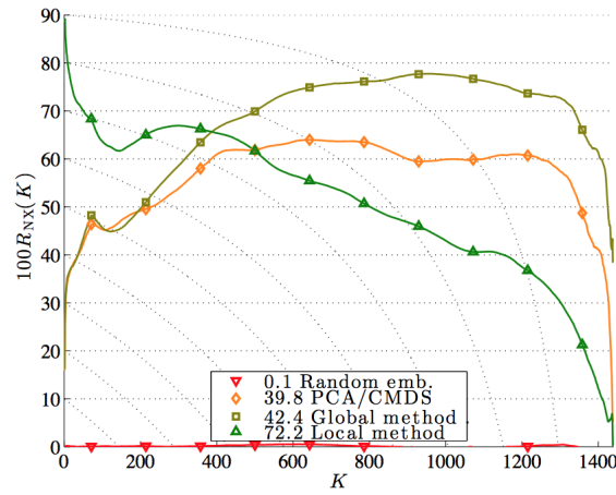
Figure 4.4: Examples of R_{NX}^K [27].
