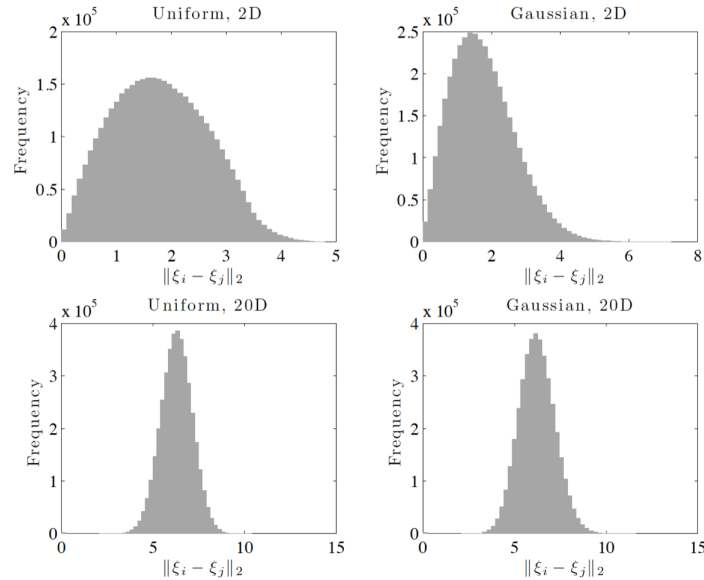
Figure 3.3: Phenomenon of norm concentration. The two left plots represent a uniform distribution in 2D and 20D. The two right plots display a gaussian distribution in 2D and 20D [27].
