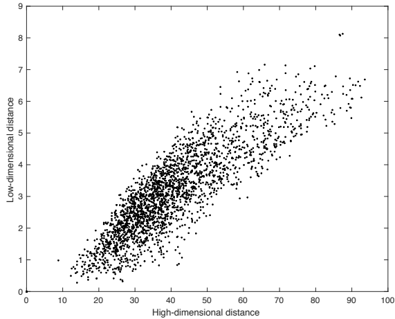
Figure 4.12: Shepard diagram of the projection in 3D using weighted reversed PCA.
