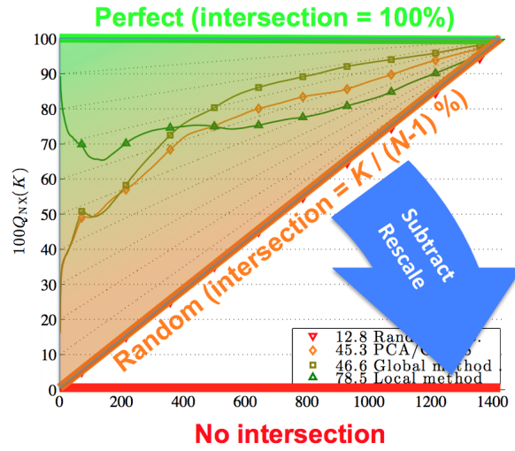
Figure 4.3: Transformation from Q_{NX}^K to R_{NX}^K [27].
