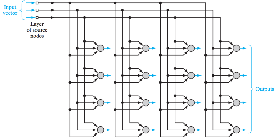
Figure 3.1: Two-dimensional lattice with a three-dimensional input and four-by-four dimensional output [19].
