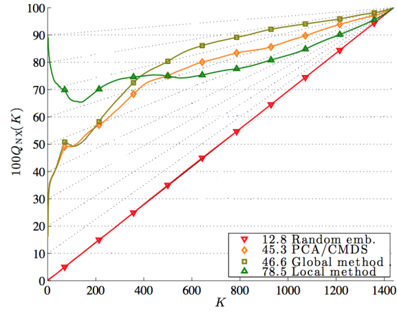
Figure 4.2: Examples of Q_{NX}^K [27].
