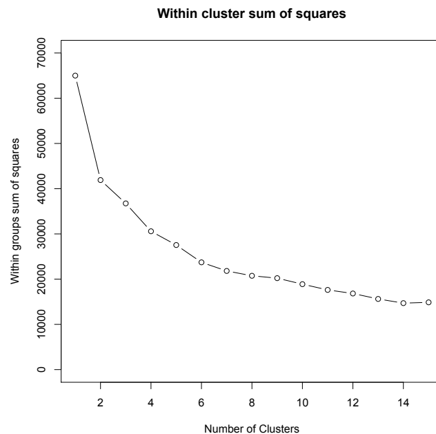
Figure 4.17: Within groups sum of squares relative to the number of clusters dividing the SOM nodes.
