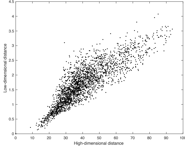
Figure 4.1: Example of a Shepard diagram.
