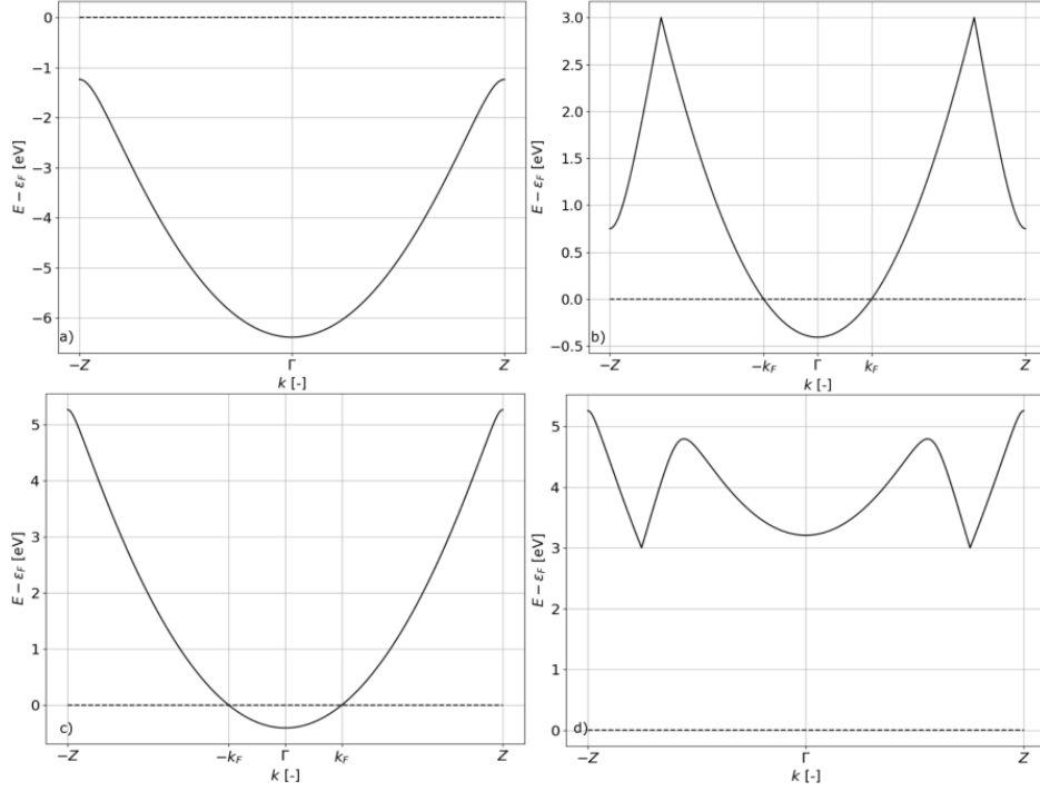
Figure B.2: Electronic bands of aluminum monoatomic chain. In panel a) band 1 is represented, in b) 2, c) 3 and d) 4. The Fermi level is represented in all the plots with a dashed line.
