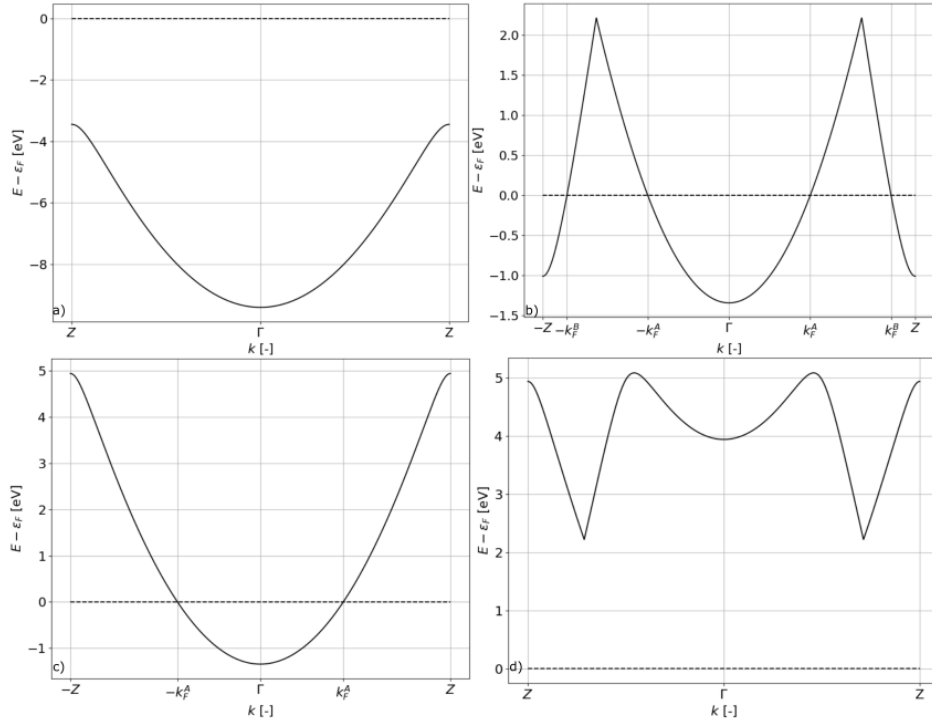
Figure B.1: Electronic bands of silicon monoatomic chain. In panel a) band 1 is represented, in b) 2, c) 3 and d) 4. The Fermi level is represented in all the plots with a dashed line.
