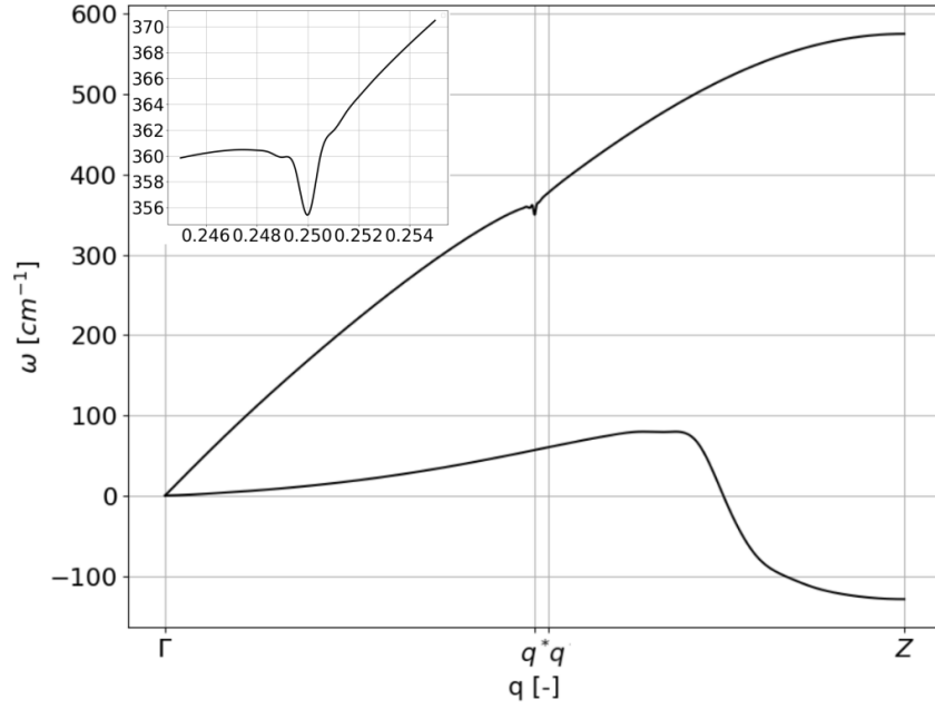
Figure 2.15: Phonon dispersion relation for an aluminum nanowire. The smearing temperature is 1 \times 10^{-5} Ha, the q mesh is composed of two-hundred equally-distanced points. In the inset, a zoom around the softening of the mode is shown with the curve sampled with a grid composed by twice as many points.
