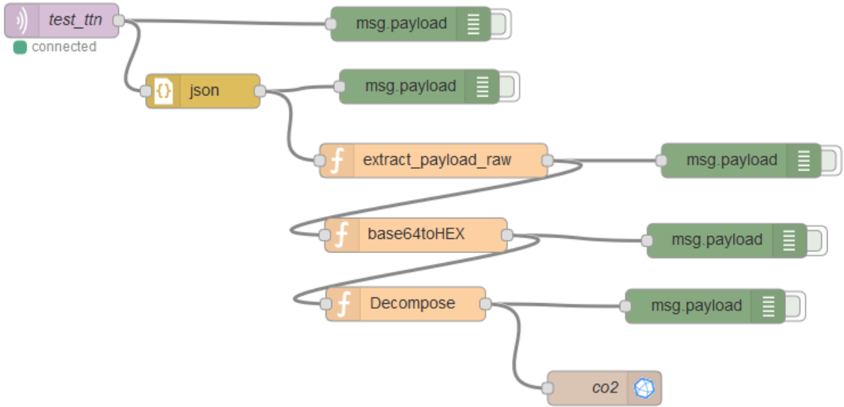
Figure 1.4: The wiring done in Node-Red for one sensor.
