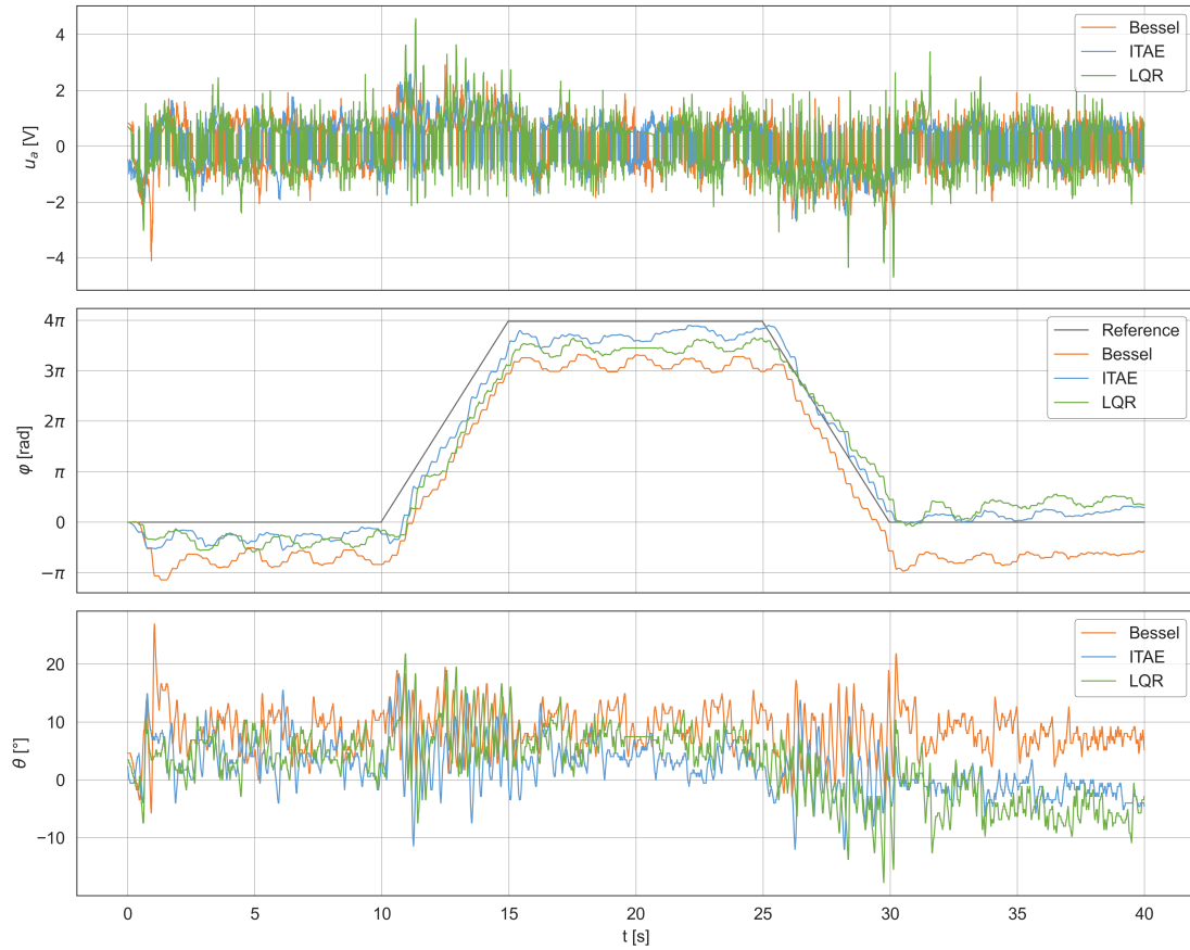
Figure 3.8: Experimentation of voltage response u_a(t) , wheel rotation angle \varphi(t) , and angular position \theta(t) over a 40-second test period under Bessel, ITAE and LQR control methods.
