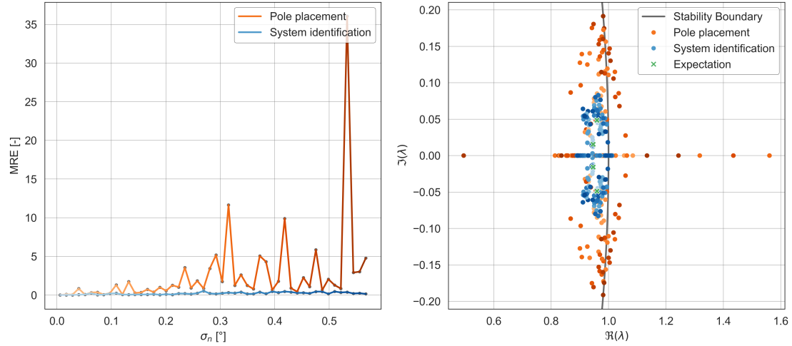
Figure 4.5: Simulation results depicting the Mean Relative Error (MRE) and pole positions under varying noise standard deviations \sigma_n , analyzed using pole placement and system identification methods with external input.
