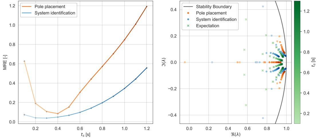
Figure 4.7: Simulation results depicting the Mean Relative Error (MRE) and pole positions under varying pole locations, analyzed using pole placement and system identification methods with external input.
