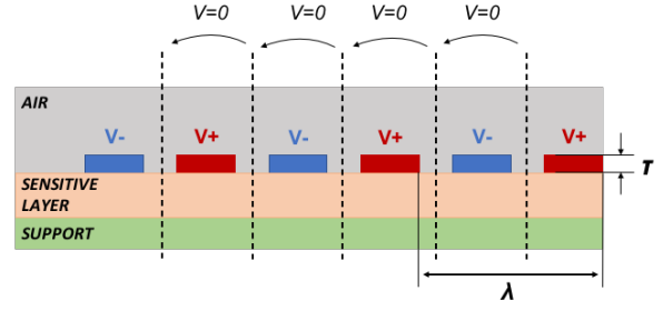
Figure 3.6: Cross-section of an IDE structure with equipotential planes
