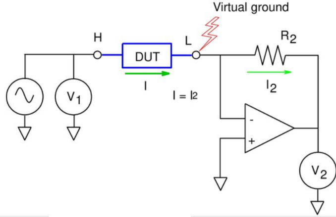
Figure 3.16: Auto balancing bridge main components. [204]
