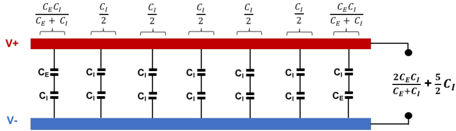
Figure 3.8: Reorganisation of the capacitances on figure 3.7 between the two electrodes
