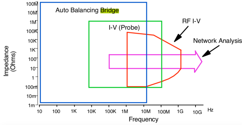
Figure 3.15: Coverage of each impedance measurement technique considering frequency and DUT impedance criteria. [204]
