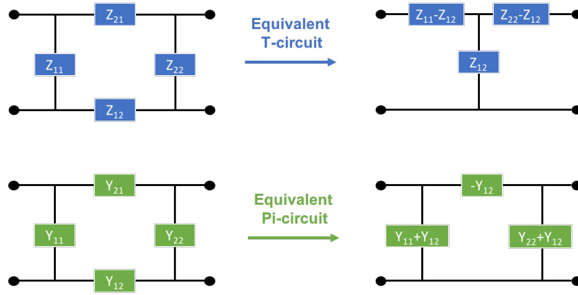
Figure 3.19: Equivalent T- and PI circuit for impedance and admittance parameters, given that the network is reciprocal.
