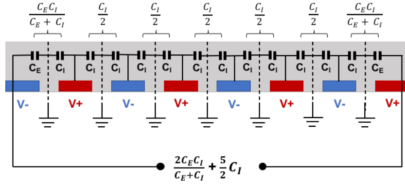
Figure 3.7: Equivalent circuit for evaluation of the semi-infinite top layer
