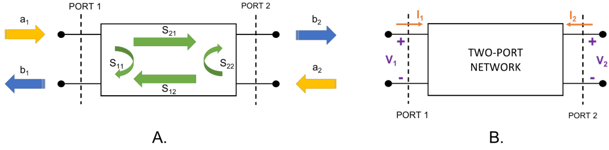
Figure 3.18: Schematisation of S-parameters (A.) and general representation of a two-port network (B.)
