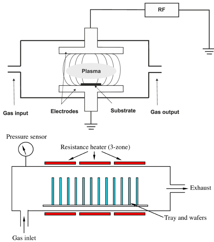
Figure 1.21: Schematic representation of a Plasma Enhanced CVD reactor chamber [133] and a Low Pressure CVD [134]
