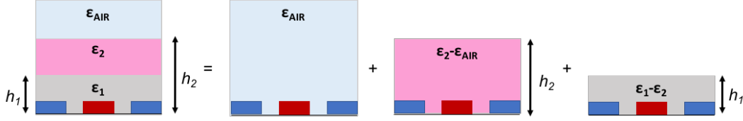
Figure 3.10: The partial capacitance technique: splitting up a two-layered half plane into two individual layers and the infinite air-layer
