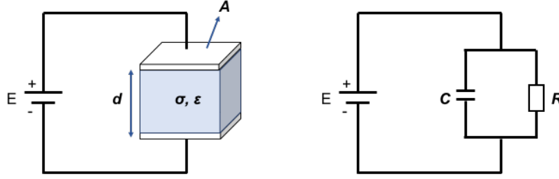
Figure 3.3: Dielectric medium between two parallel plates and its equivalent circuit.
