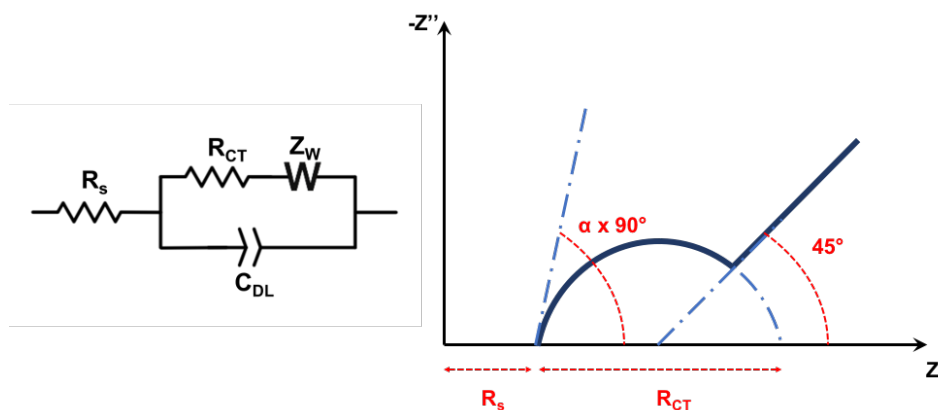
Figure 1.18: General Randles circuit and corresponding Nyquist plot. \alpha is defined in figure 1.17
