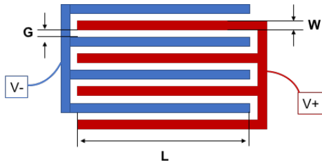
Figure 3.5: Electrode plane
