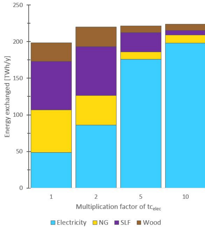
Figure 4.14: Evolution of energy exchanged by each carrier with the increase of electrical transfer capacities ( tc_{elec} ).
