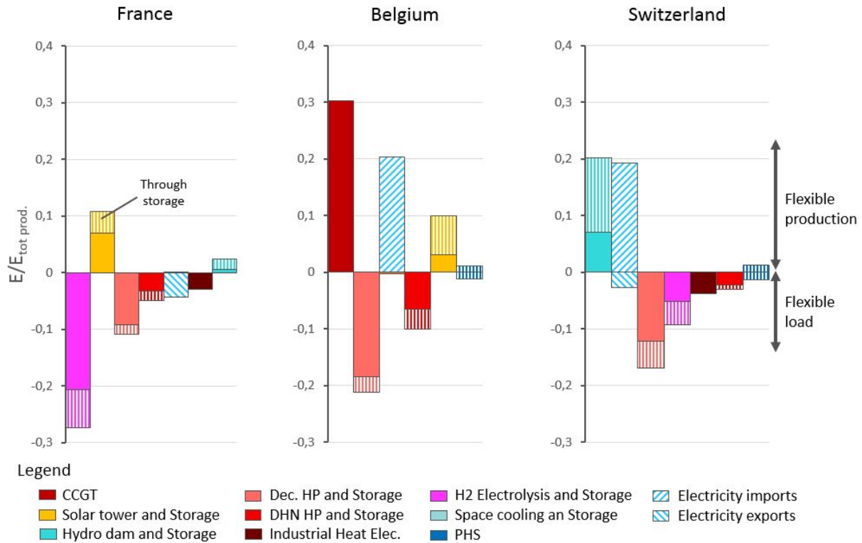
Figure 4.7: Share of the flexibility providers and their storage into the electricity production and consumption mix. (abbrev.:
