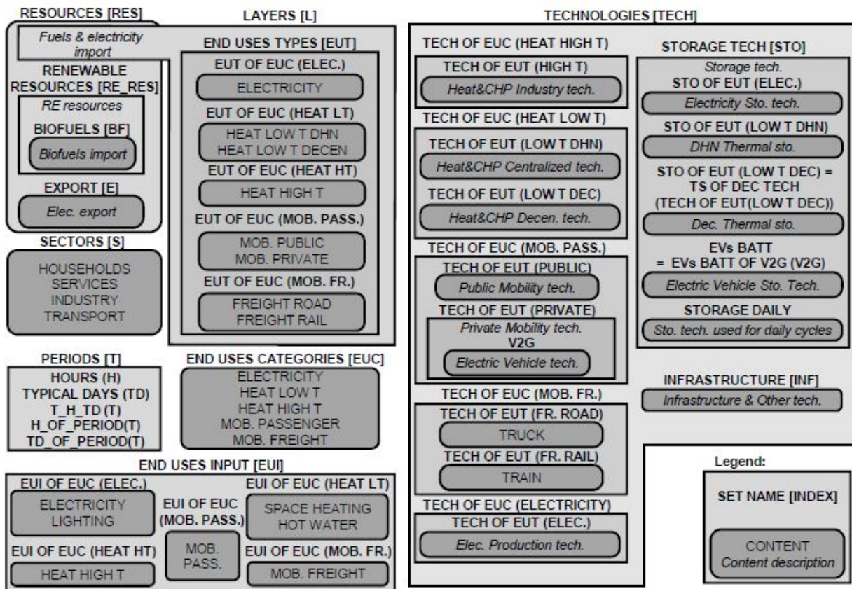
Figure A.4: Visual representation of the sets and indices of the LP framework. Abbreviations: space heating (SH), hot water (HW), temperature (T), mobility (MOB), vehicle-to-grid (V2G), thermal storage (TS).[27]
