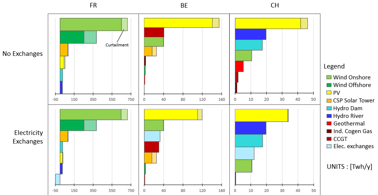
Figure 3.1: Comparison of electricity production mix of the different cells in the scenarios : no exchanges and electrical exchanges. (abbrev.: France (FR), Belgium (BE), Switzerland (CH), photovoltaic panels (PV), concentrated solar power (CSP), industrial cogeneration (Ind. Cogen) combined cycle gas turbine (CCGT), electricity (Elec.))
