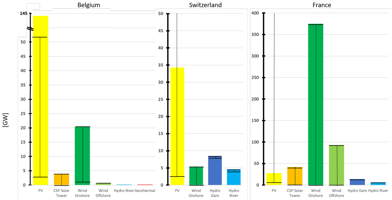
Figure C.2: Installed renewable assets of each country and their maximum and minimum potential (horizontal black line) (abbrev. : photovoltaic panels (PV))
