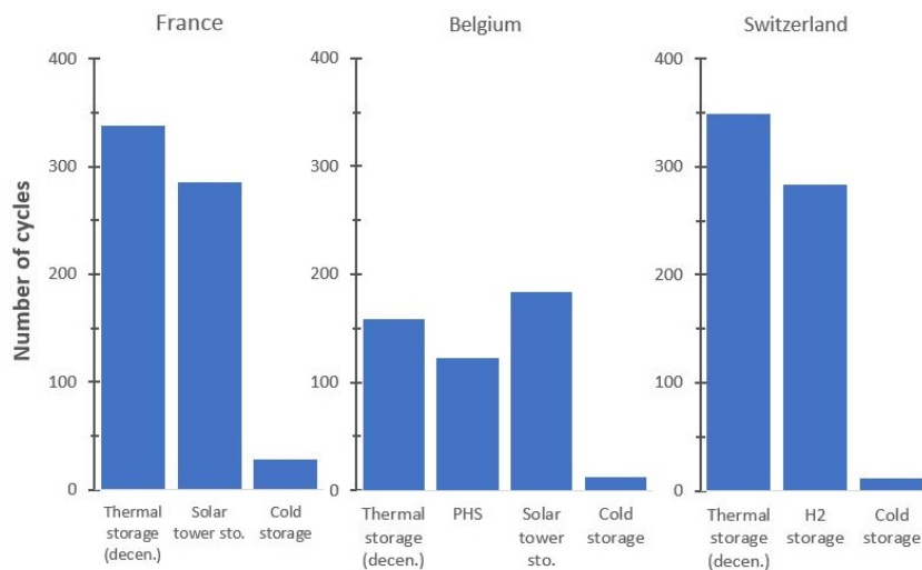
Figure 4.5: Number of equivalent cycles of daily storage in each country. (abbrev.: decentralised (decen.), storage (sto.), pumped hydro storage (PHS))
