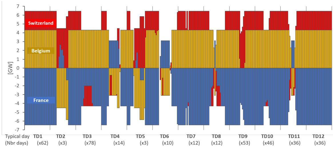
Figure 3.2: Verification of the balance of electricity exchanges between countries at each hour of each TD [GW].
