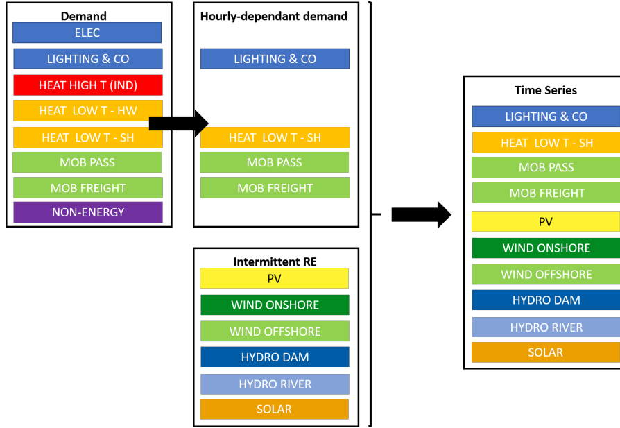
Figure 1.3: Existing time series in EnergyScope TD.
