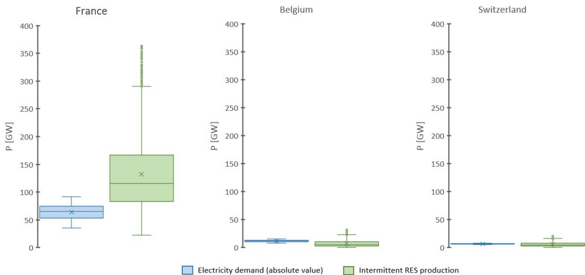
Figure 4.2: Quantitative statistics of the fixed electricity demand and the intermittent renewable energy (IRE) production.
