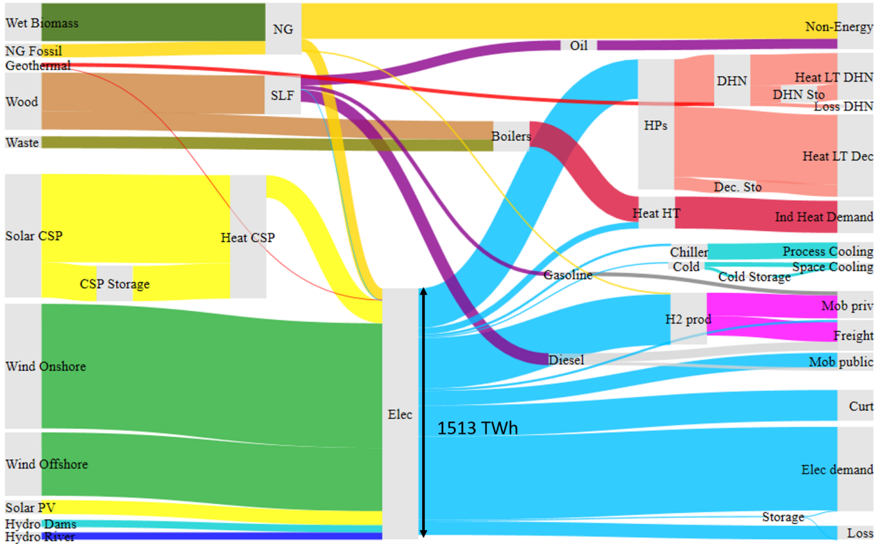
Figure E.1: Sankey diagram of the global system
