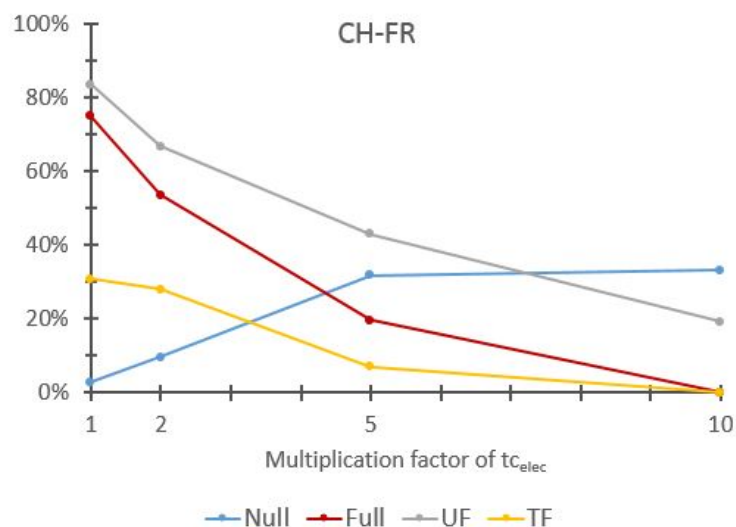
Figure 4.17: Evolution of the time spent at null and full capacity and of the utilisation factor (UF) and the transit factor (TF) of the CH-FR electrical line with the increase in electrical transfer capacities ( tc_{elec} ) size.
