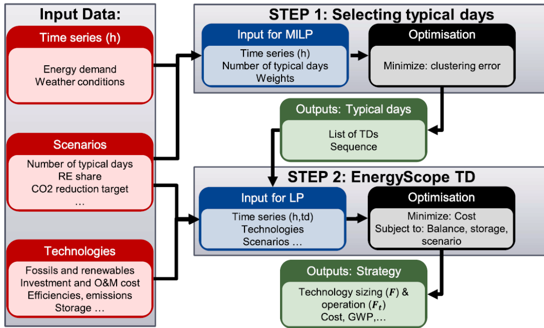
Figure 1.1: Structure of EnergyScope typical days (TD) [28]. (abbrev. : renewable energy (RE), operation and maintenance (O&M), mixed integer linear programming (MILP), linear programming (LP), global warming potential (GWP))
