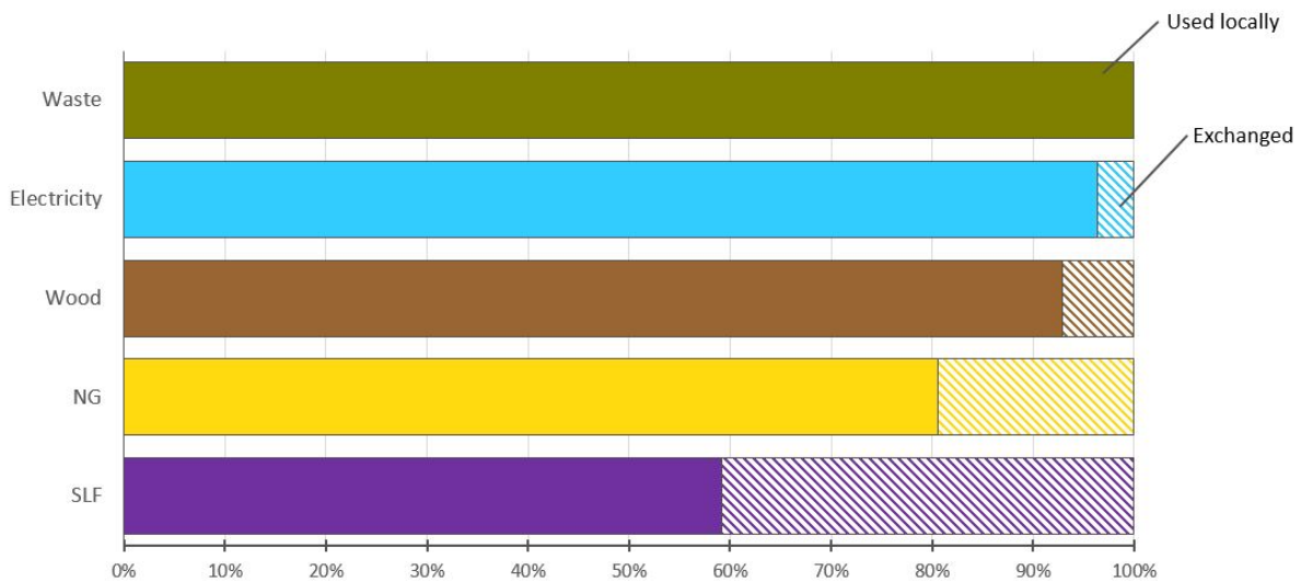
Figure 4.11: Share of resources exchanged and used locally for waste, electricity, wood, natural gas (NG) and synthetic liquid fuel (SLF).
