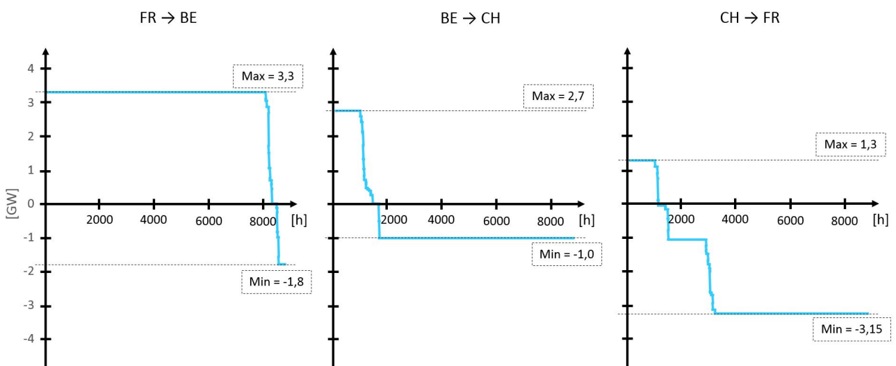
Figure D.4: Duration of electricity exchanges on each transmission line
