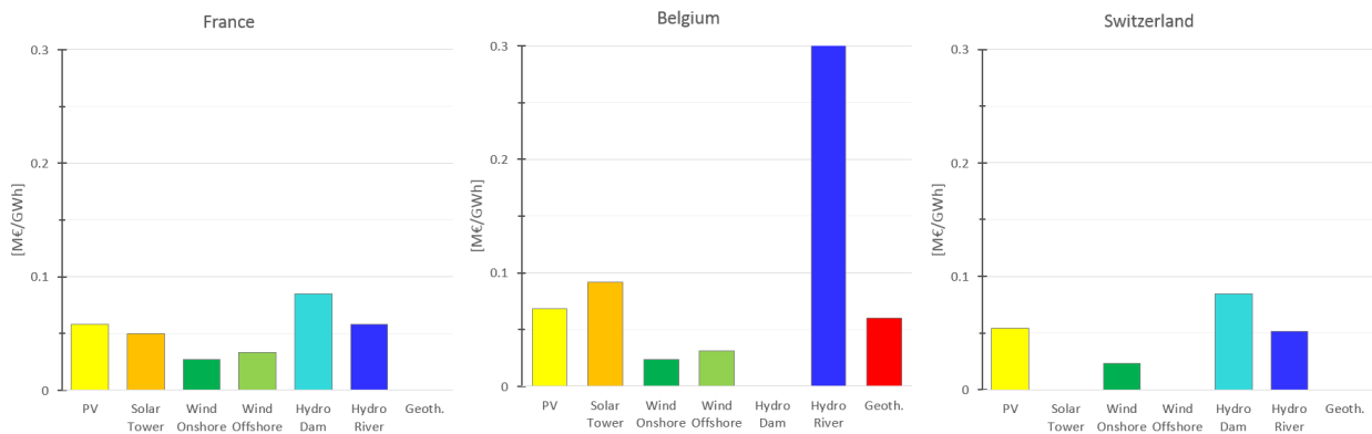
Figure C.3: Levelized Cost of Energy (LCOE) of the RES assets
