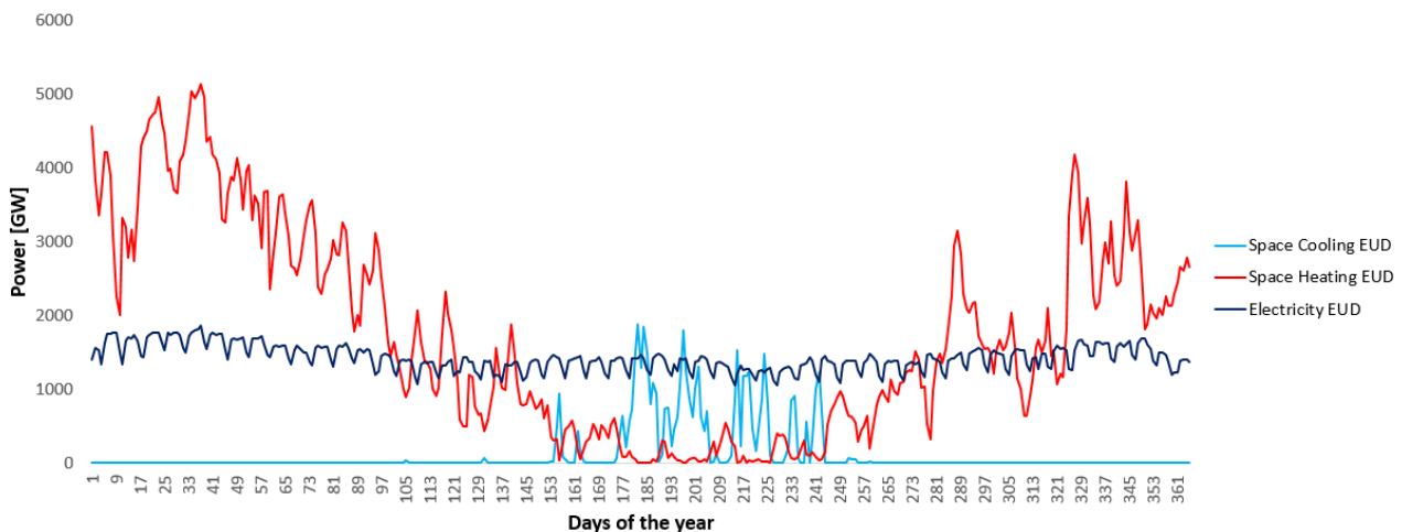
Figure 2.2: Variation of the daily electricity, space heating, and space cooling demand of the global system over the year (beginning on January 1st).
