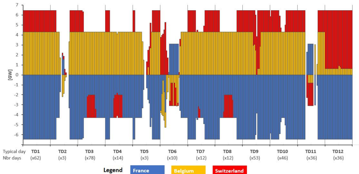
Figure 4.8: Verification of the balance of electricity exchanges between countries at each hour of each TD [GW]. A positive value means that the country imports and a negative value that it exports.
