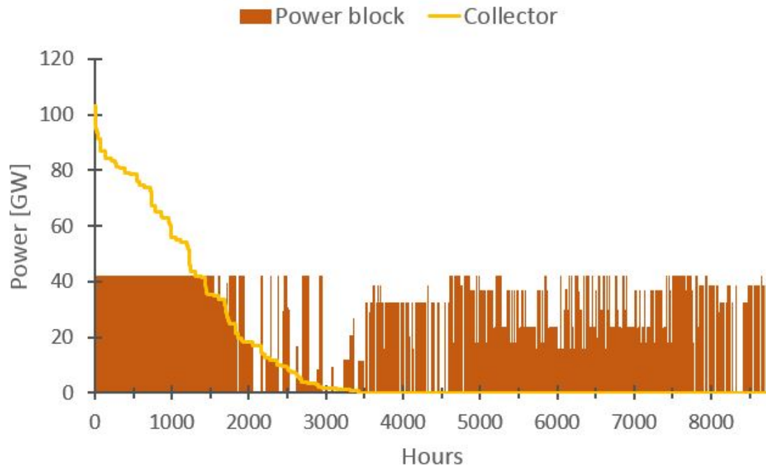
Figure D.3: Duration curve of solar tower resource and power output in France in the all exchange scenario
