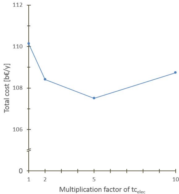
Figure 4.13: Evolution of the total annualised cost of the 3-cell system with an increase in transfer capacities of electrical lines ( tc_{elec} ). The increase is expressed as a multiplication factor of the 2020 transfer capacities (see Section 2.3.1).
