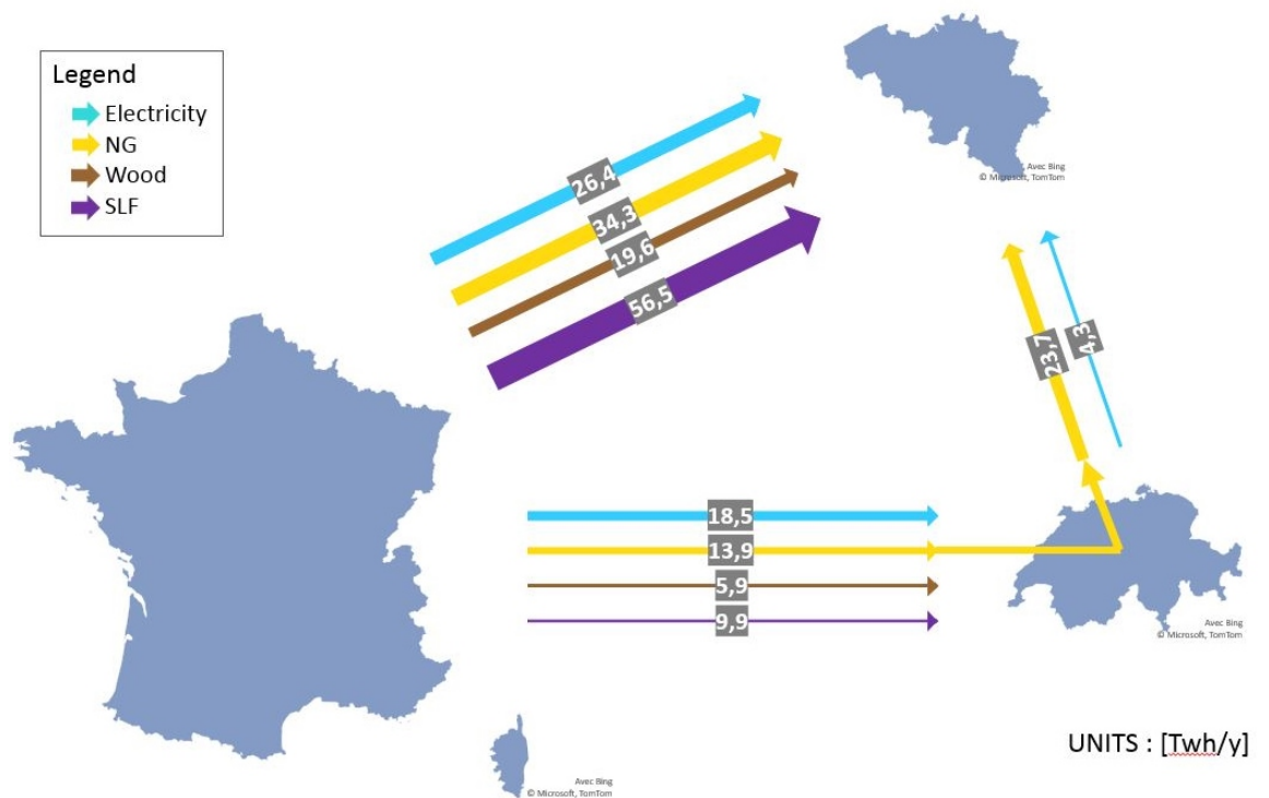
Figure 4.12: Yearly balance of exchanges for each interconnection [Twh/y].
