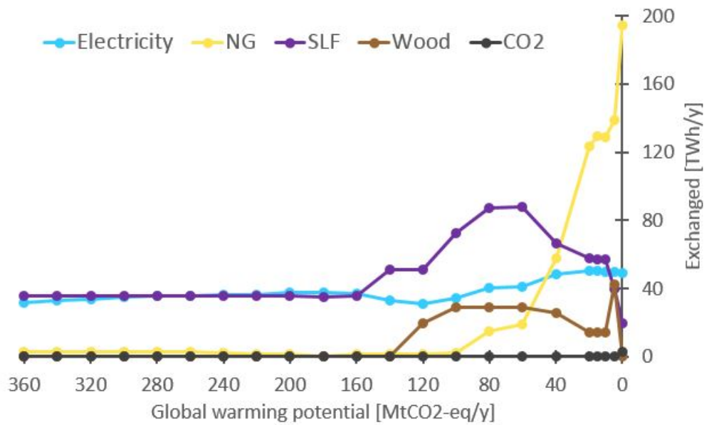
Figure 4.19: Evolution of exchanges during the energy transition of the 3-cell all exchanges scenario.
