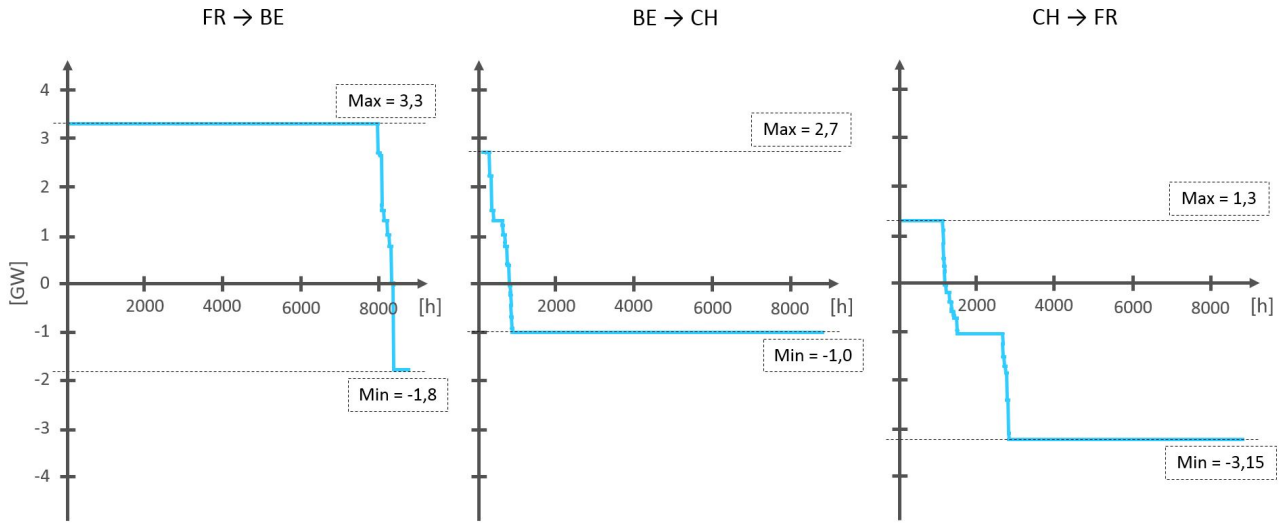
Figure 3.4: Load curve of electrical exchanges.
