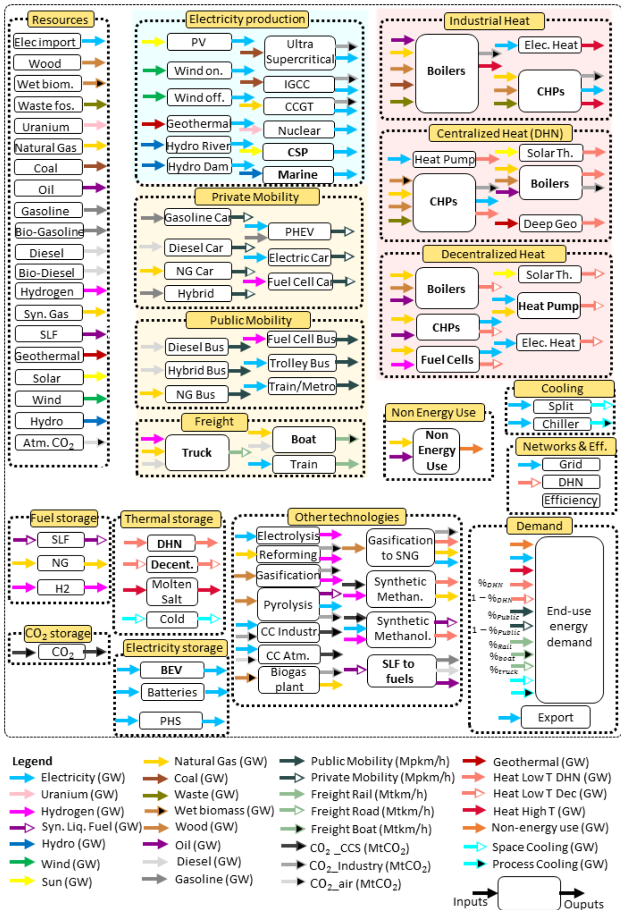
Figure A.8: Definition of all the resources, conversion technologies and EUD through the concept of layer Bold technologies represent groups of technologies with different energy inputs (e.g. Boilers include gas boilers, oil boilers, ...). Decent. represents the group of thermal storage for each decentralised heat production technology 82 [6][26]
