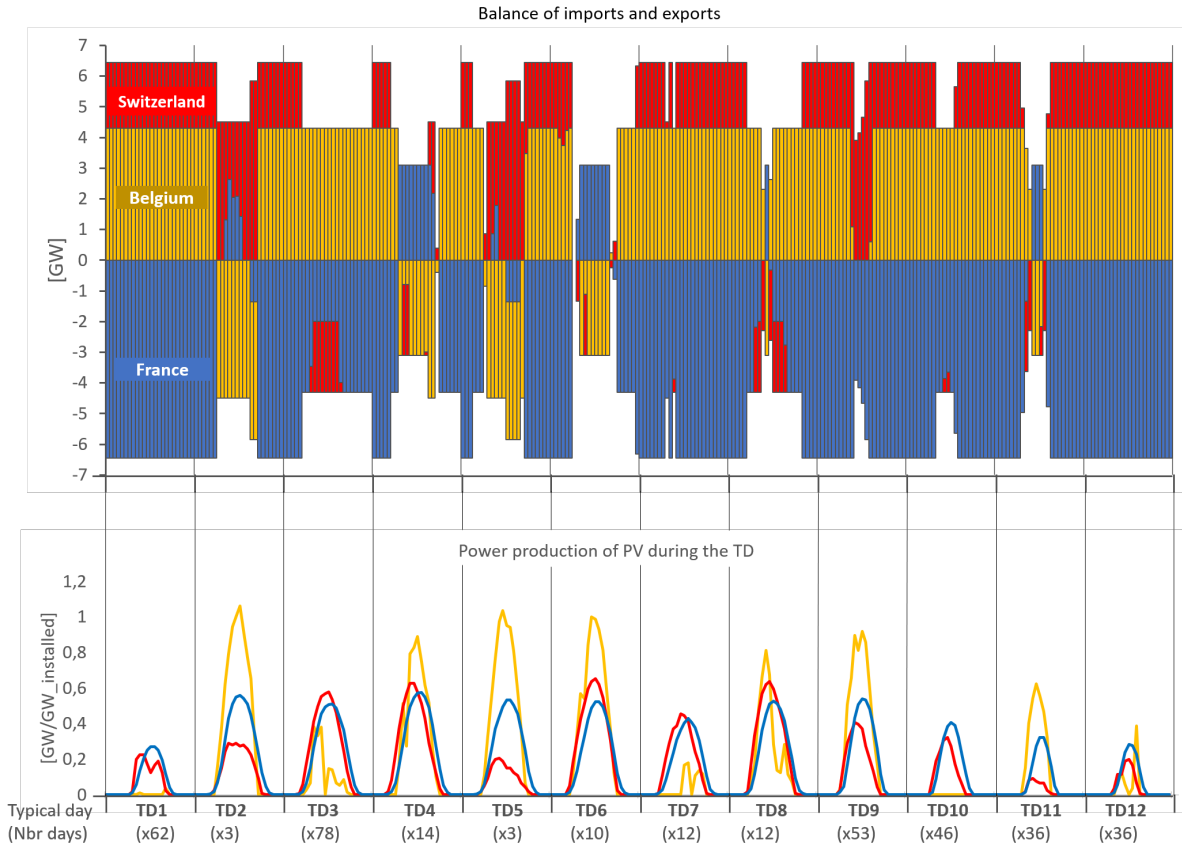
Figure 3.3: Relation between the hourly imports/exports and hourly coefficient of performance of PVs ( c_{pt,PV} ) in Switzerland and Belgium.
