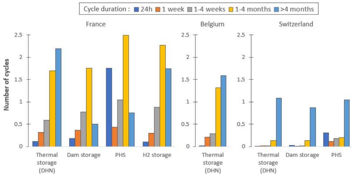
Figure 4.6: Number of equivalent cycles for mid-term and long-term storage in each country. (abbrev.: district heating network (DHN), pumped hydro storage (PHS))
