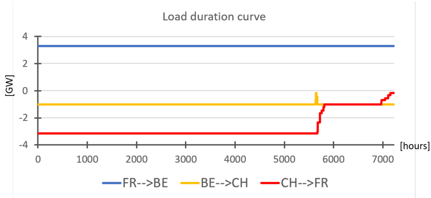
Figure 3.6: Duration curve of transmission lines in Case 1.
