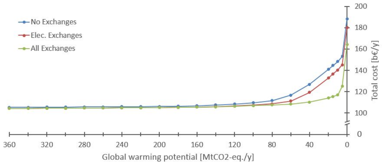
Figure 4.18: Pareto front of the cost-CO2 optima for the no exchanges, electricity exchanges and all exchanges scenarios.
