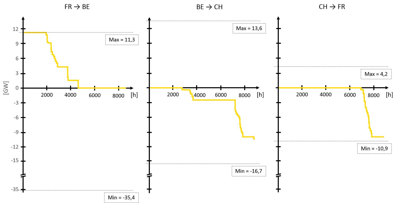
Figure D.5: Duration of natural gas (NG) exchanges on each transmission line
