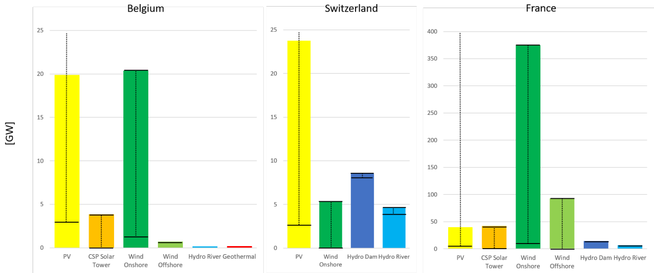
Figure E.2: RE Assets of Belgium, Switzerland and France
