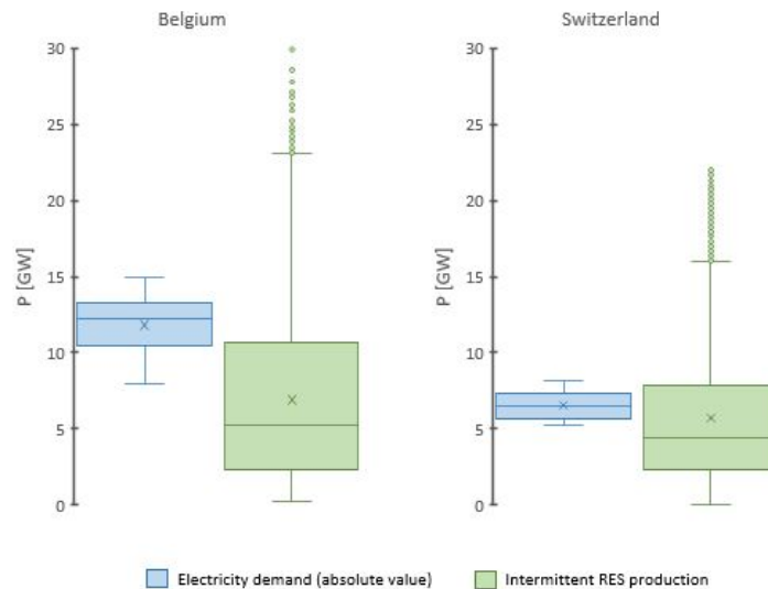
Figure 4.3: Quantitative statistics of the fixed electricity demand and intermittent renewable energy (IRE) production, a zoom on Belgium and Switzerland.
