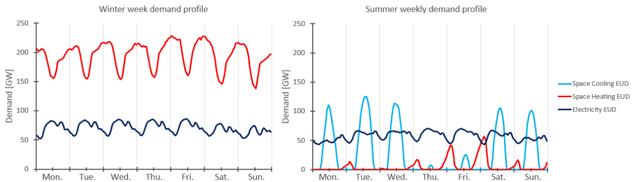
Figure 2.3: Weekly profile of electricity, space heating, and space cooling demand of the global system over the year.
