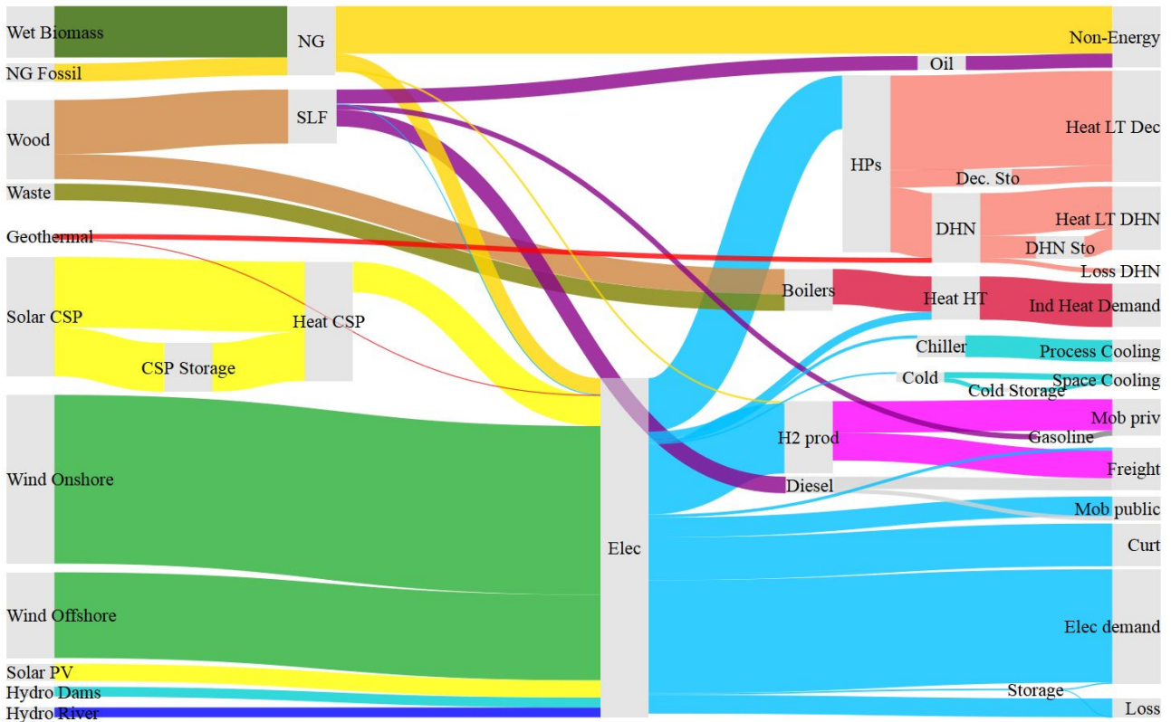
Figure 4.1: Energy flows in the overall system from primary energies (left side) to end-use demand (right side). (abbrev.: see list of abbreviations)
