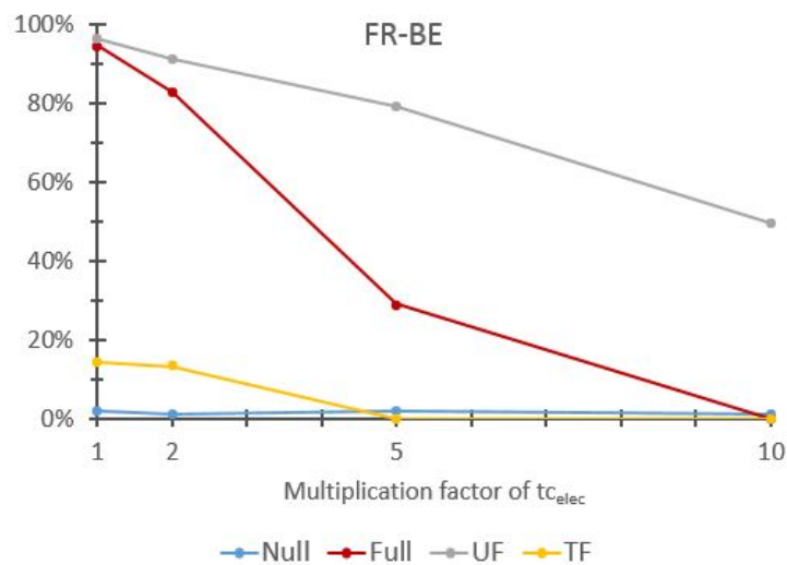
Figure 4.15: Evolution of the time spent at null and full capacity and of the utilisation factor (UF) and the transit factor (TF) of the FR-BE electrical lines with the increase in electrical transfer capacities ( tc_{elec} ) size.
