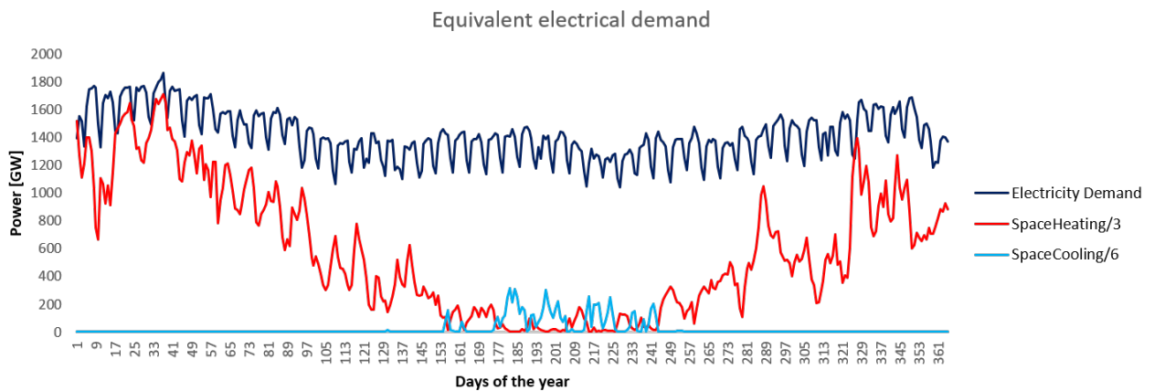
Figure B.2: Electricity, heating and cooling demand in equivalent electrical GW supposing a ratio of 3 for heat and a ratio of 6 for cold
