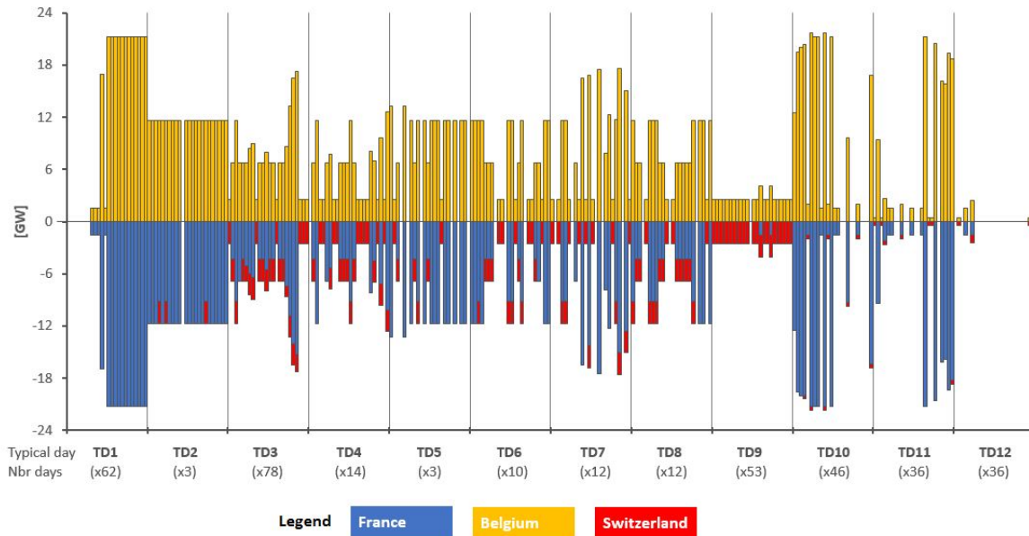
Figure 4.9: Verification of the balance of natural gas (NG) exchanges between countries at each hour of each TD [GW]. A positive value means that the country imports and a negative value that it exports.
