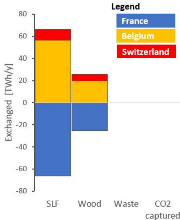
Figure 4.10: Verification of the balance of freight resources (synthetic liquid fuel (SLF), wood, waste and CO 2 captured) exchanged between countries on a yearly scale. A positive value means that the country imports and a negative value that it exports.
