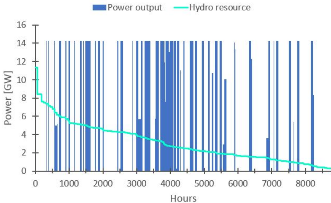
Figure D.2: Duration curve of hydro dam resource and power output in France in the all exchange scenario
