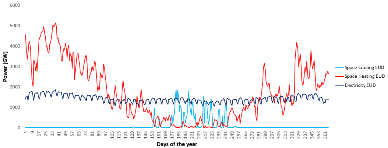
Figure B.1: Electricity, space heating, and space cooling demand of the global system
