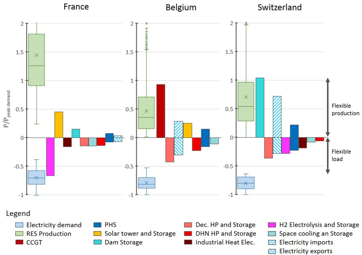
Figure 4.4: Power of flexible loads and flexible production assets compared to intermittent renewable energy sources (IRES) production and electricity demand, normalised by peak demand of the country. (abbrev. : combined cycle gas turbine (CCGT), pumped hydro storage (PHS), Decentralised (Dec.), heat pump (HP), district heating network (DHN), hydrogen (H2))
