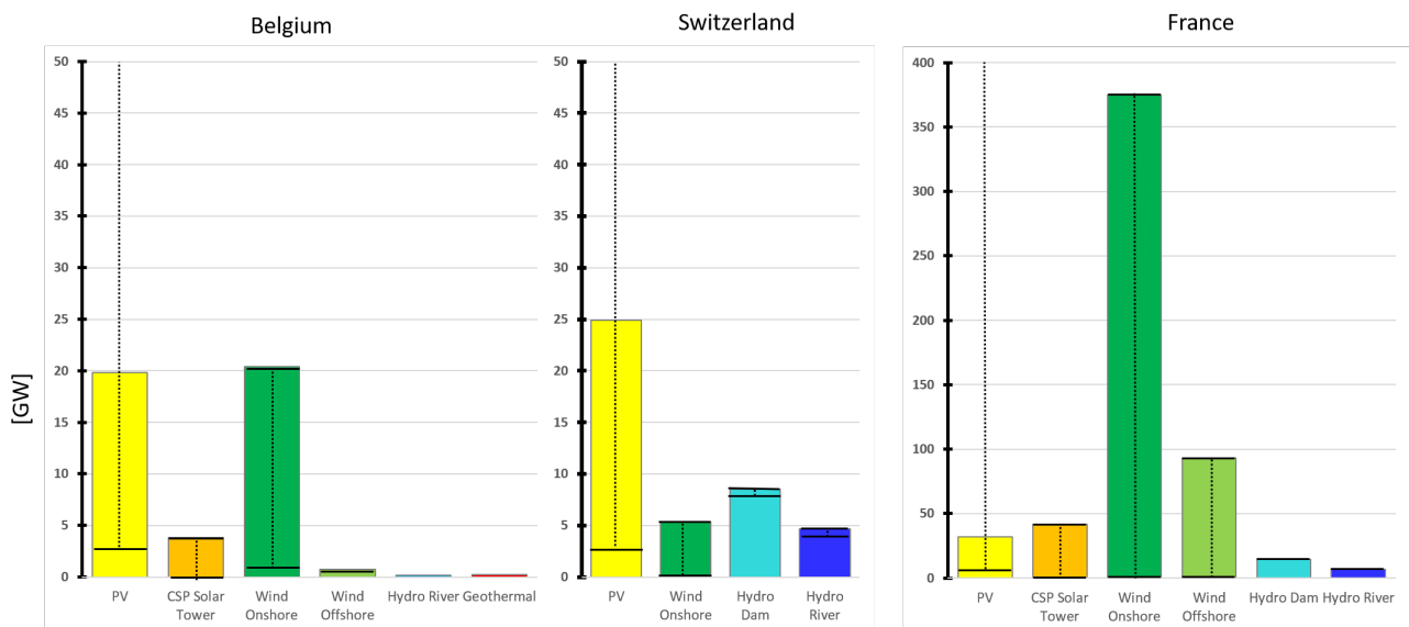
Figure D.1: RES Assets of the 3C-system with all exchanges permitted
