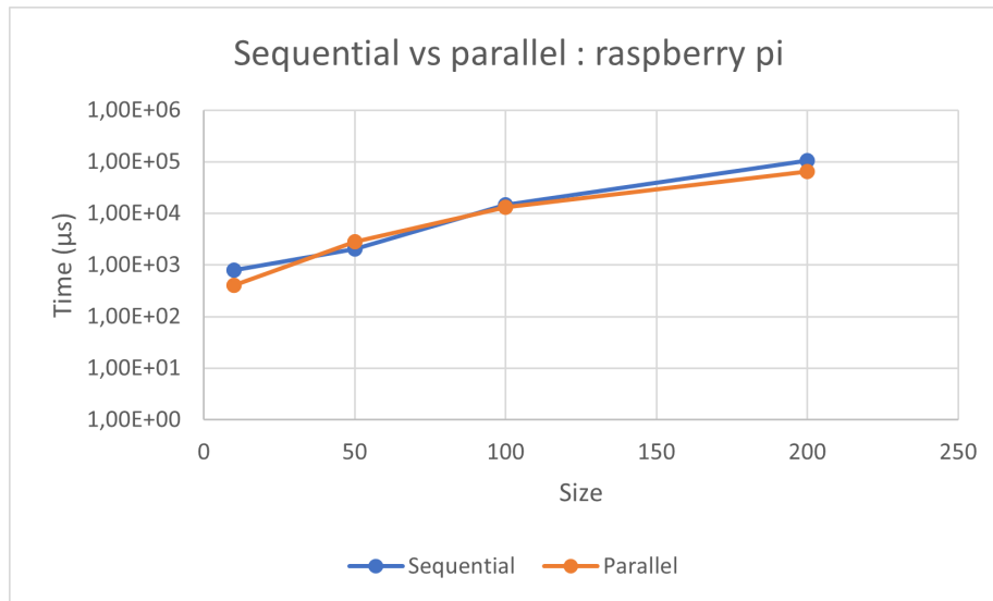
Figure 6.17: Comparing ErlBlas sequential and parallel implementations on multiplication for raspberry pi
