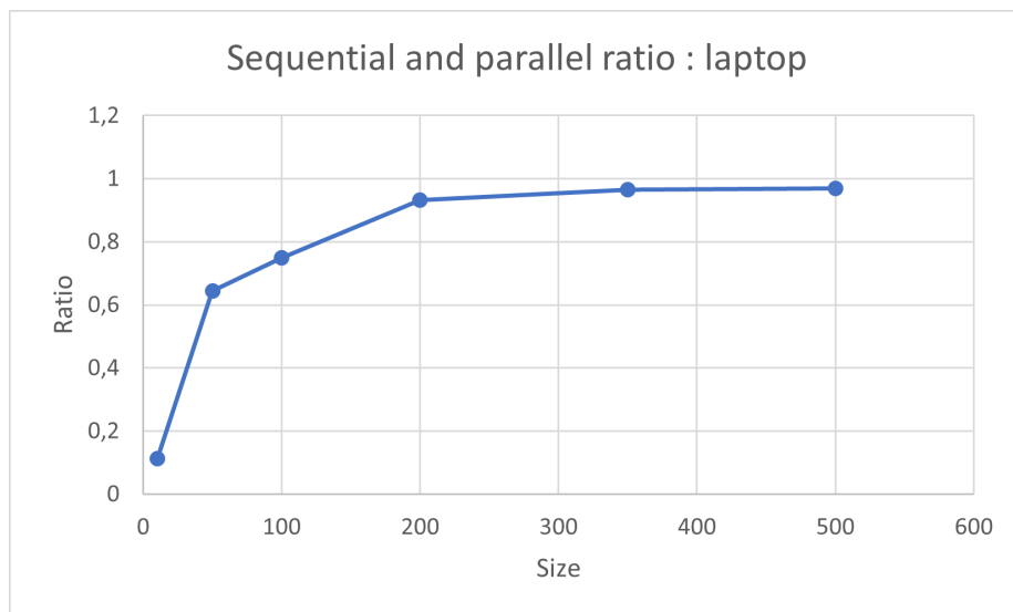
Figure 6.22: Ratio ErlBlas of sequential and parallel implementations on addition for laptop
