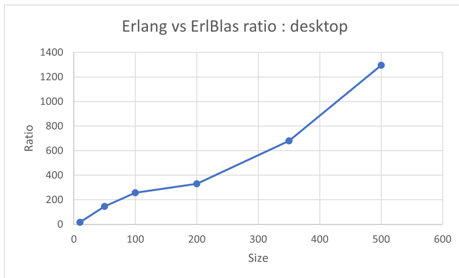
Figure 6.8: Ratio of single core pure Erlang and multicore ErlBlas on multiplication for desktop
