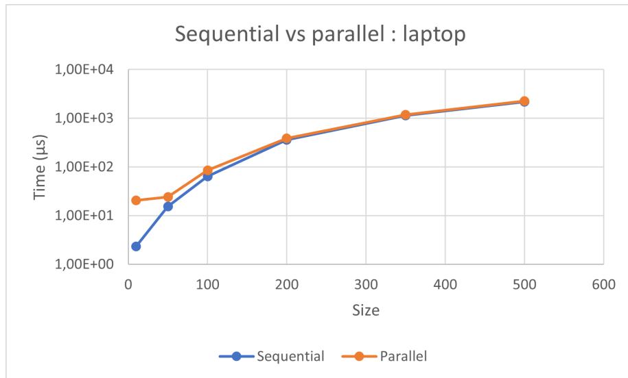
Figure 6.21: Comparing ErlBlas sequential and parallel implementations on addition for laptop
