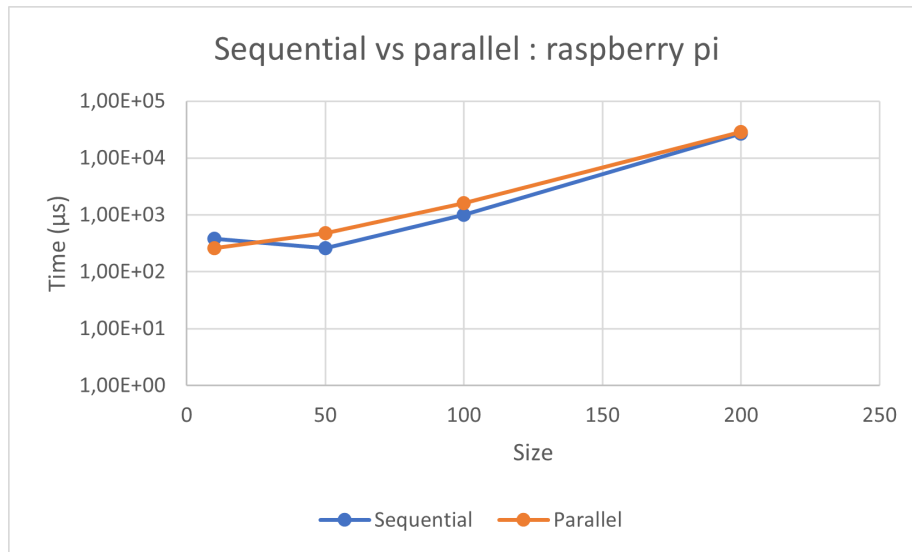
Figure 6.23: Comparing ErlBlas sequential and parallel implementations on addition for raspberry pi
