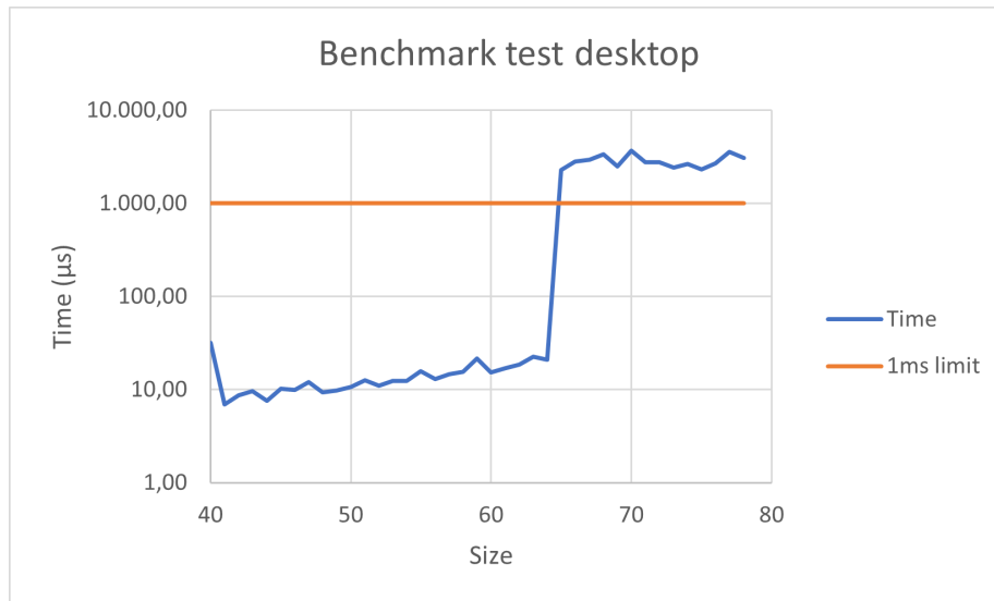
Figure 6.26: Running times for multiplication of pure C on different sizes on desktop
