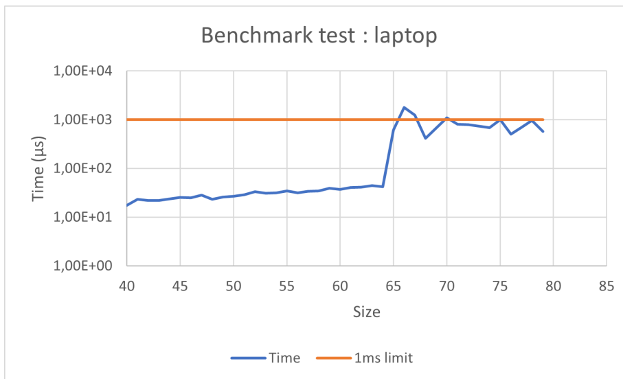
Figure 6.27: Running times for multiplication of pure C on different sizes on laptop
