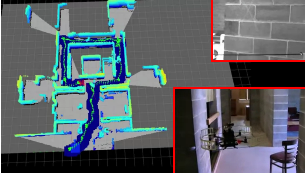
Figure 2.13: Map build and Vehicle used by V. Kumar et al. (vehicle sold by Ascending Technologies, GmbH) [139][140]
