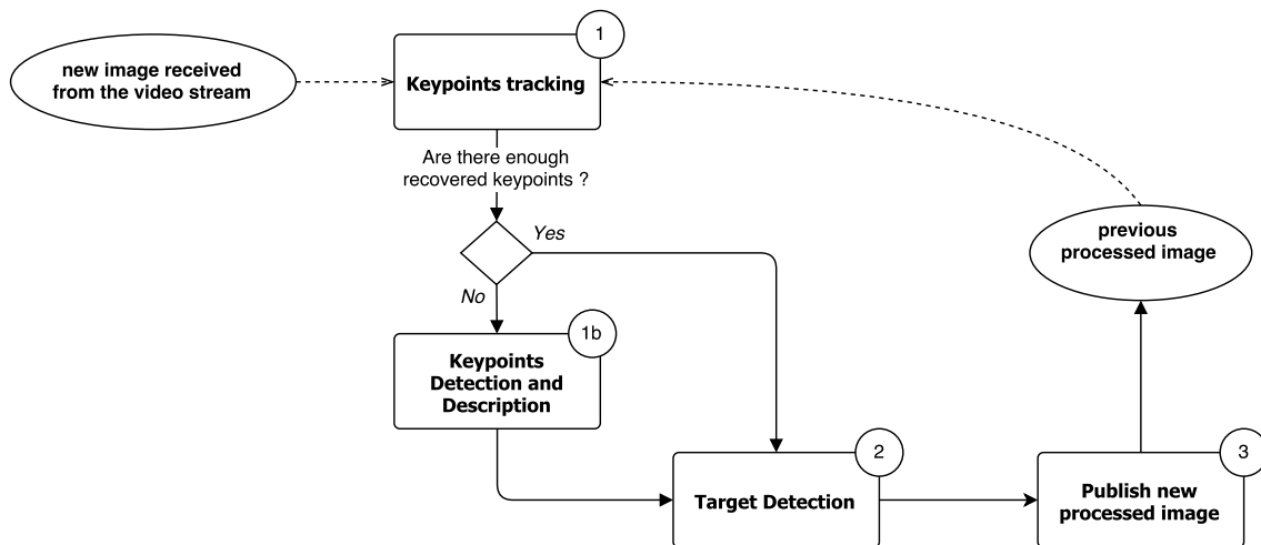
Figure 4.13: Keypoints extraction procedure
