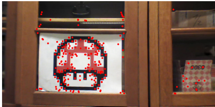
Figure 4.9: Keypoints detection (with SIFT). The keypoints (in red) are superposed on the image in the 2D Viewer node.
