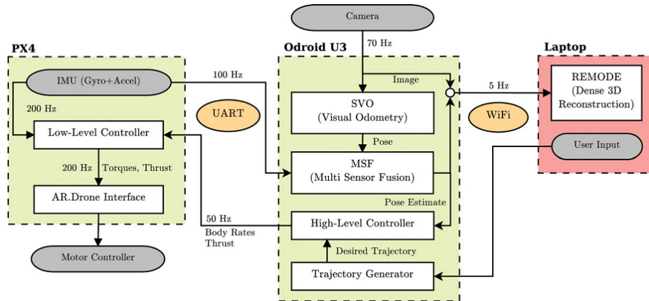
Figure 2.11: Hardware configuration used in [103]
