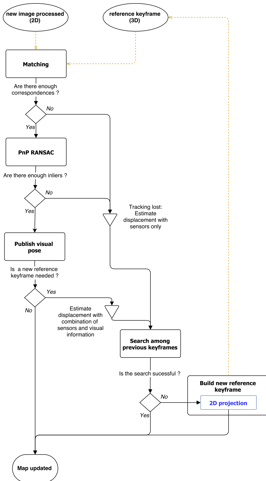
Figure 4.21: Visual pose estimation and mapping decision tree (in blue: the provisional perspective projection (2D simplification), see Figure 4.25. )
