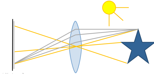
Figure 4.5: Simplified 2D lens camera projection [157]
