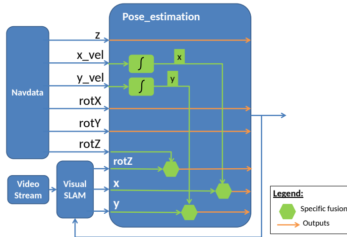
Figure 4.26: Summary of the inputs and outputs of the Pose_estimation node
