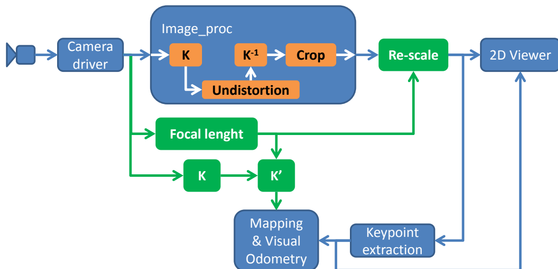
Figure 4.6: Insertion of the undistortion stage in the general image pipeline scheme
