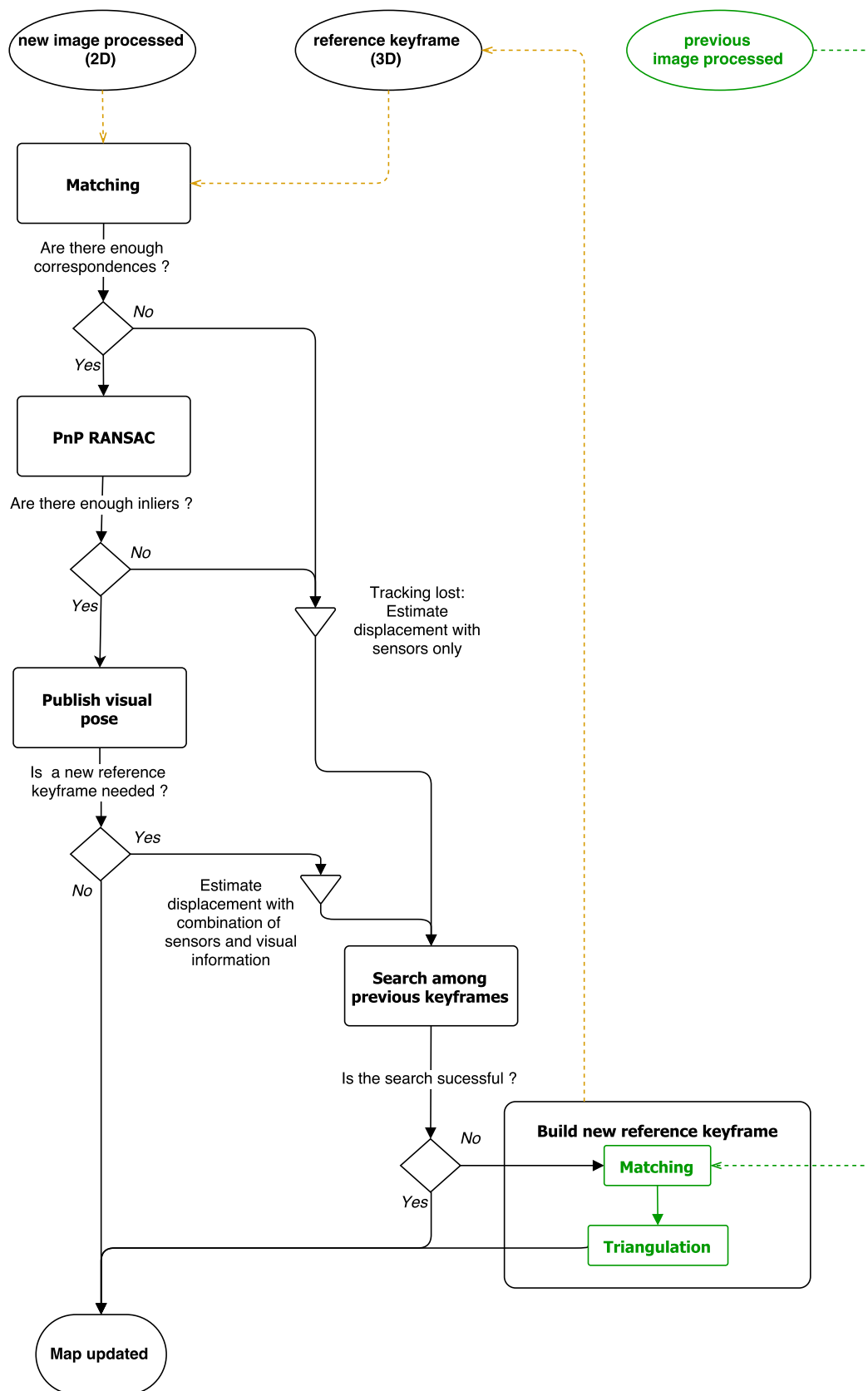
Figure 4.25: Visual pose estimation and mapping decision tree with missing blocks for 3D mapping (in green)
