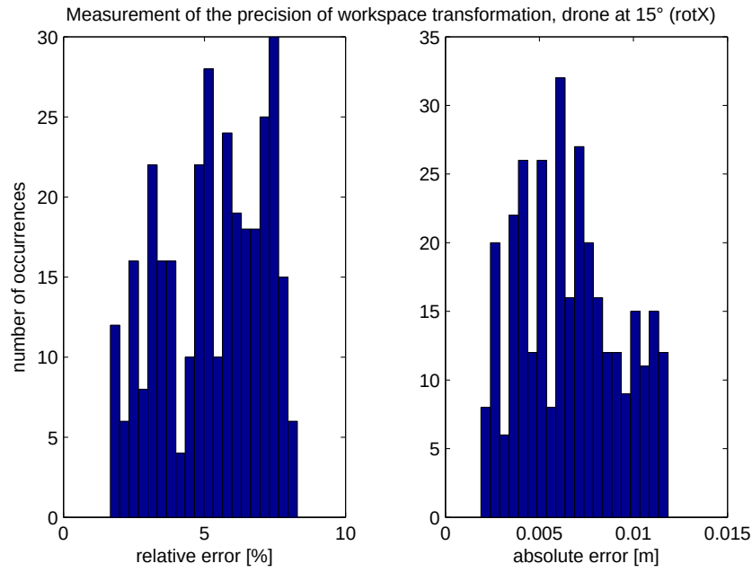
Figure C.2: Measurement of the precision of the perspective projection with the drone inclined at 15^\circ
