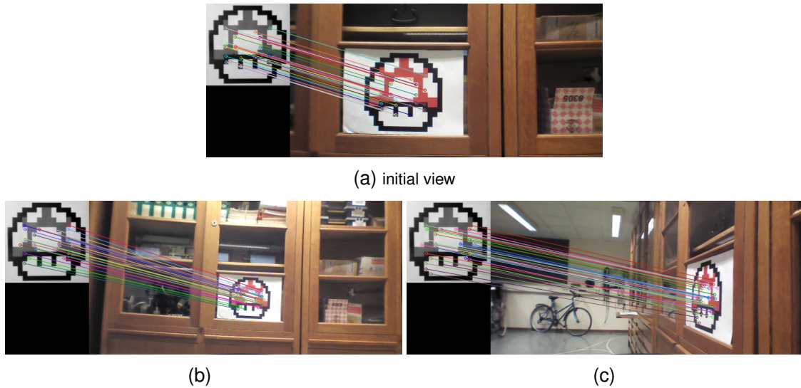
Figure 4.12: Keypoints tracking with important perspective distortions: the initial view (a) is processed with keypoints detection, keypoints tracking is used across several pictures until views (b) or (c)
