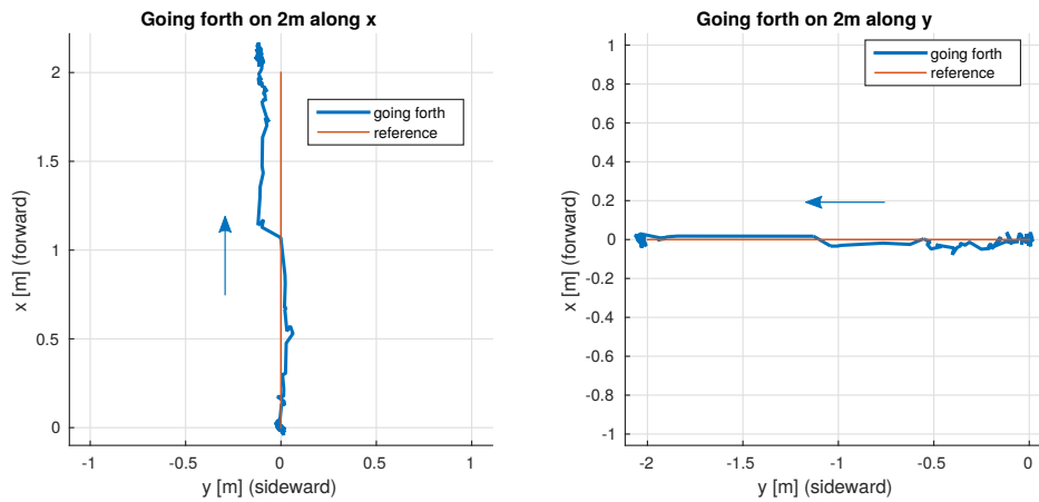
Figure 5.2: Measurement of the precision of the visual pose estimation for a pure translational displacement in the x direction (a); and for a pure translational displacement in the y direction (b)
