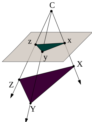
Figure 4.18: P3P Problem:
