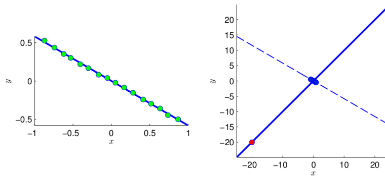
Figure 4.19: Simple example of the effect of an outlier (in red) on a line interpolation with the least square method and without RANSAC (from [168])
