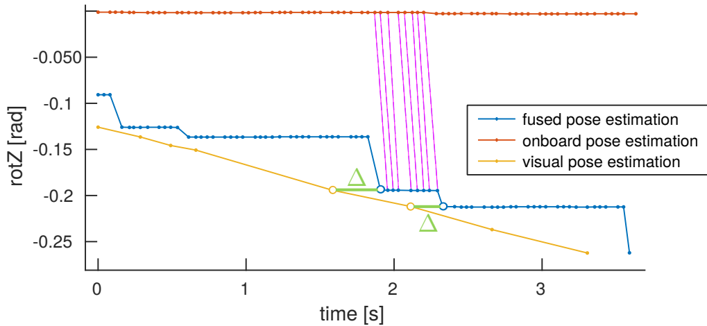
Figure 4.29: Effect of the re-calibration of the navdata pose estimation with the SLAM pose estimation. MATLAB® post-edited experiment results.
