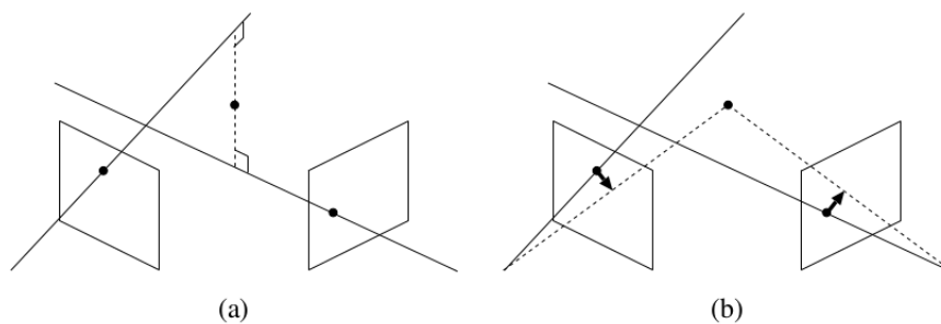
Figure 4.24: Triangulation: (a) midpoint method, (b) optimal correction [173]
