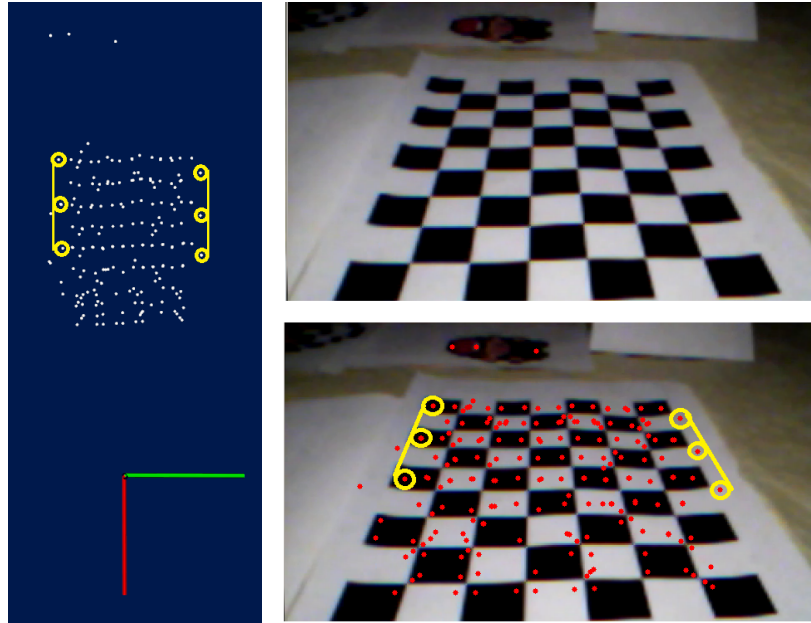
Figure 4.23: Illustration of the perspective transformation for extreme angles: the rectangular pattern (a checkerboard), which appears like a trapeze on the image, is printed correctly in the map (the red dots are the detected keypoints, the yellow lines were added to highlight the (non-)parallelism of the edges of the pattern).
