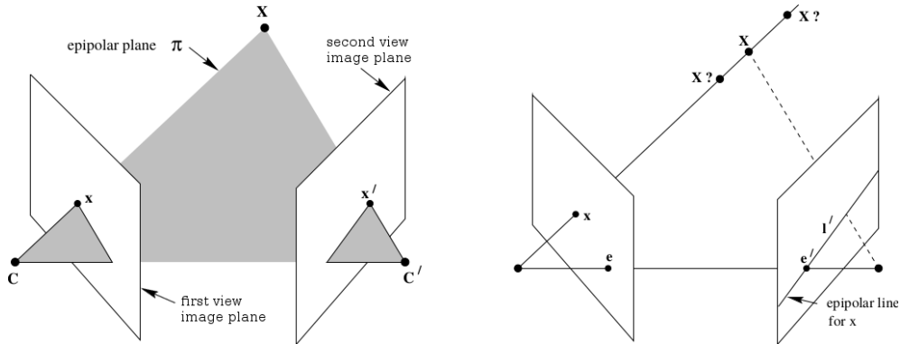
Figure 4.17: Epipolar constraint (from [166] on p.240)
