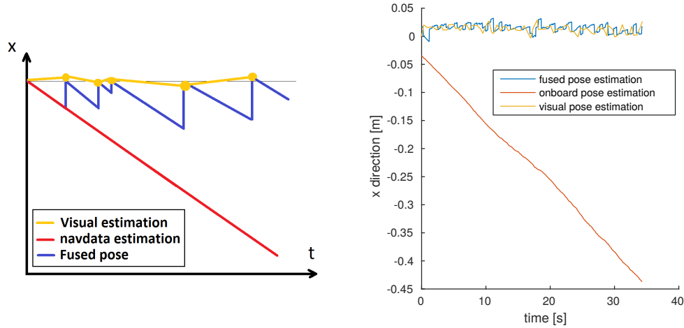
Figure 4.28: Effect of the re-calibration of the navdata pose estimation with the SLAM pose estimation. (a) Hand-drawn expected behaviour; (b) Measurement when the drone is kept static.
