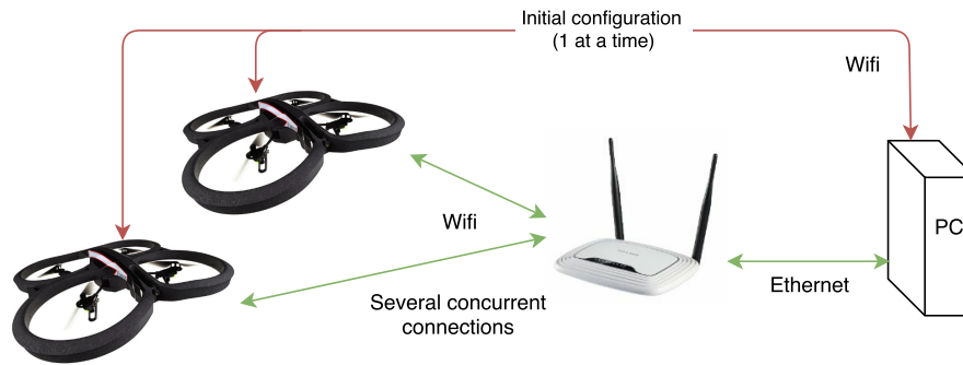
Figure 3.4: Multi-drone development platform with Parrot AR.Drone 2.0
