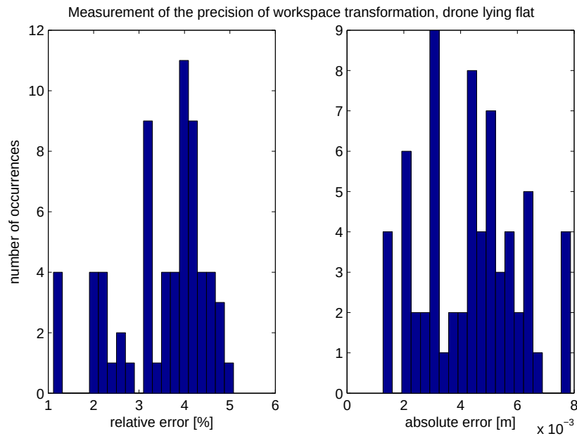
Figure C.1: Measurement of the precision of the perspective projection with the drone lying flat
