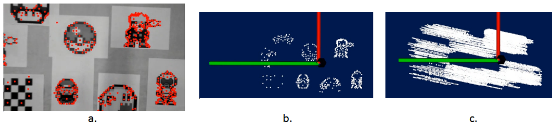
Figure B.1: Effect of the drift for the keypoints mapping if only the integration of on-board measurement is used. The drone is kept static, no SLAM is used (each new image keypoints are mapped). (a) keypoints superimposed to what the drone sees (b) initial keyframe put in the map (c) after a few seconds, all added keyframe superimpose in the map in an odd fashion
