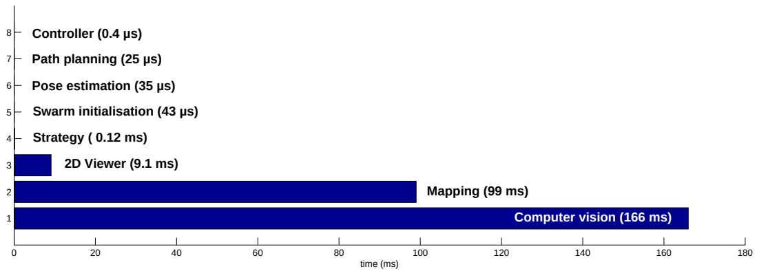
Figure 5.11: Code execution timings
