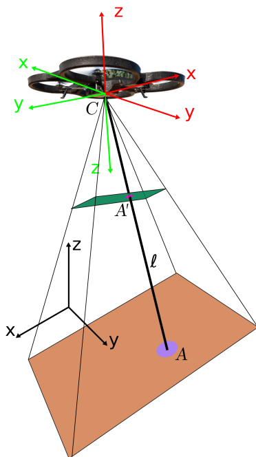
Figure 4.22: Summary of all coordinate systems:
