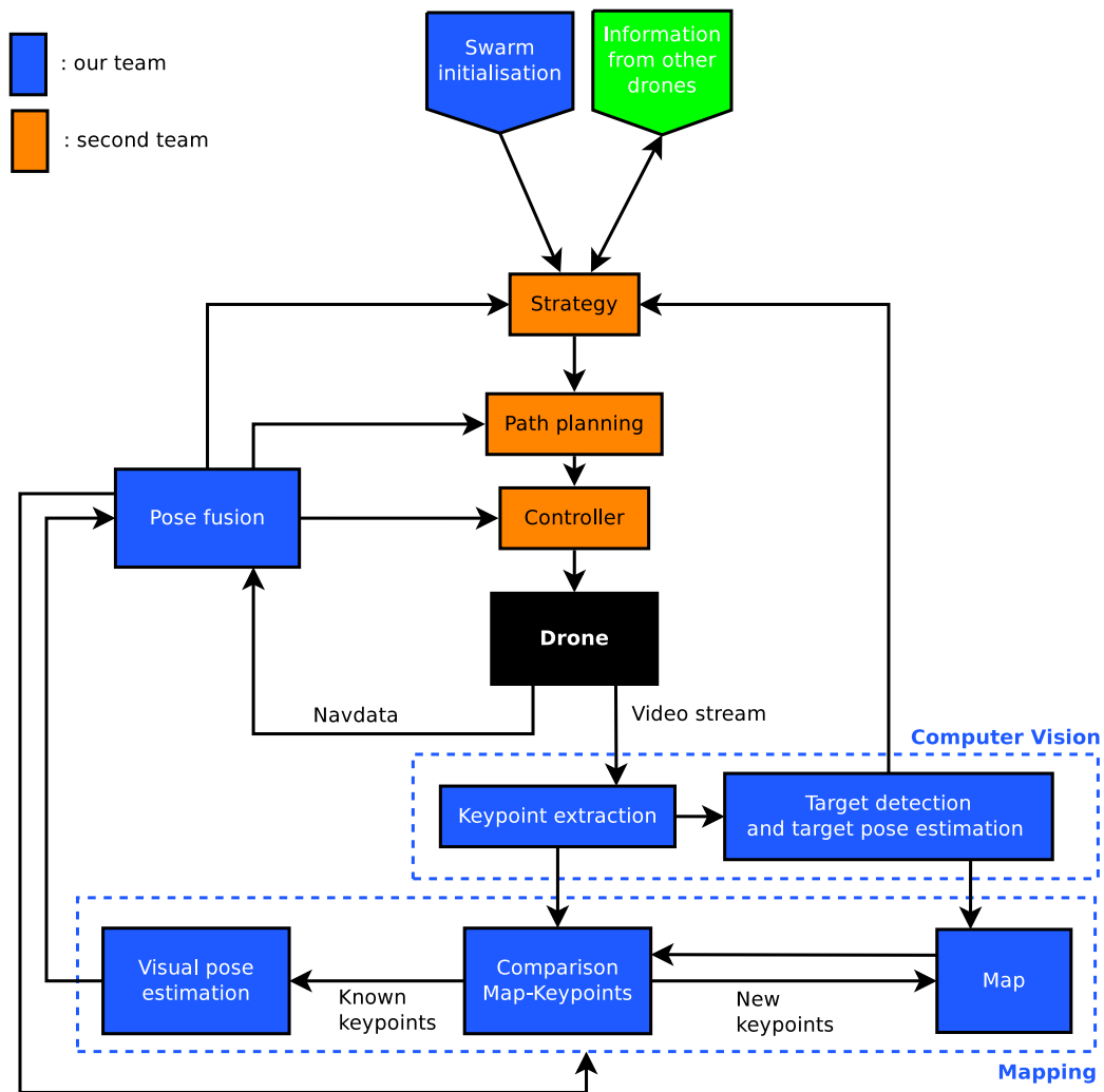
Figure 3.7: The code architecture imagined by our two teams of students
