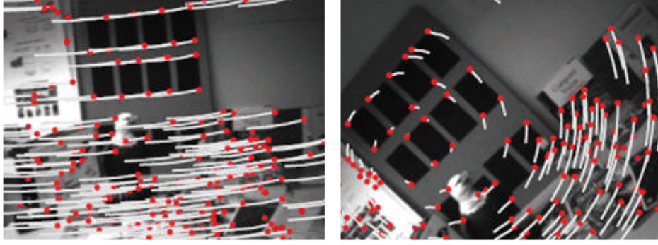
Figure 4.11: Tracking example [162]
