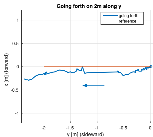
Figure 5.4: Measurement of the precision of the visual pose estimation for a pure translational displacement in a cluttered environment
