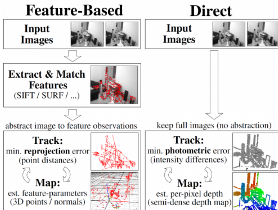
Figure 4.1: LSD-SLAM: Difference to keypoint-based methods [154]
