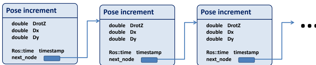
Figure 4.27: Example of a queue for the pose estimation increments that must be added when a visual correction is done.
