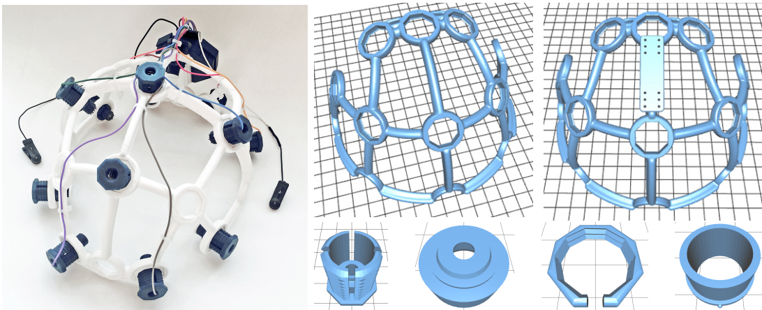
Figure 3.3: Ultracortex Mark III helmet from OpenBCI [42]
