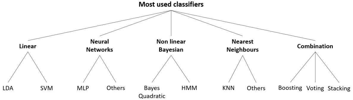
Figure 2.6: Most common classification algorithms used with BMIs [32]
