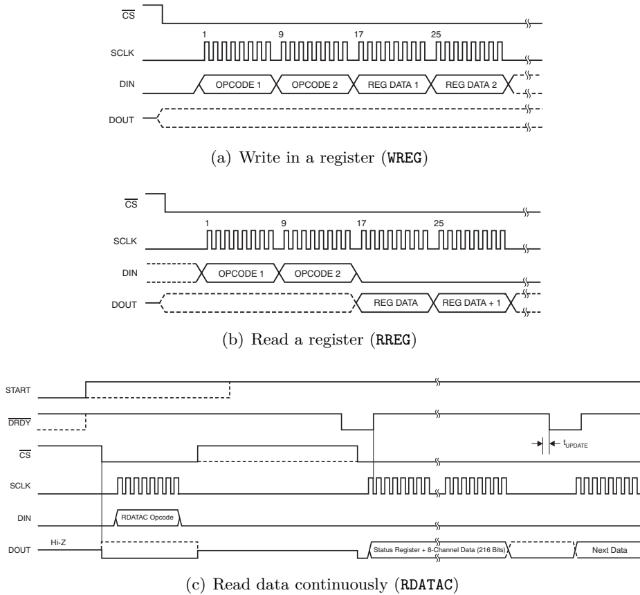
Figure 4.3: Illustrations of several communications with the ADS [27]
