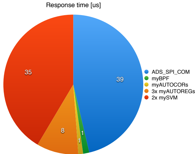
Figure 5.8: Response time repartition of the FPGA implementation
