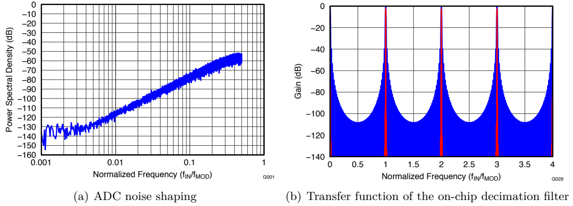
Figure 3.5: Illustrations of some properties of the ADS1299 [27]
