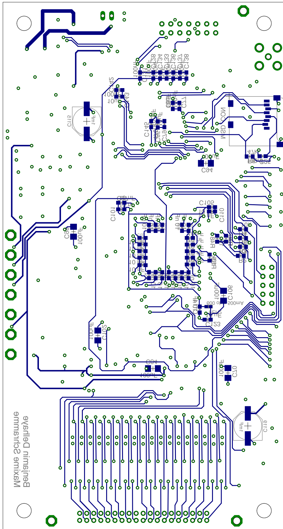
Figure A.11: Board - Layer 4 - Bottom
