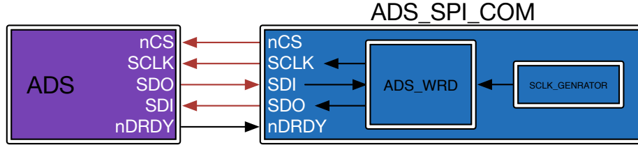
Figure 4.4: Main connections between the ADS and the module ADS_SPI_COM
