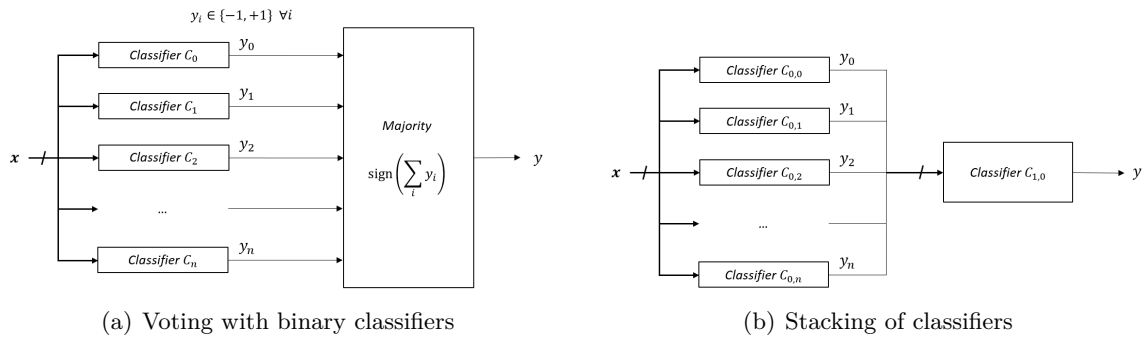
Figure 2.11: Two possible combinations of classifiers
