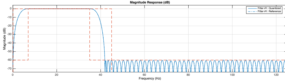
Figure 4.9: Magnitude response of the FIR BPF
