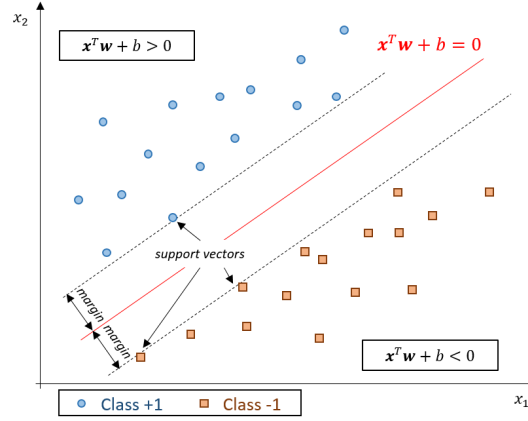
Figure 2.8: SVM classification of two classes using two features
