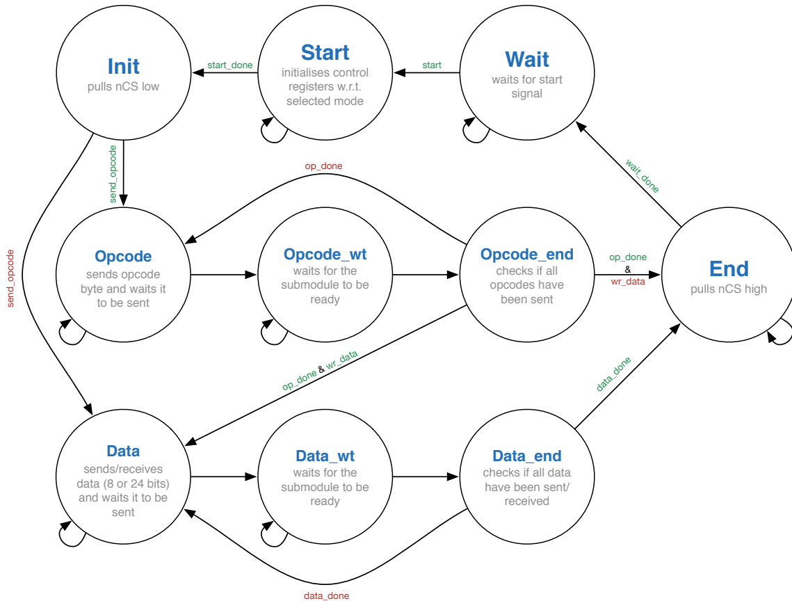
Figure 4.5: FSM of the module ADS_SPI_COM
