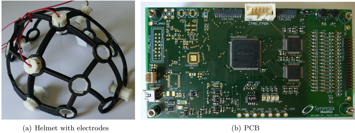
Figure 3.6: Illustrations of the experimentation system
