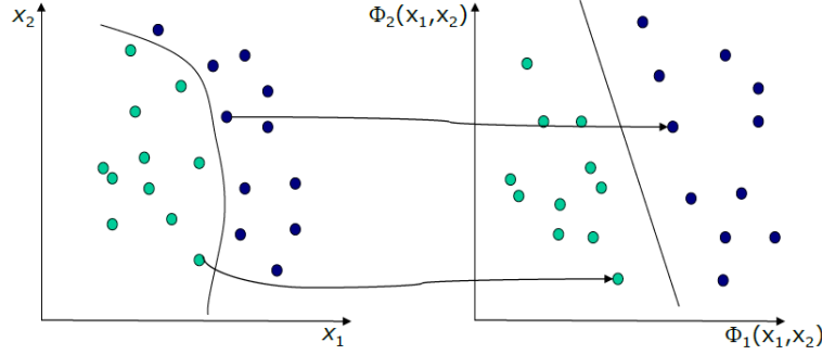
Figure 2.10: Mapping in a higher dimensional space using a function \Phi(\mathbf{x}) [1]
