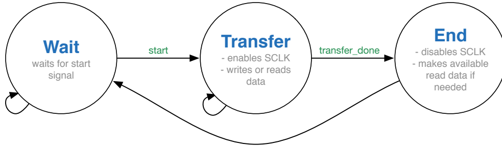
Figure 4.6: FSM of the module ADS_WRD
