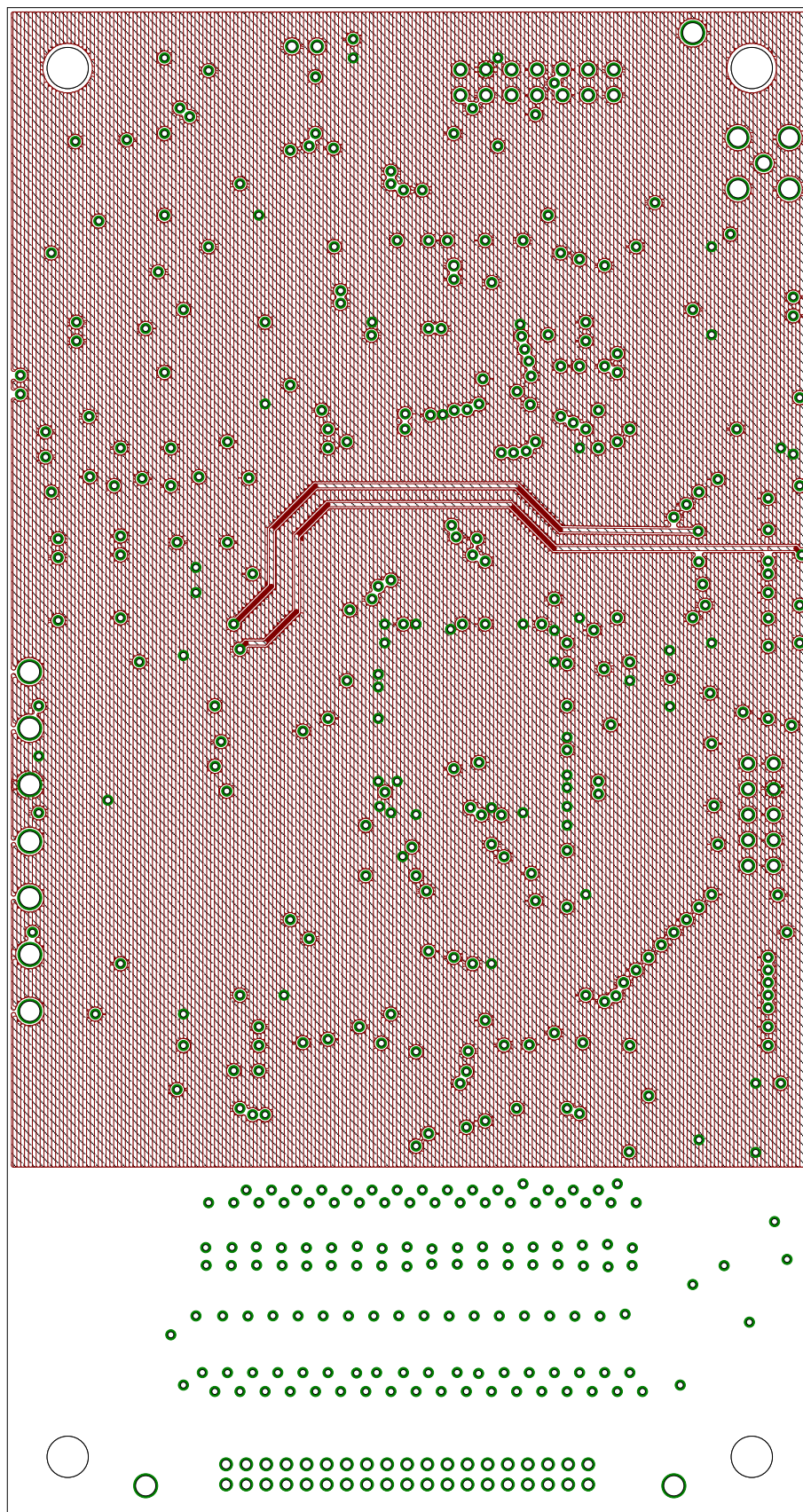
Figure A.10: Board - Layer 3 - DVDD
