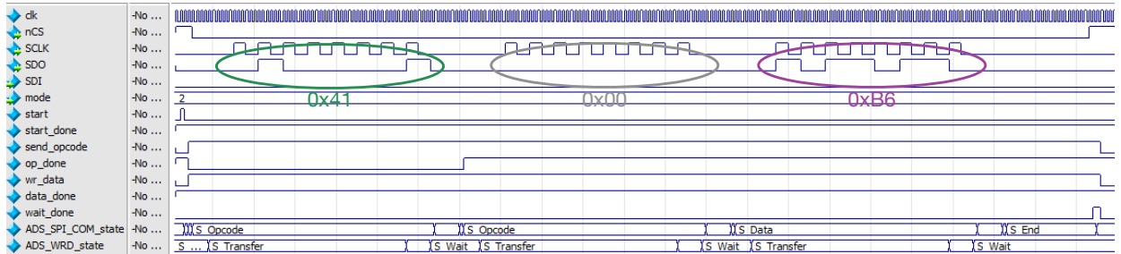
Figure 4.7: Simulation of the module ADS_SPI_COM on MODELSIM
