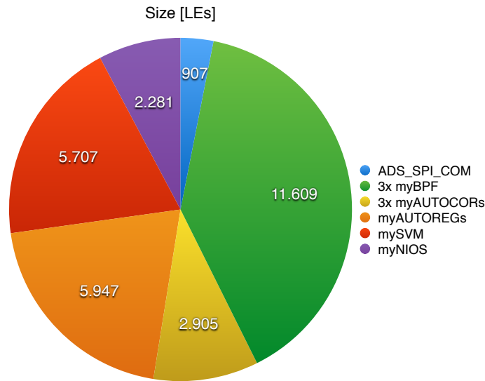
Figure 5.7: Size repartition of the FPGA implementation
