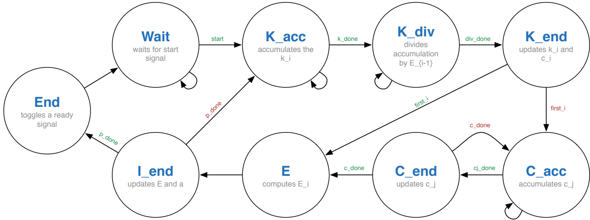
Figure 4.19: FSM of the module myAUTOREGs
