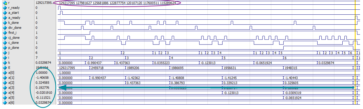
Figure 4.21: Simulation of the module myAUTOREGs on MODELSIM
