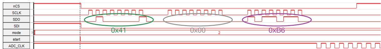
Figure 4.8: Simulation of the module ADS_SPI_COM on SIGNALTAP
