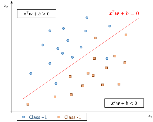
Figure 2.7: Linear classification of two classes using two features
