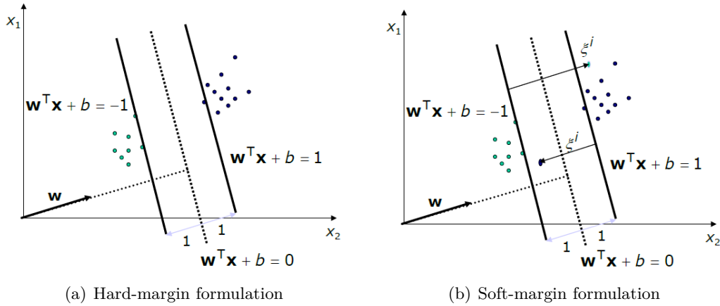
Figure 2.9: Two SVM formulations [1]
