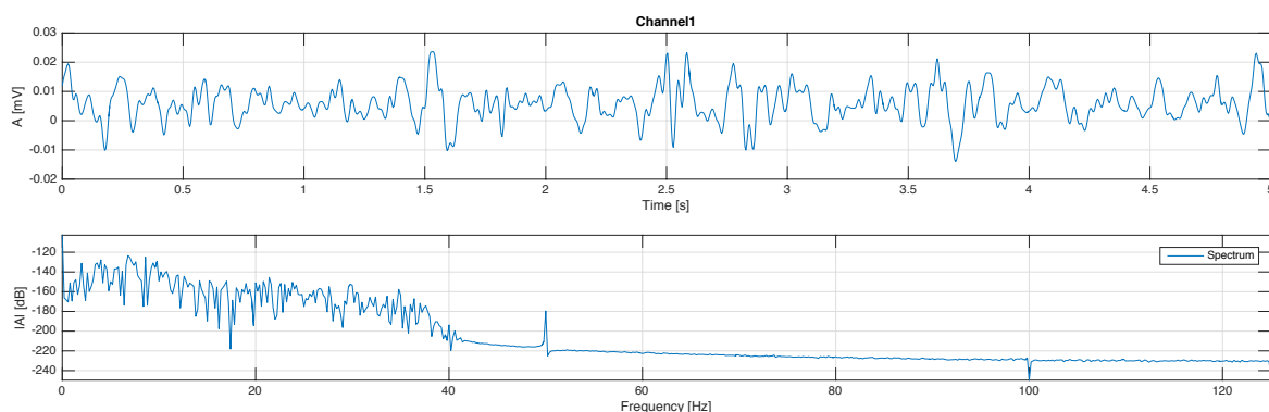
Figure 5.6: Typical acquisition with the experimentation system
