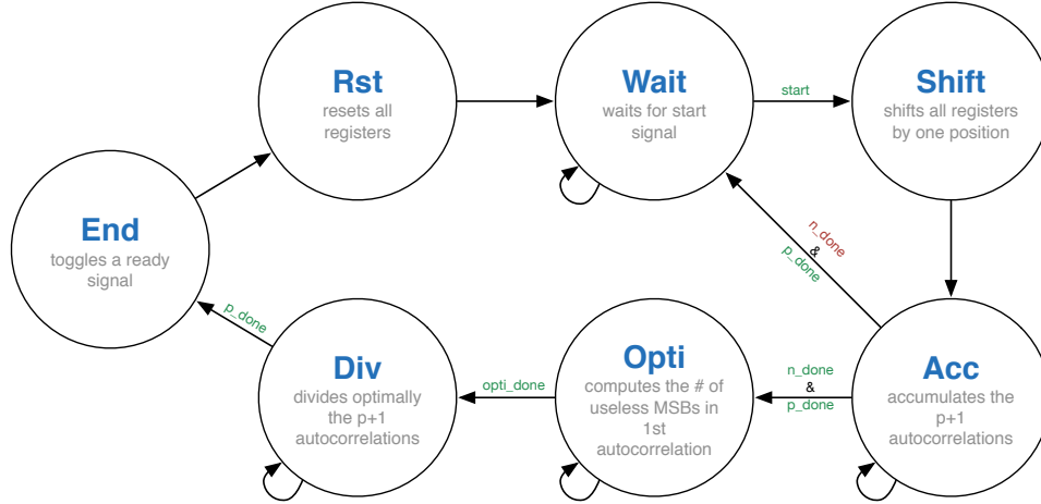
Figure 4.14: FSM of the module myAUTOCORs
