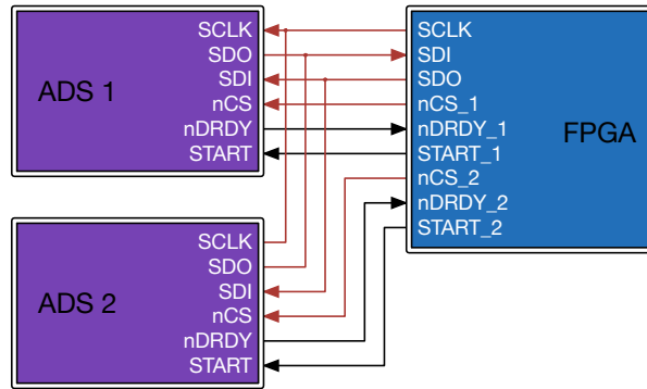
Figure 4.2: Main connections between FPGA and ADSs
