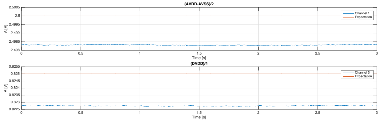
Figure 5.2: Supply test on the ADS
