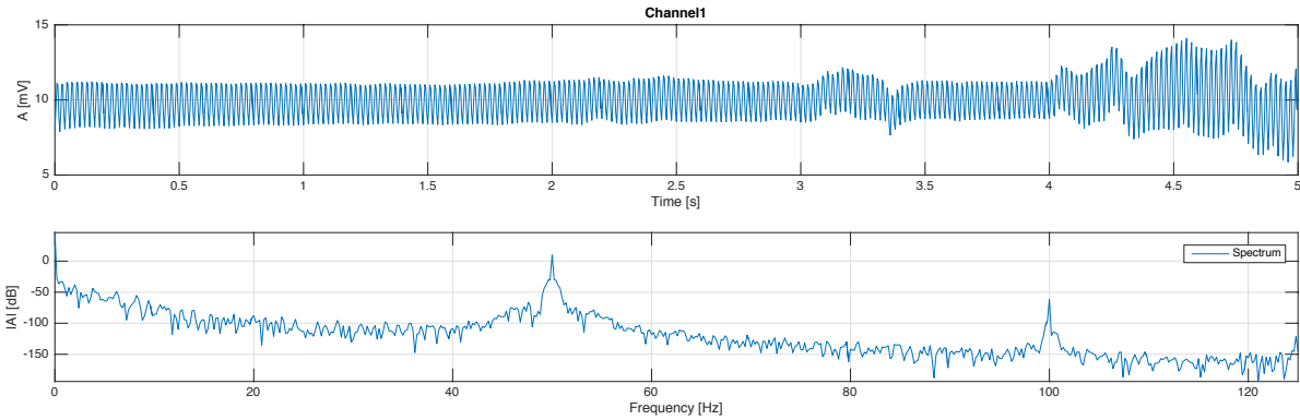
Figure 5.4: EEG acquisition without bias
