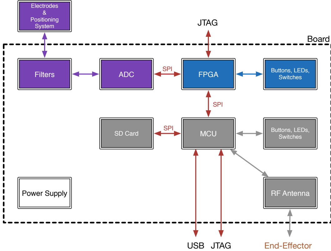
Figure 3.2: Global system overview
