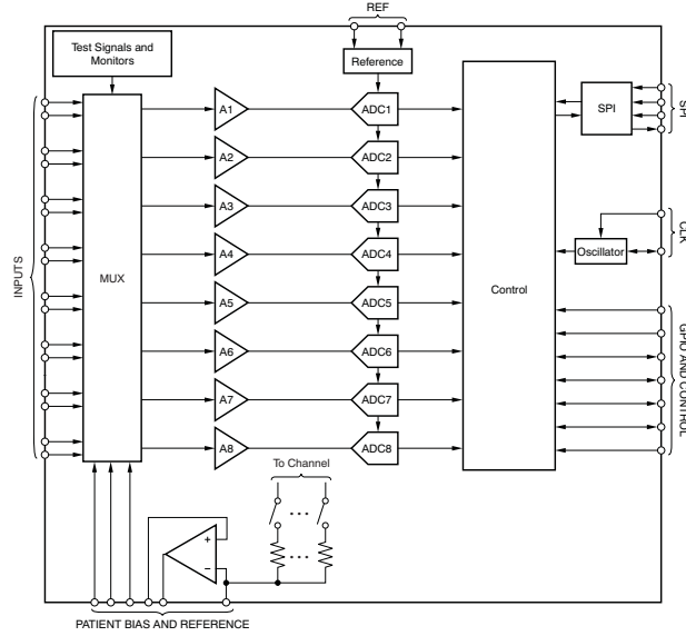
Figure 3.4: Simplified scheme for the ADS1299 [27]
