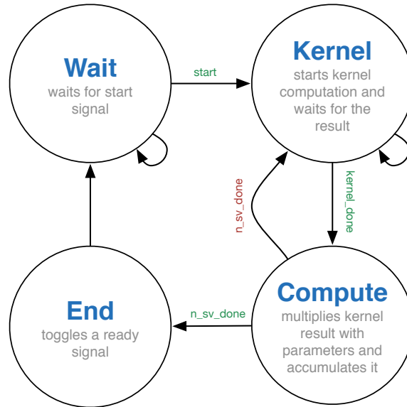
Figure 4.23: FSM of the module mySVM
