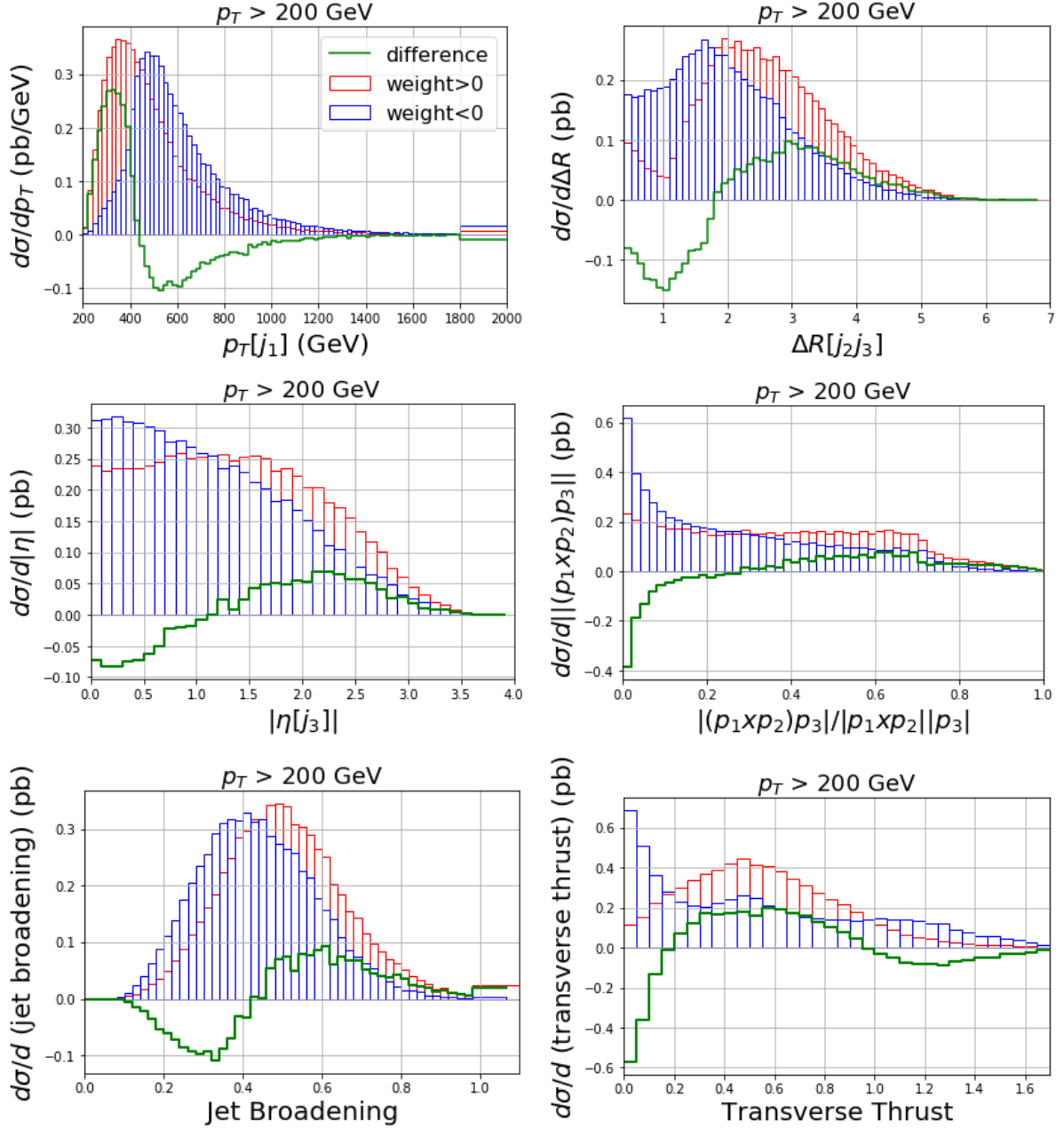
FIGURE 2.3.1. Examples of differential distributions that better divide the interference events, for p_T > 200 GeV; respectively, the transverse momentum of the 1 st jet, the angular distance between the 2 nd and 3 rd jets, the pseudorapidity of the 3 rd jet, the triple product of the momenta of the three jets, the jet broadening and the transverse thrust. The red line represents the differential cross-section contribution by the positive-weighted events, the blue one the income from negative-weighted ones; their difference, the green plot, is the differential cross-section distribution for the interference. All of them show one or more sign flips in the differential cross-section trend, for certain values of the observable. The relative binnings are described in Table 2.4; for the transverse momentum and the jet broadening, the last bin is not entirely shown
