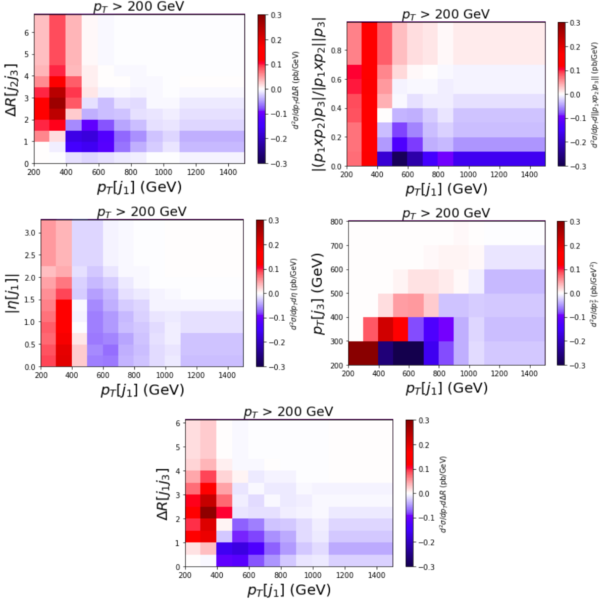
FIGURE 2.3.3. Examples of double differential distributions, for p_T > 200 GeV; all three involve the transverse momentum of the 1 st jet, respectively vs the angular distance between the 2 nd and 3 rd jets, the normalised triple product of the three jet momenta, the pseudorapidity of the 1 st jet, the transverse momentum of the 3 rd jet and the angular distance between the 1 st and the 3 rd jets. The relative binnings are described in Table 2.4; for the transverse momenta, the last bin is not entirely displayed. The total differential cross-section for each bin is codified in the color bar besides each plot, with red shades for the positive contributions and blue shades for the negative ones. The first 2 combinations are promising ones, since it is quite easy to isolate the differently colored regions of the plane, by considering some compact ranges for the variables; this is not true for the third plot, since the sign of the cross-section does not seem to depend in a significative way on the value of |\eta[j_1]| . The last two plots suggest the signs of the event weights are related to their topology
