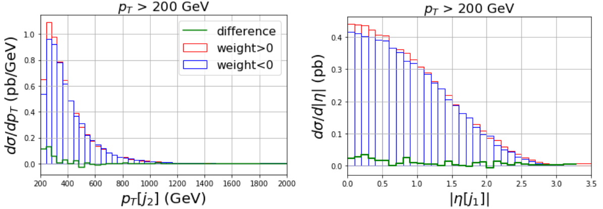
FIGURE 2.3.2. Some examples of differential distributions that do not divide the interference events, for p_T > 200 GeV; respectively, the transverse momentum of the 2^{nd} jet and the pseudorapidity of the 1^{st} jet. The red line represents the differential cross-section contribution by the positive-weighted events, the blue one the income from negative-weighted ones; their difference is the green plot. The cross-section is almost null all over the range, so that an analysis of the interference effects is not worth it. The relative binnings are described in Table 2.4; for both the distributions, the last bin is not entirely displayed
