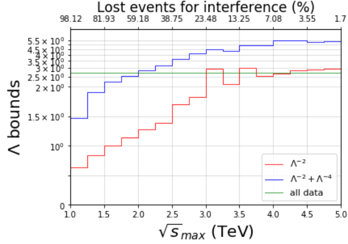
FIGURE 2.3.5. Upper bounds on \Lambda as functions of an upper cut over the center-of-mass energy, \sqrt{s} , inferred from the p_T[j_1] distribution with bins of 40 GeV, for C_G = 1 . The red line shows the bounds from the \mathcal{O}(\Lambda^{-2}) order only, while the blue one takes into account the \mathcal{O}(\Lambda^{-4}) contribution, too. The green line reports the bounds from the interference, obtained using all the events. The axis on top of the plot reports the percentage of events, in the interference sample, that get lost when imposing the corresponding cut on the energy
