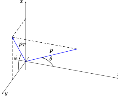
FIGURE 2.1.1. Some quantities used in jet analysis. The incoming beams travel along the z direction, while \mathbf{p} is the momentum of one outgoing jet
