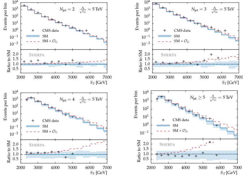
FIGURE 1.5.1. S_T distributions from CMS, in various bins of jet multiplicity N_{jets} , compared to signal and background predictions, including perturbative uncertainties 20
