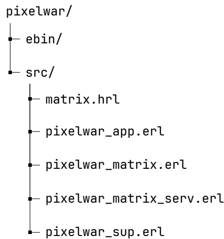
Figure 3.1: Initial file structure for section 3.2.1
