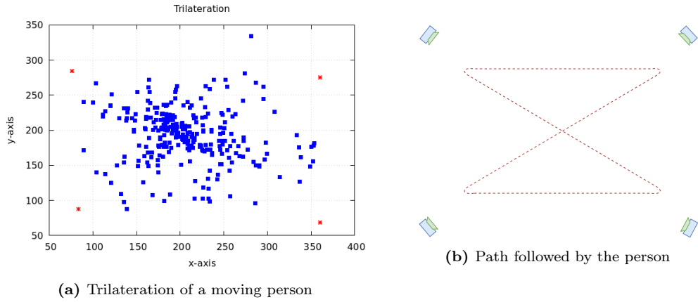
Figure 48.: Trilateration of moving person inside a room with 4 sonars. Obtained with gnuplot
