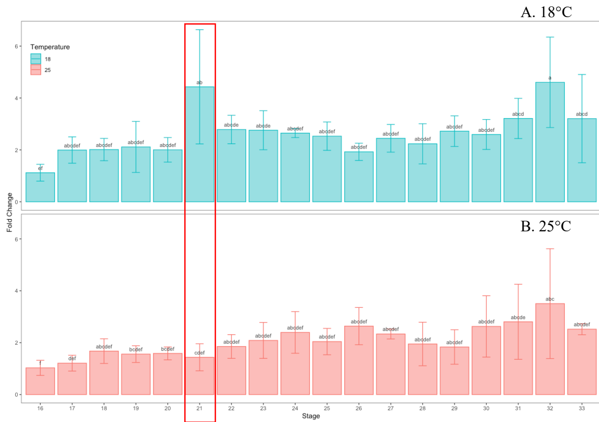
Figure 4 - Fold change of dnmt3ab during the embryo development of K. marmoratus at (A) 18°C and (B) 25°C. The interaction between the developmental stage and the temperature is not significant ( p\text{-value} = 2.42\text{e-}01 ). 18S was used as housekeeping gene. The red box represents the stage for which temperature as a significant impact on gene expression. Significant differences between stages and temperature were checked using post hoc Tukey's test.
